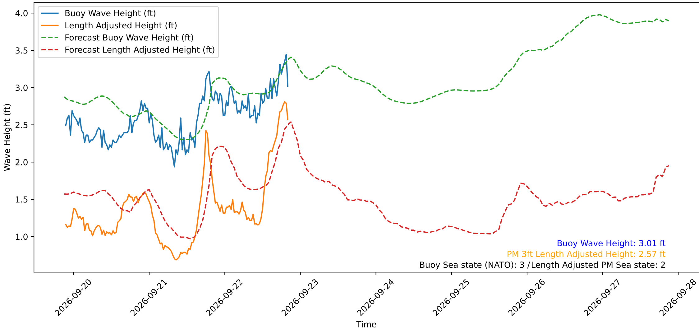
Wave Heights over Time for Green Beach at 2026-09-22 21:01:11
