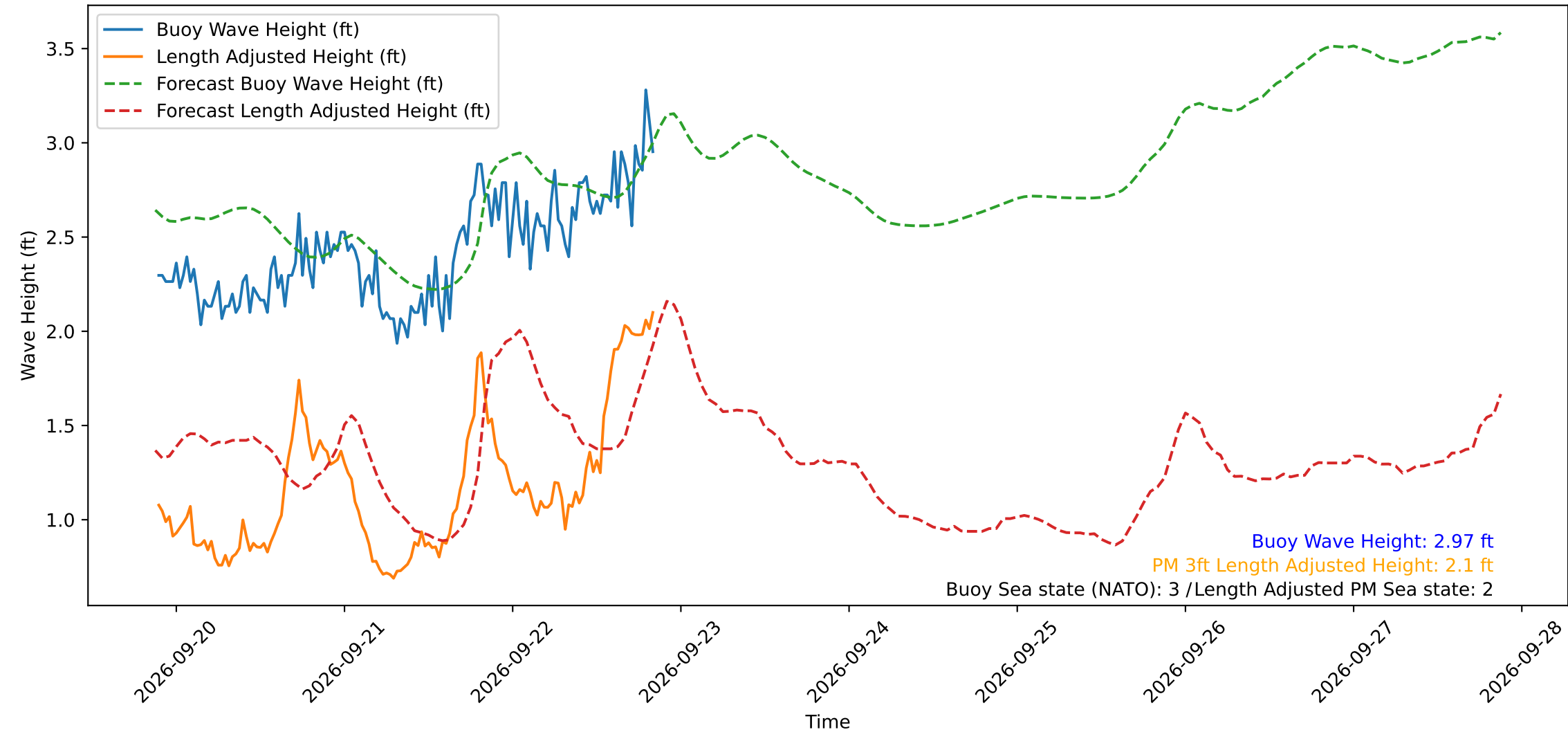
Wave Heights over Time for Red Beach at 2026-09-22 21:00:48
