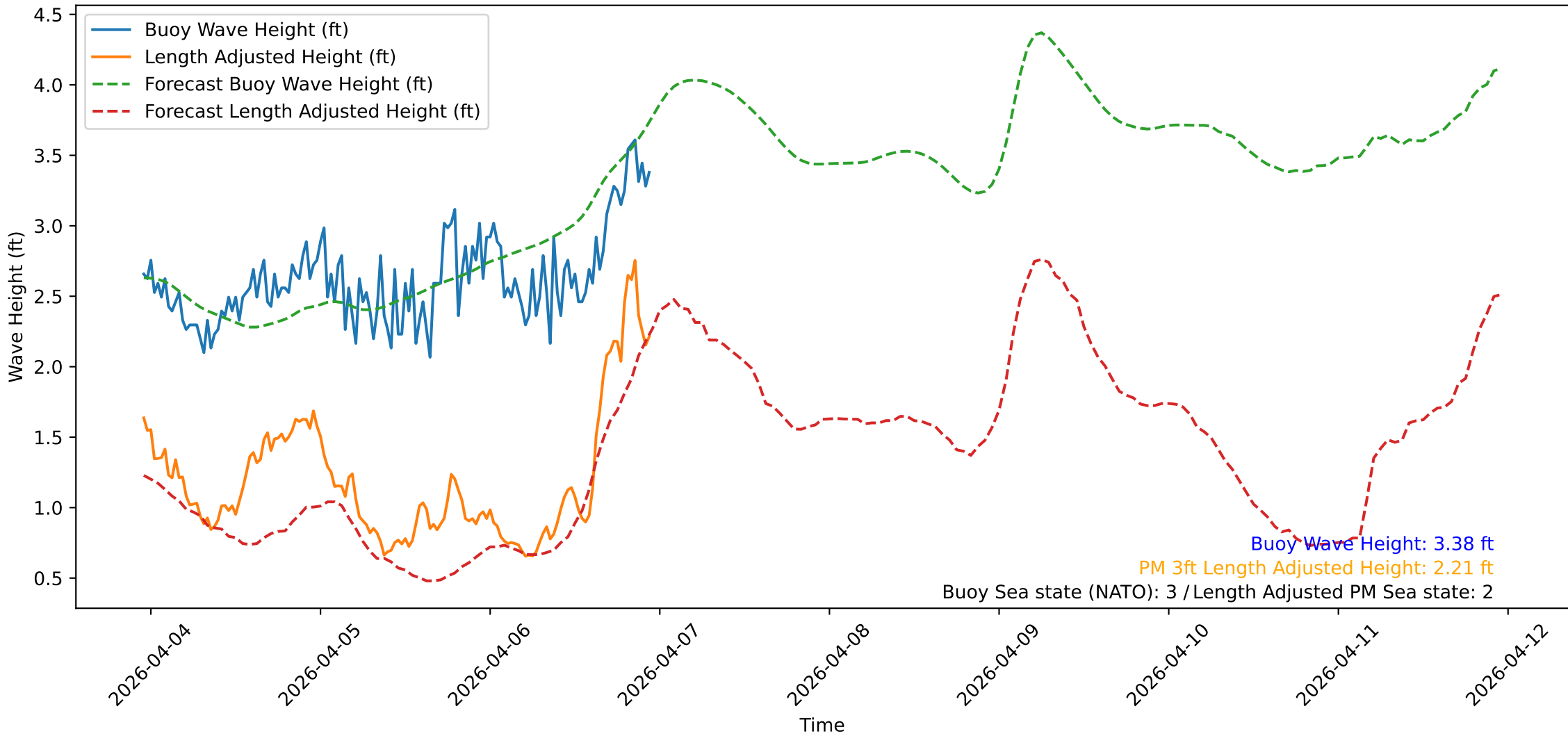
Wave Heights over Time for Oceanside Harbor at 2026-04-06 23:10:34
