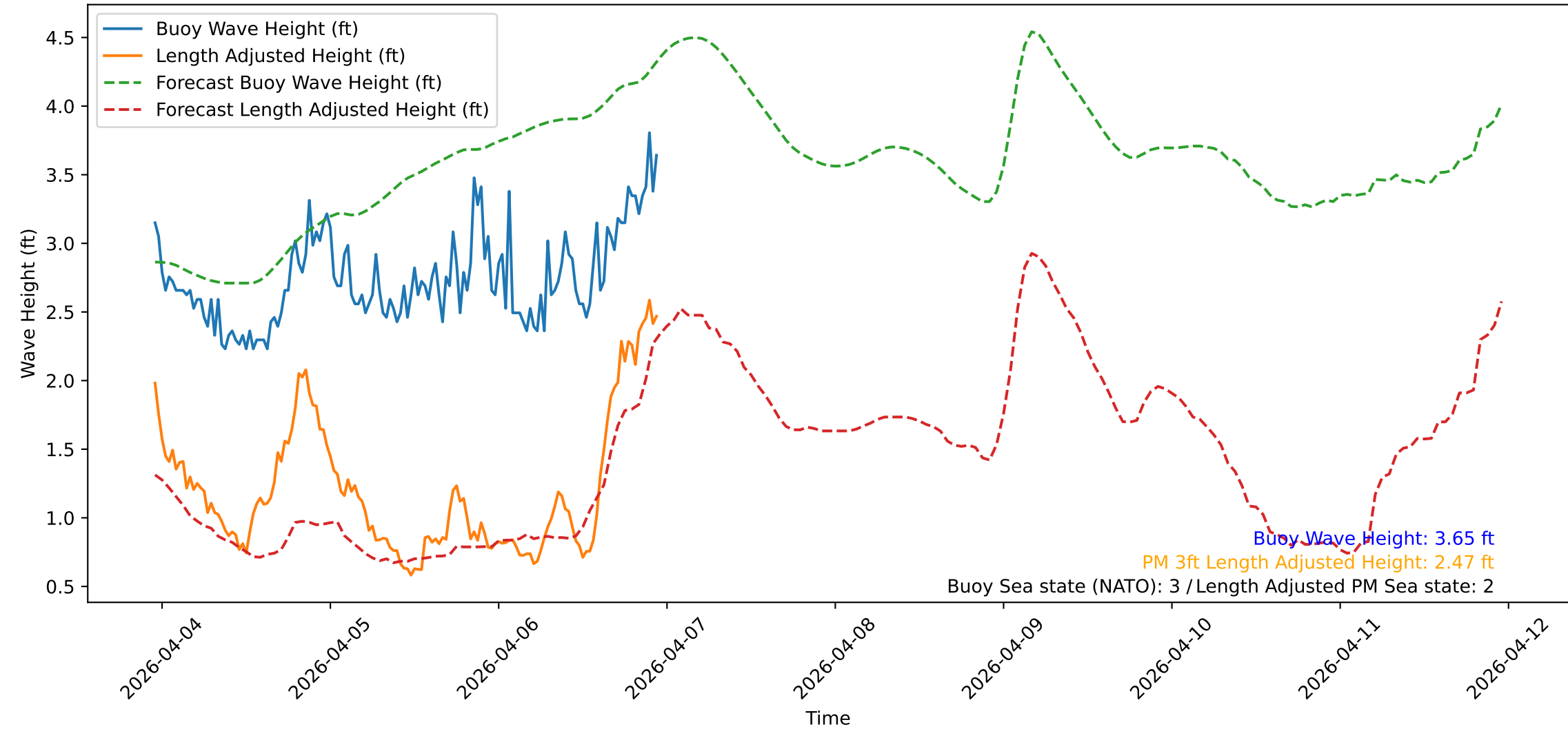
Wave Heights over Time for Green Beach at 2026-04-06 23:11:13
