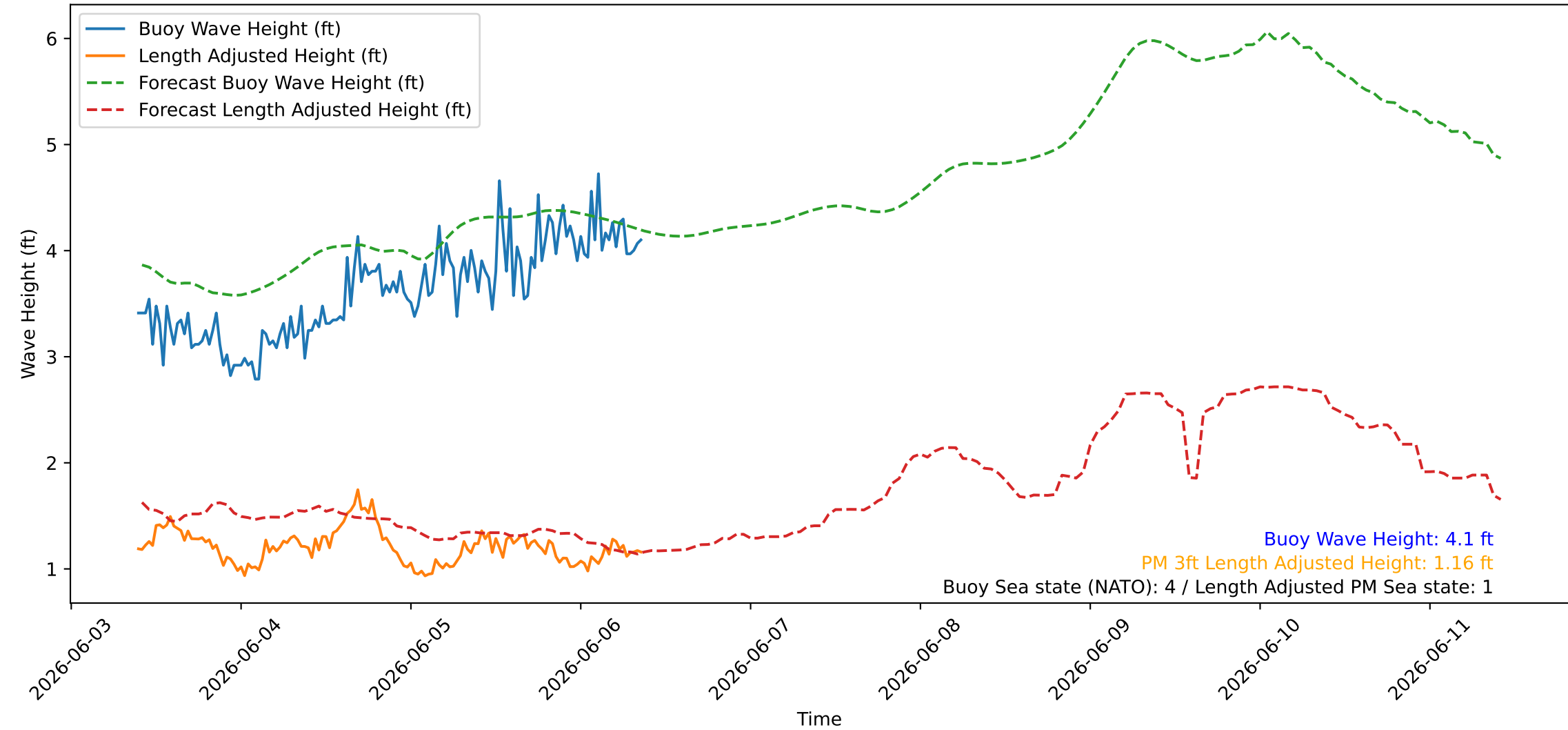
Wave Heights over Time for Green Beach at 2026-06-06 09:31:08
