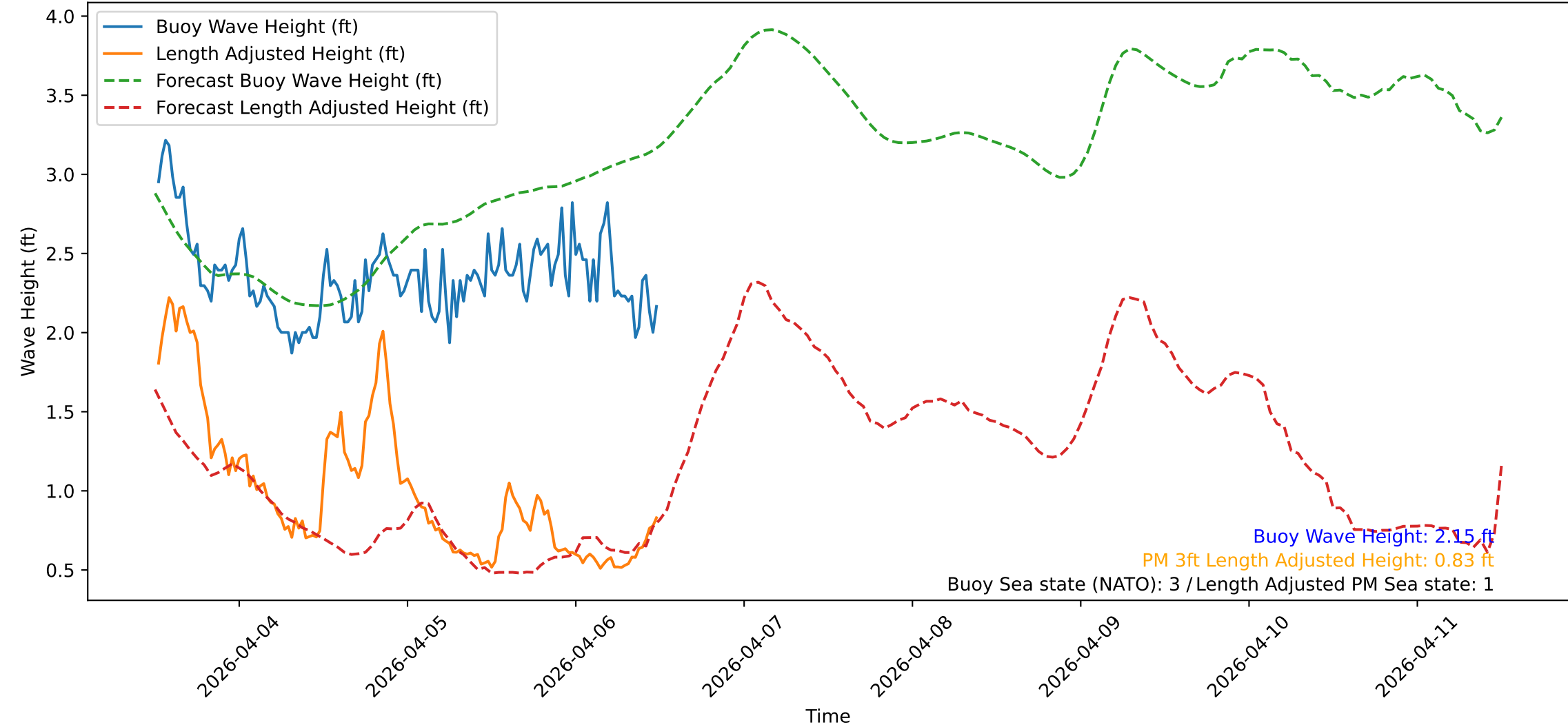
Wave Heights over Time for Red Beach at 2026-04-06 12:20:47
