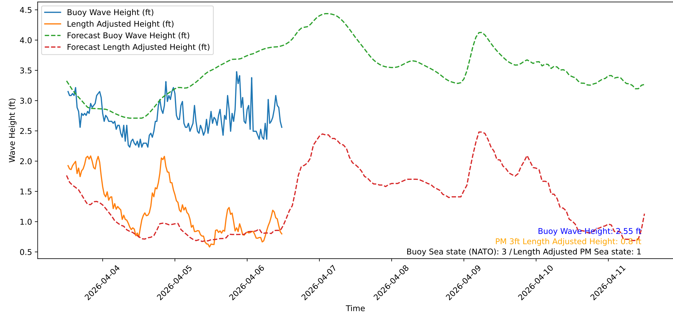
Wave Heights over Time for Green Beach at 2026-04-06 12:21:10
