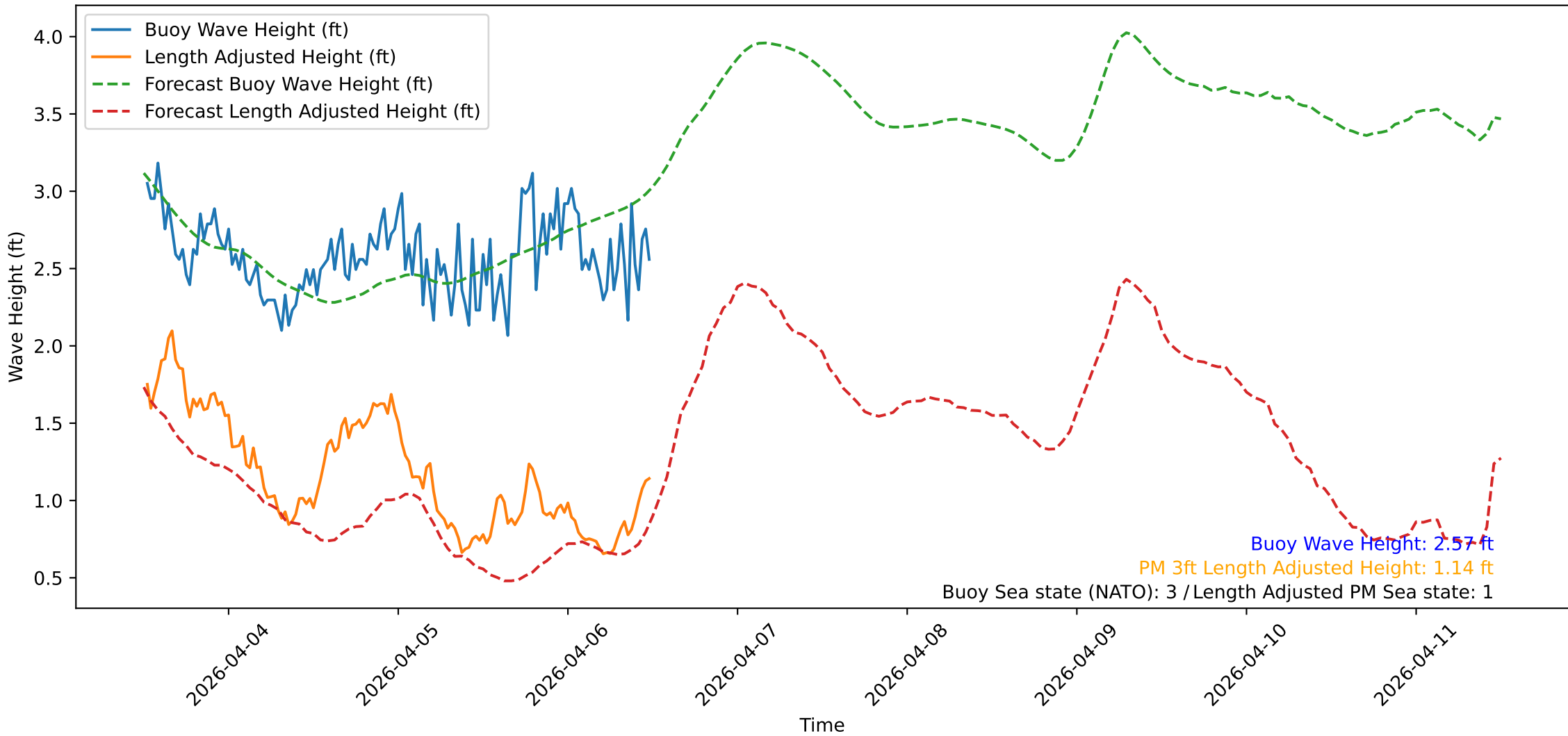
Wave Heights over Time for Oceanside Harbor at 2026-04-06 12:20:32
