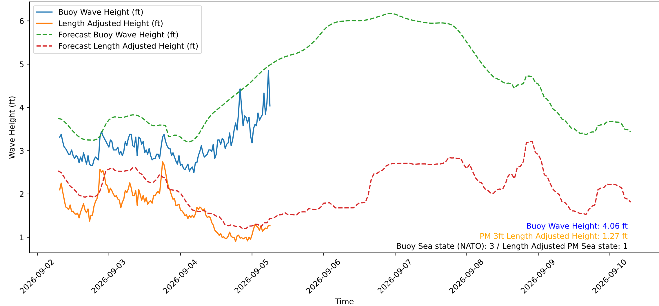
Wave Heights over Time for Green Beach at 2026-09-05 07:21:15
