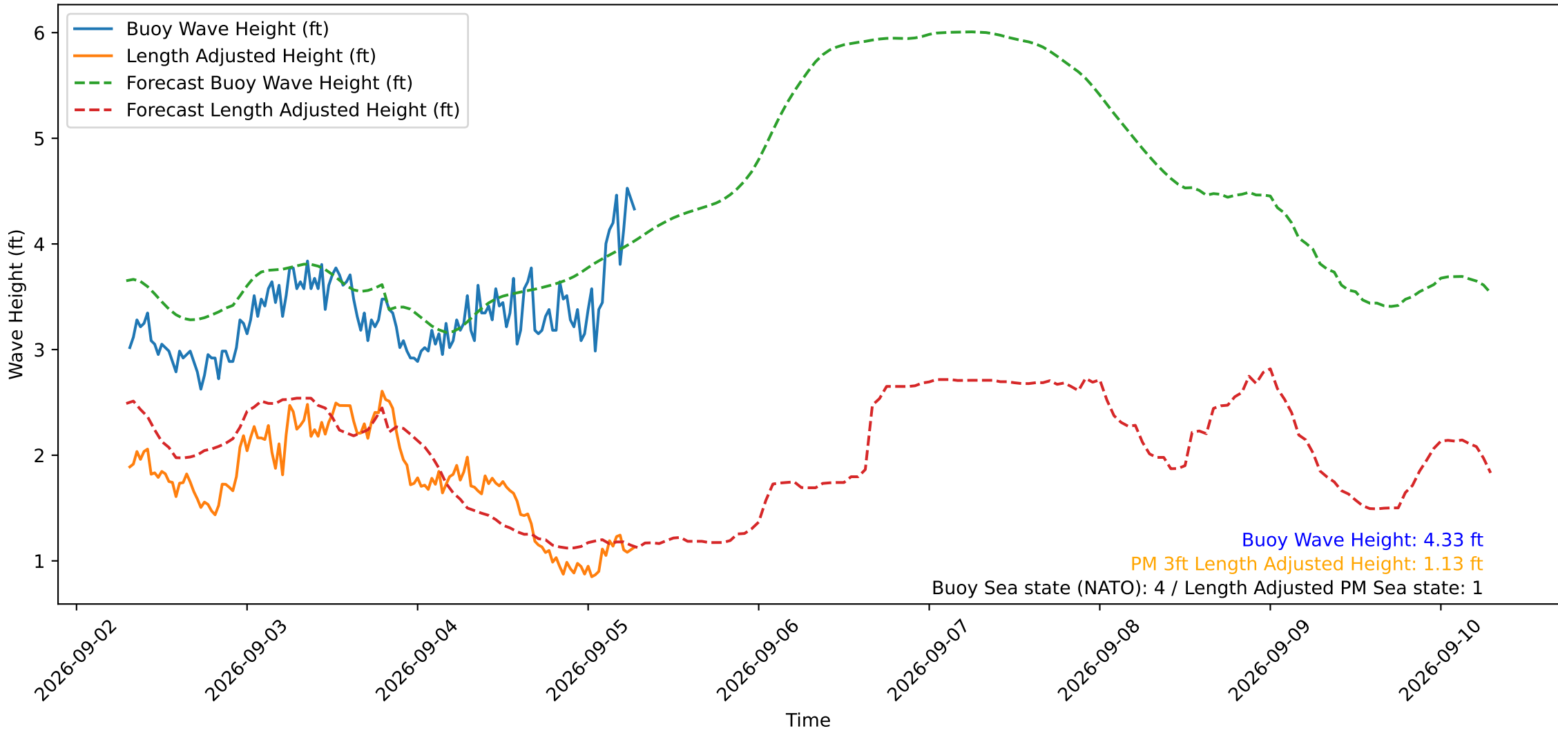
Wave Heights over Time for Oceanside Harbor at 2026-09-05 07:20:29
