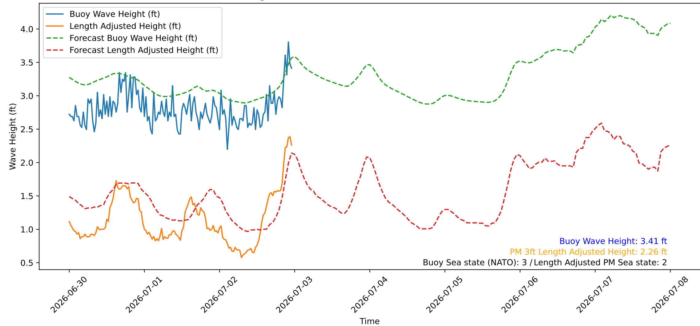
Wave Heights over Time for Red Beach at 2026-07-02 23:40:45
