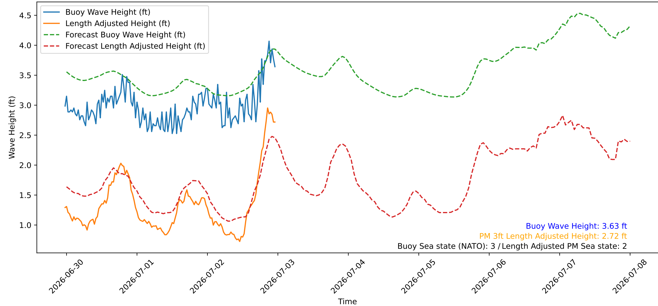
Wave Heights over Time for Green Beach at 2026-07-02 23:41:08
