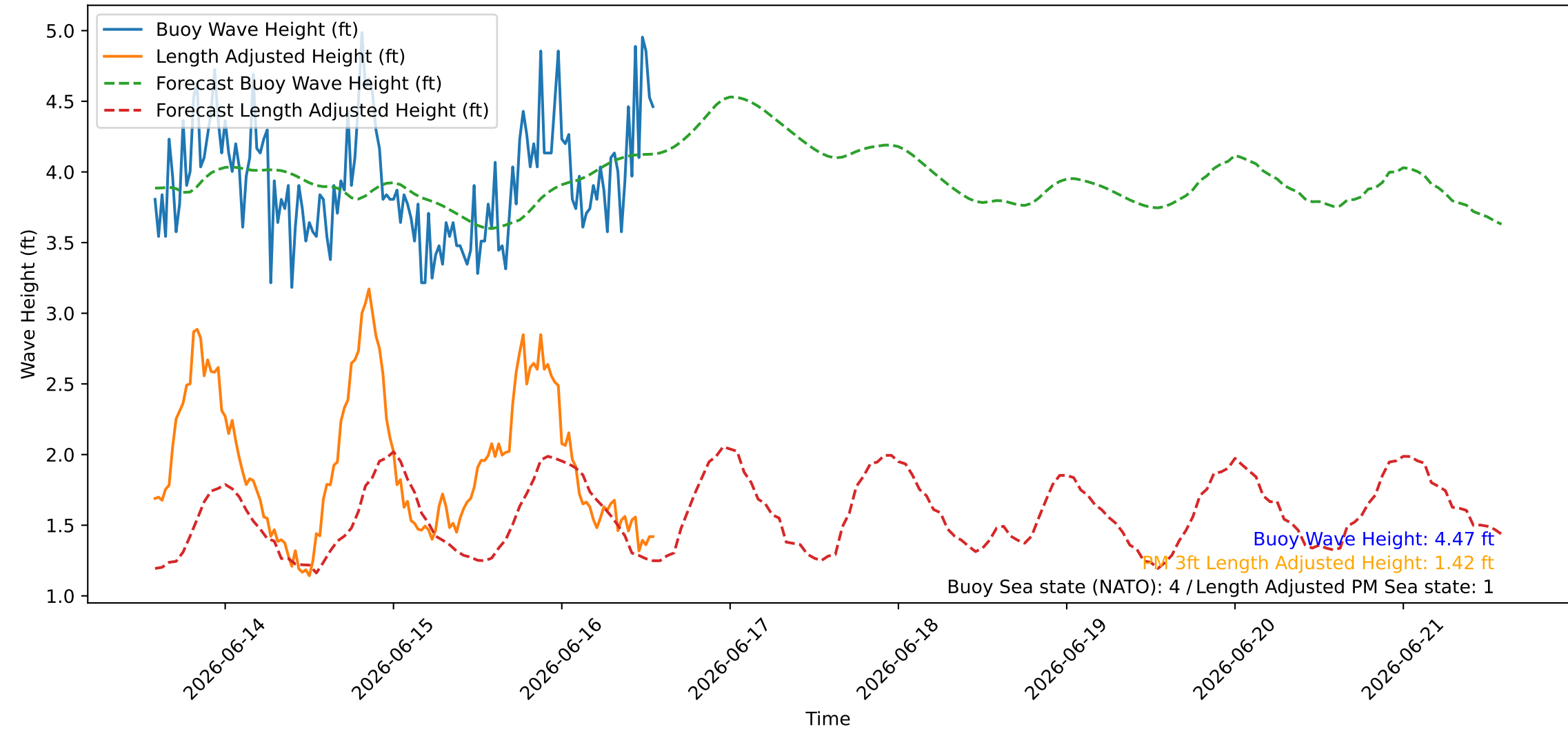
Wave Heights over Time for Oceanside Harbor at 2026-06-16 13:50:26
