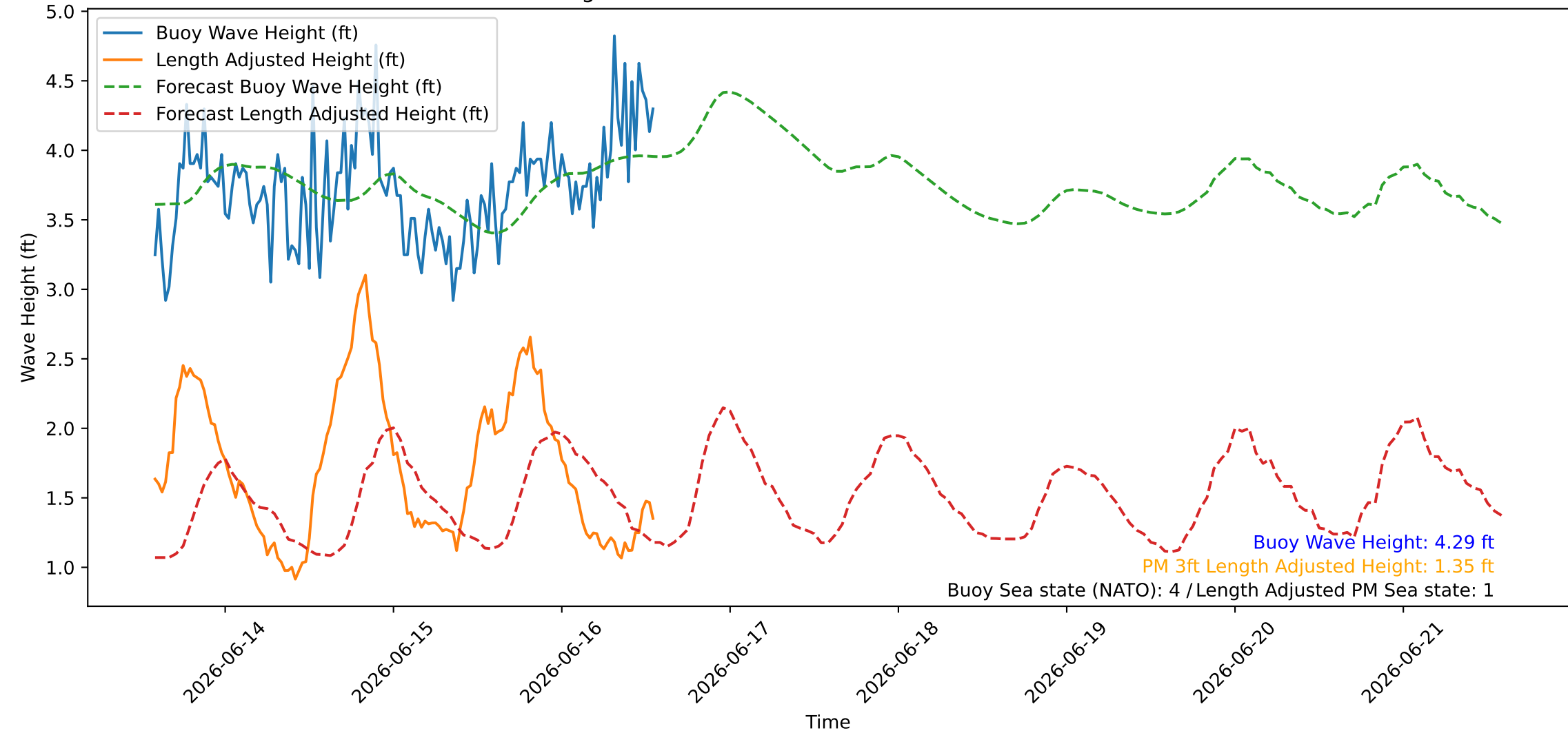
Wave Heights over Time for Red Beach at 2026-06-16 13:50:47
