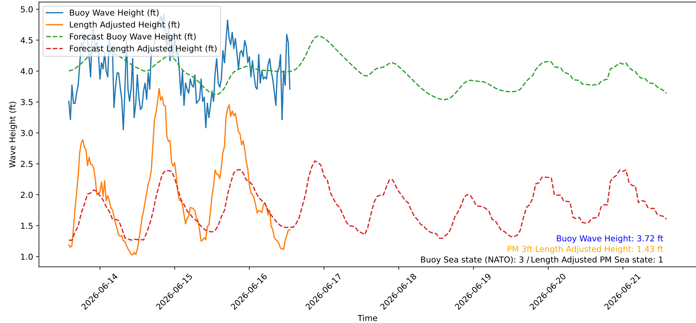
Wave Heights over Time for Green Beach at 2026-06-16 13:51:09
