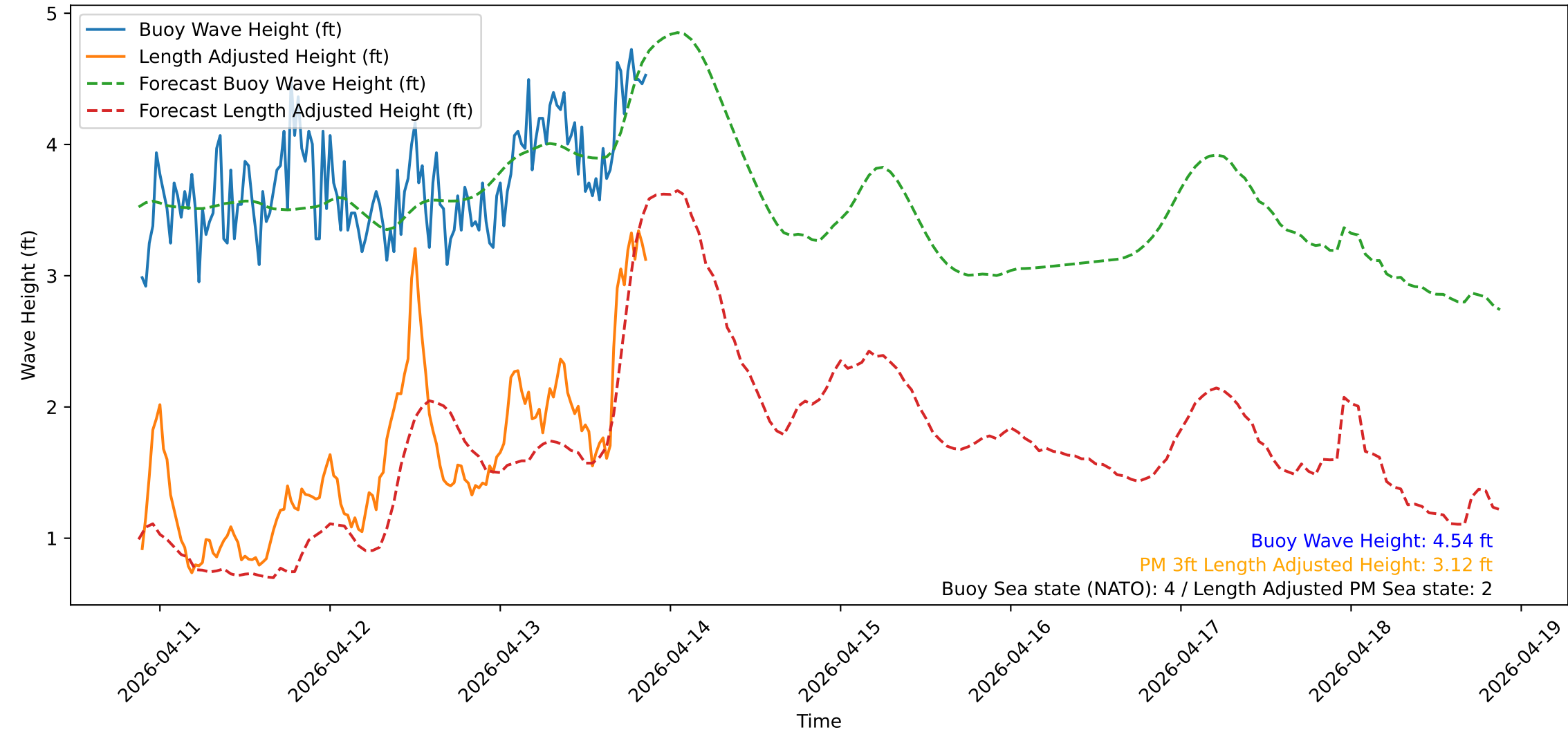
Wave Heights over Time for Green Beach at 2026-04-13 21:21:13
