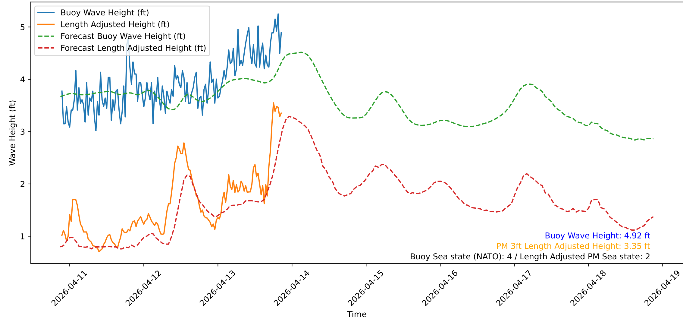
Wave Heights over Time for Oceanside Harbor at 2026-04-13 21:20:31
