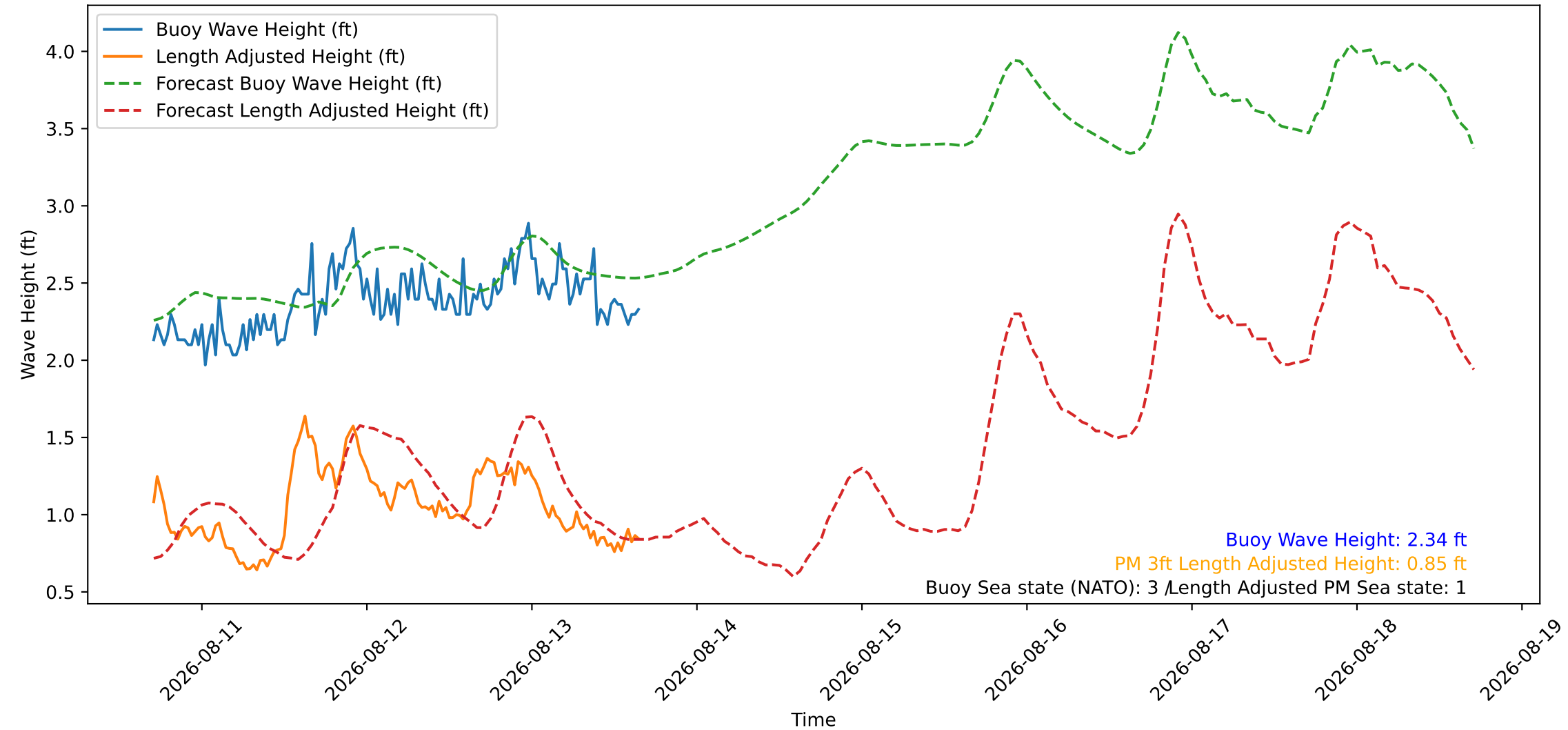
Wave Heights over Time for Red Beach at 2026-08-13 16:40:47
