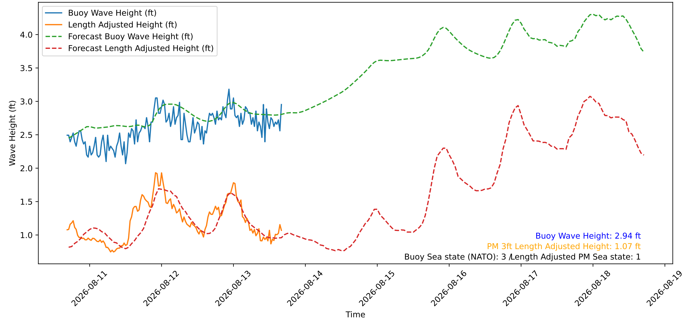
Wave Heights over Time for Oceanside Harbor at 2026-08-13 16:40:27
