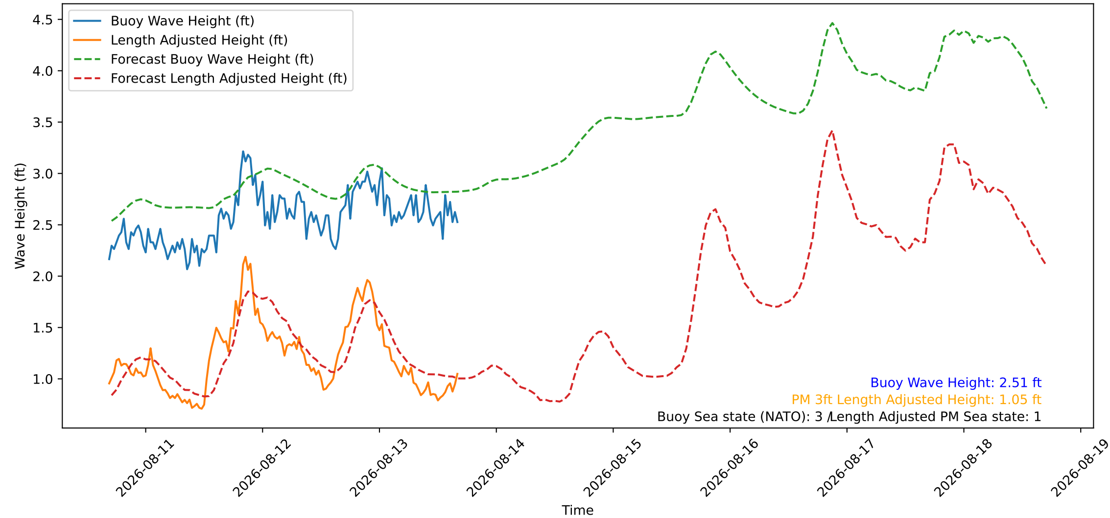
Wave Heights over Time for Green Beach at 2026-08-13 16:41:09
