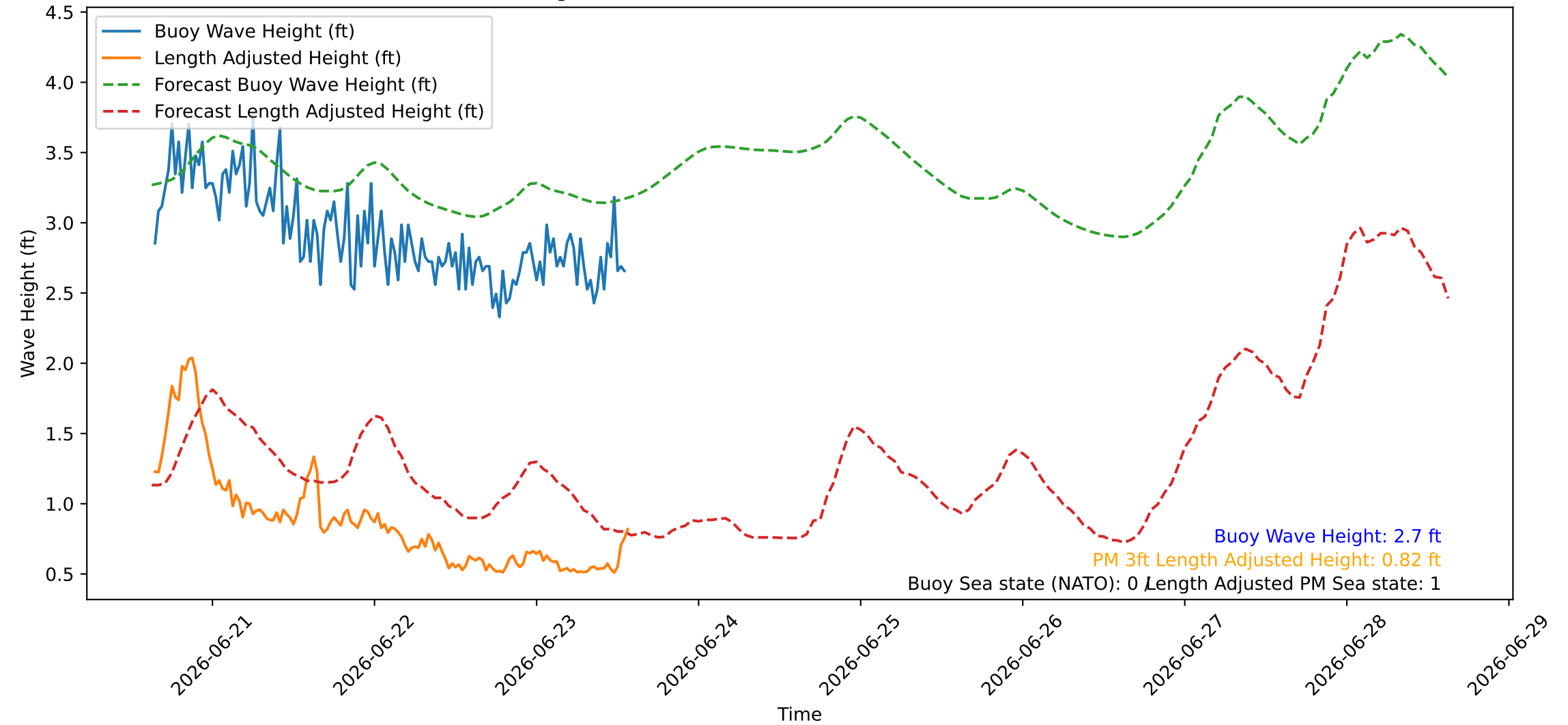
Wave Heights over Time for Red Beach at 2026-06-23 15:20:45
