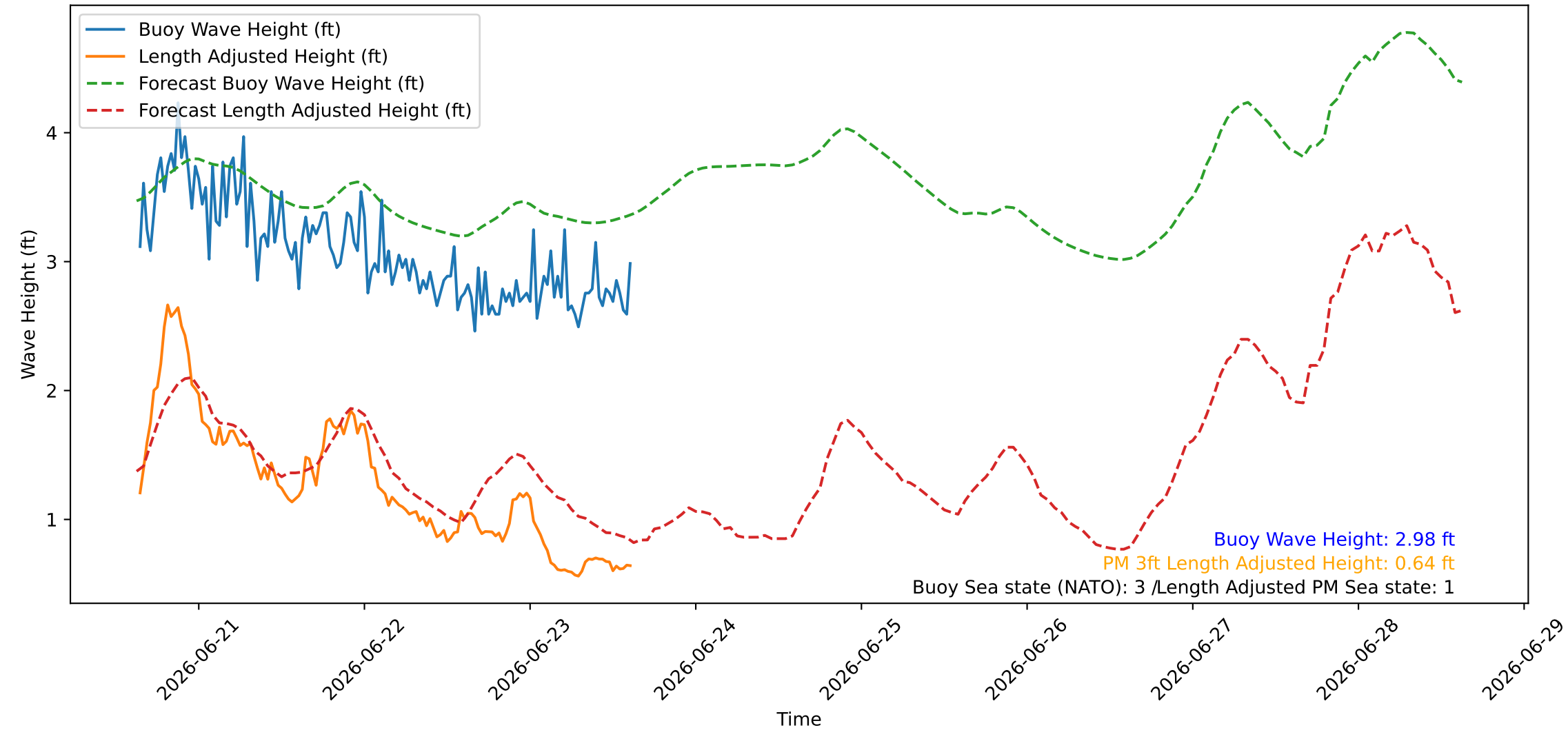
Wave Heights over Time for Green Beach at 2026-06-23 15:21:08
