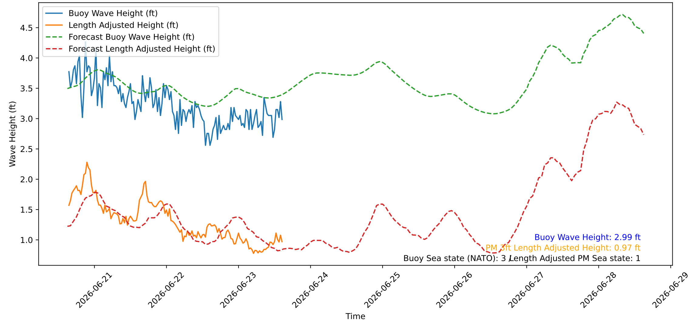
Wave Heights over Time for Oceanside Harbor at 2026-06-23 15:20:25
