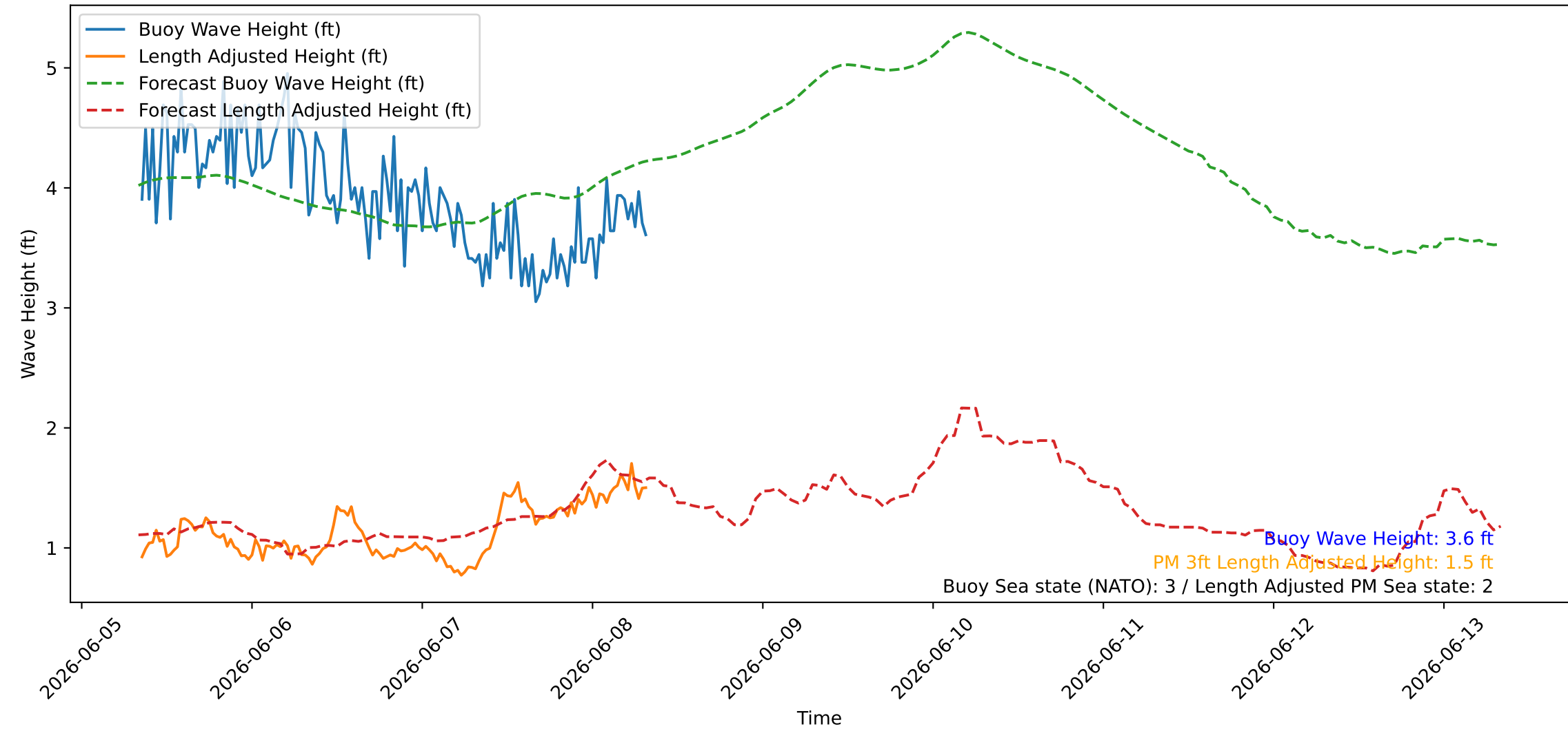
Wave Heights over Time for Red Beach at 2026-06-08 08:20:47
