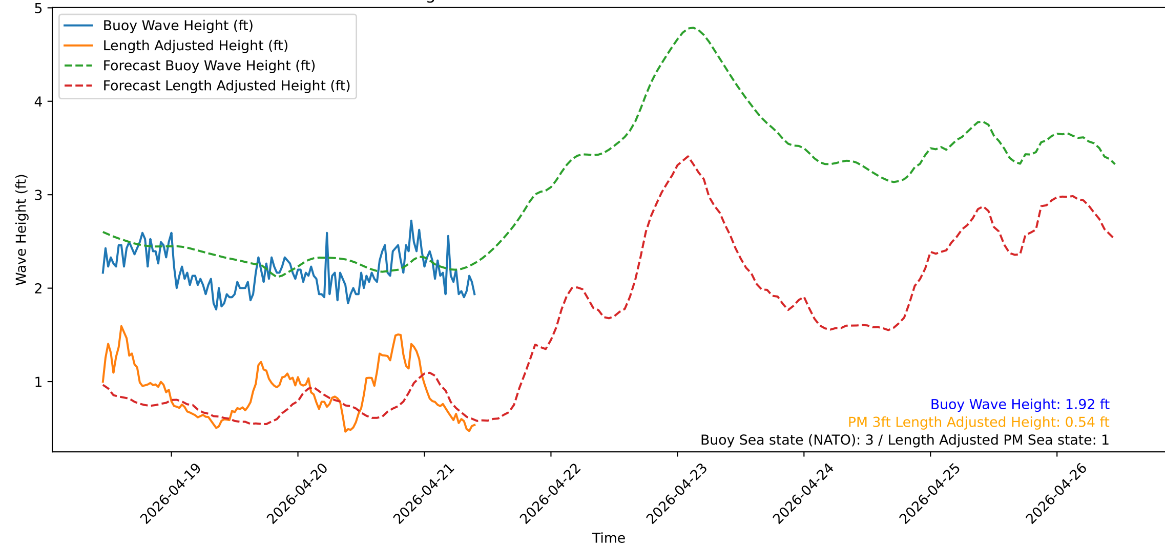
Wave Heights over Time for Red Beach at 2026-04-21 10:30:51
