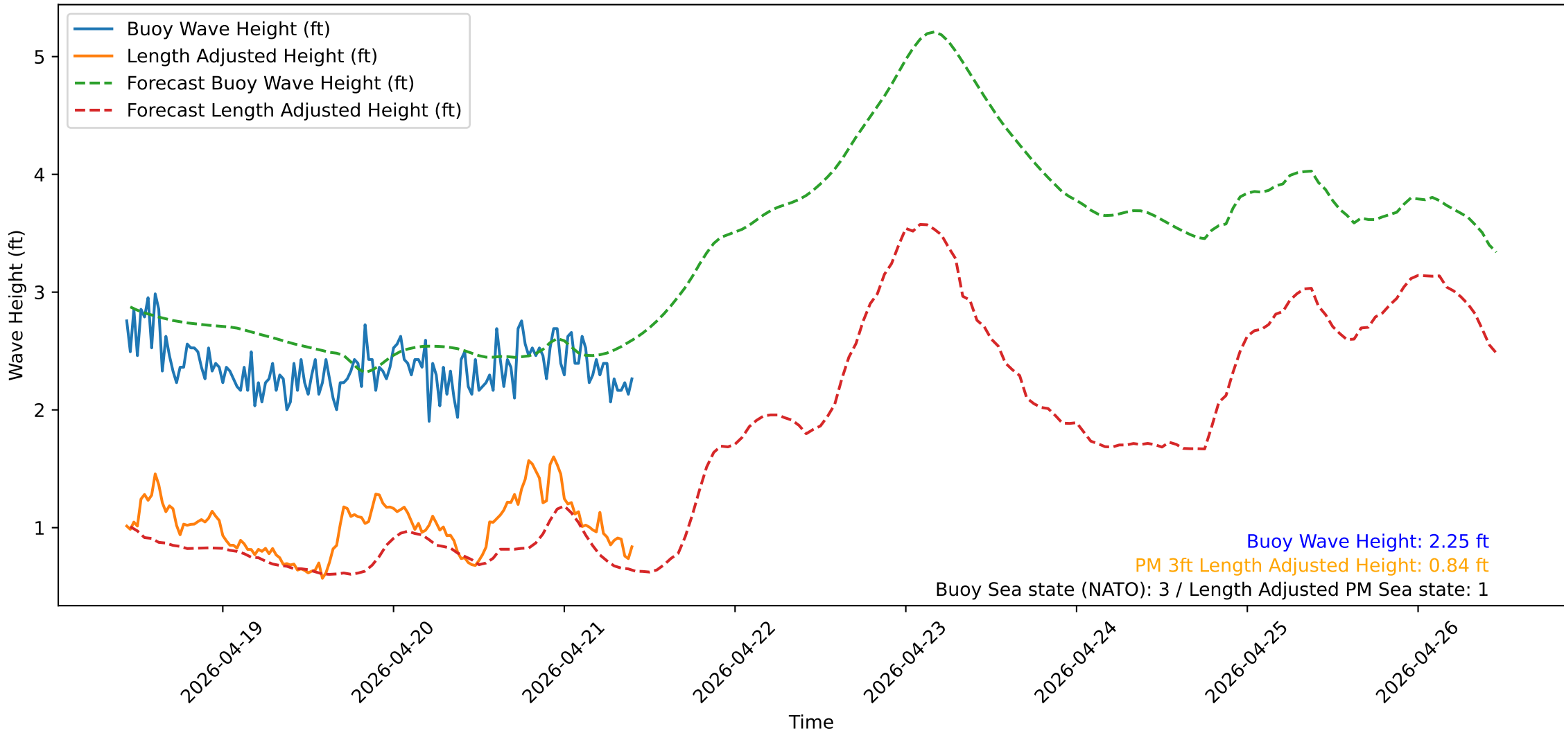
Wave Heights over Time for Oceanside Harbor at 2026-04-21 10:30:32
