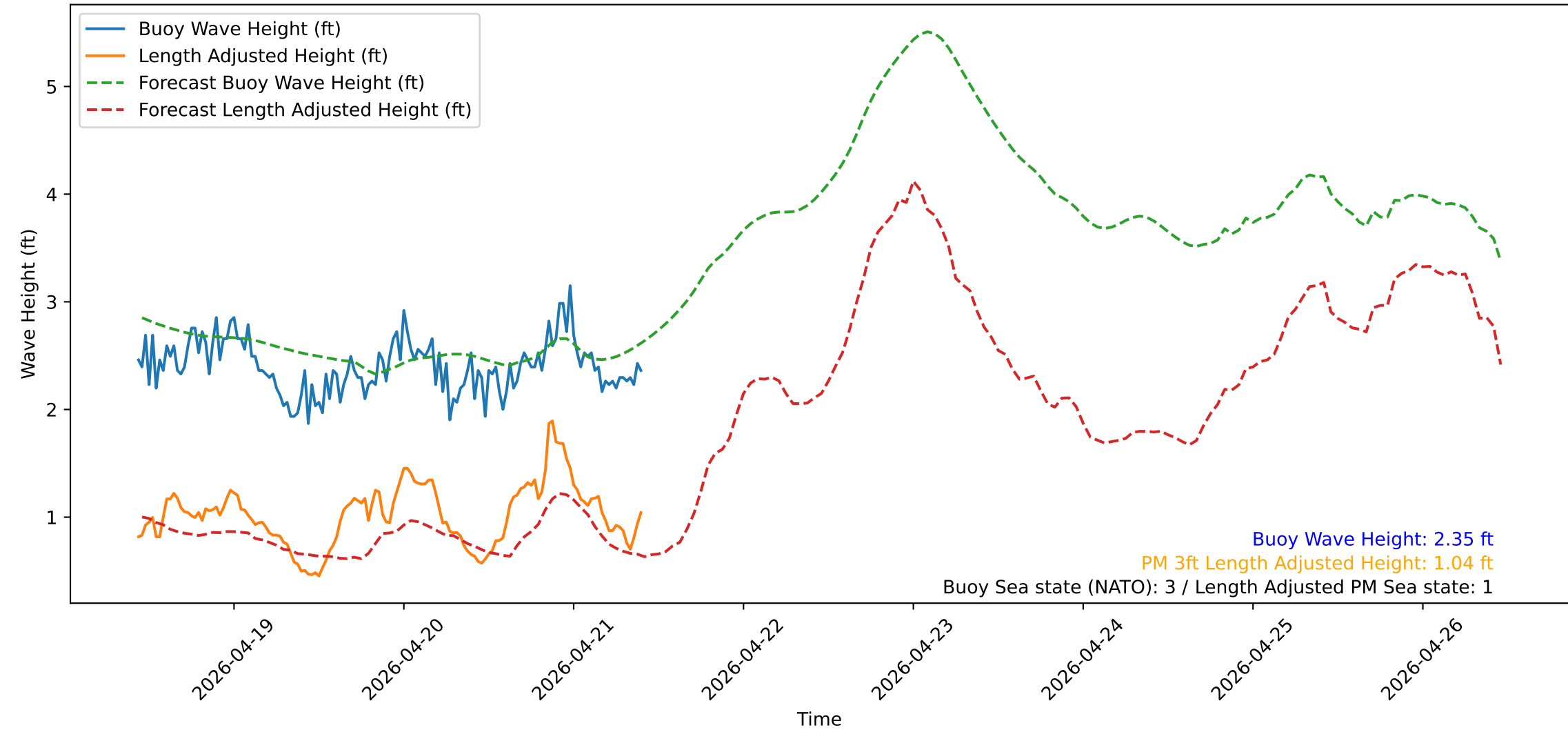
Wave Heights over Time for Green Beach at 2026-04-21 10:31:14
