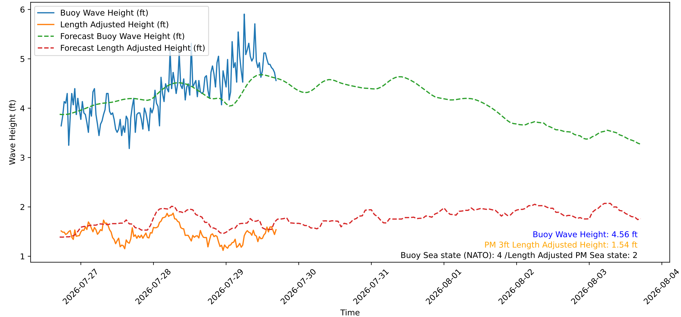
Wave Heights over Time for Oceanside Harbor at 2026-07-29 17:20:26
