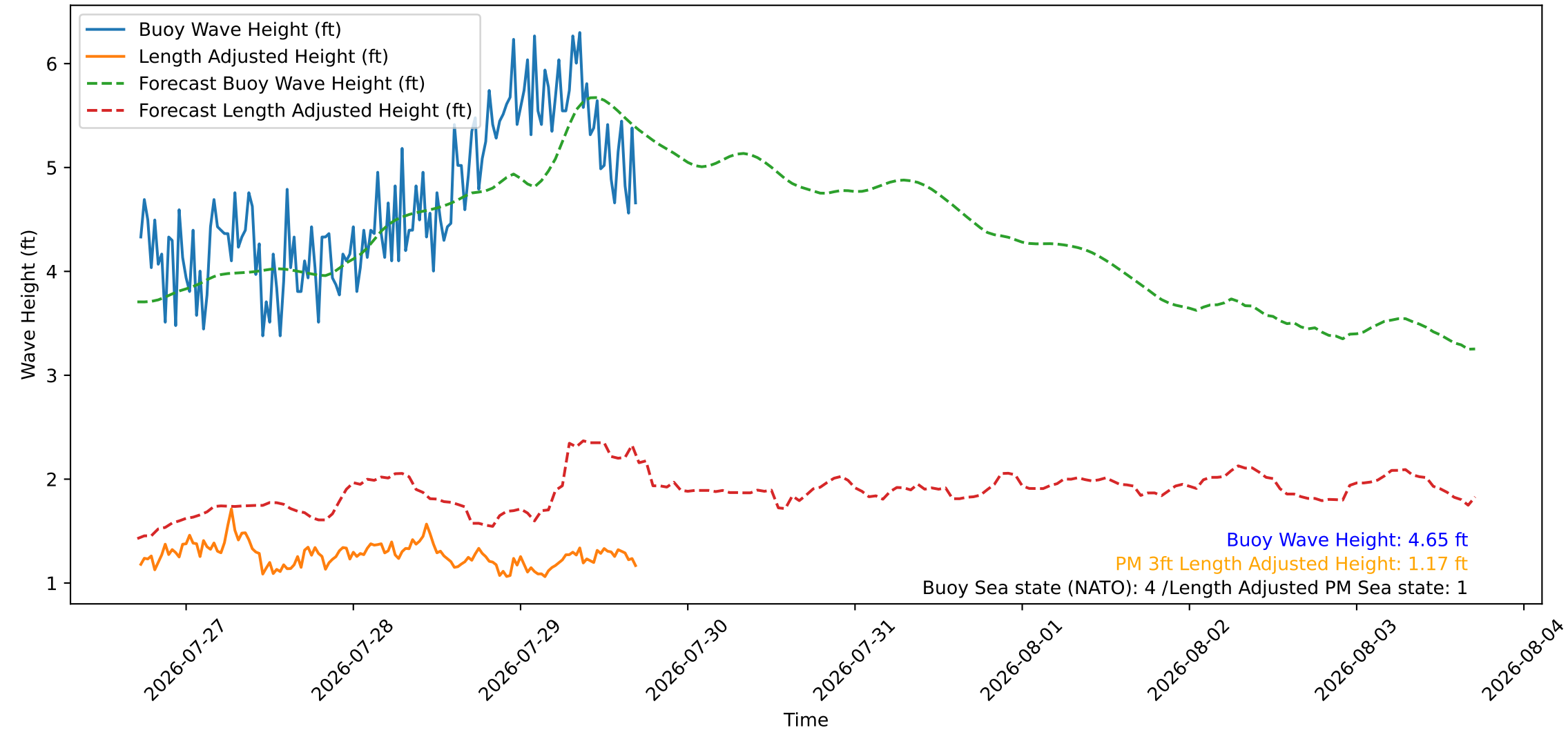
Wave Heights over Time for Green Beach at 2026-07-29 17:21:10
