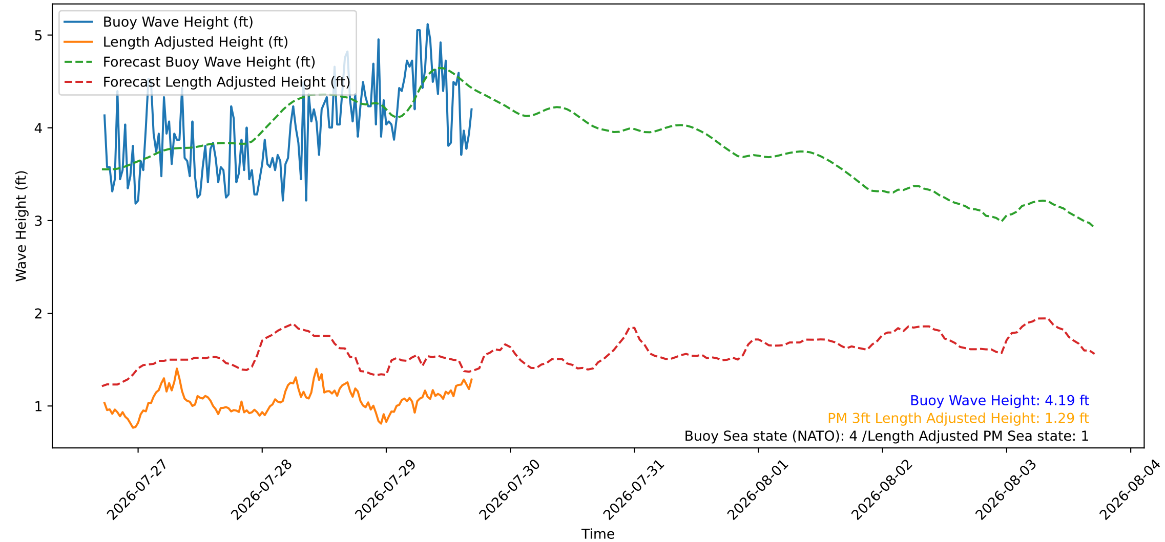
Wave Heights over Time for Red Beach at 2026-07-29 17:20:48
