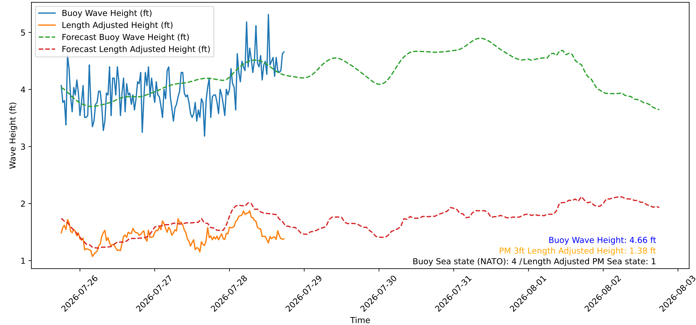
Wave Heights over Time for Oceanside Harbor at 2026-07-28 18:10:26
