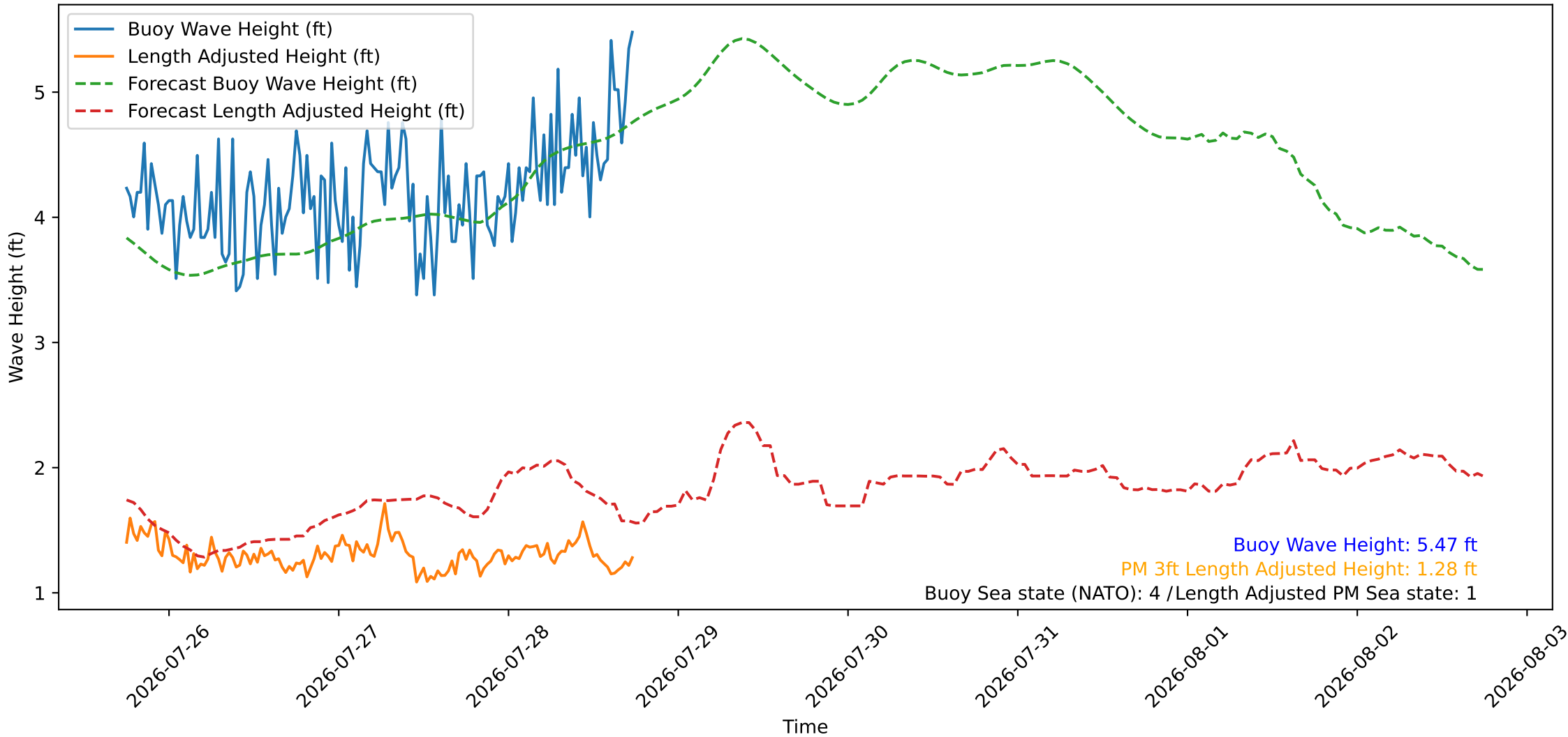
Wave Heights over Time for Green Beach at 2026-07-28 18:11:08
