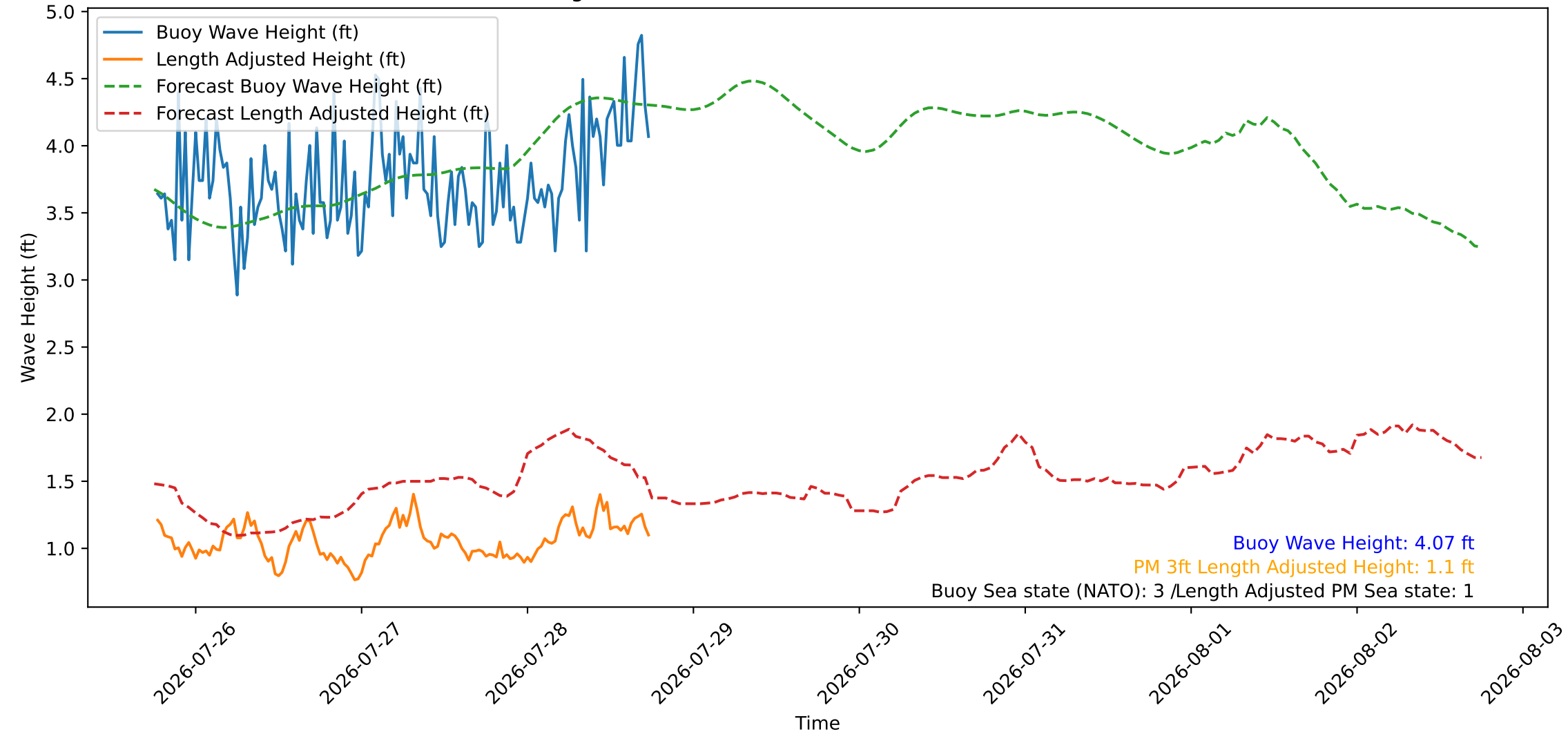
Wave Heights over Time for Red Beach at 2026-07-28 18:10:46
