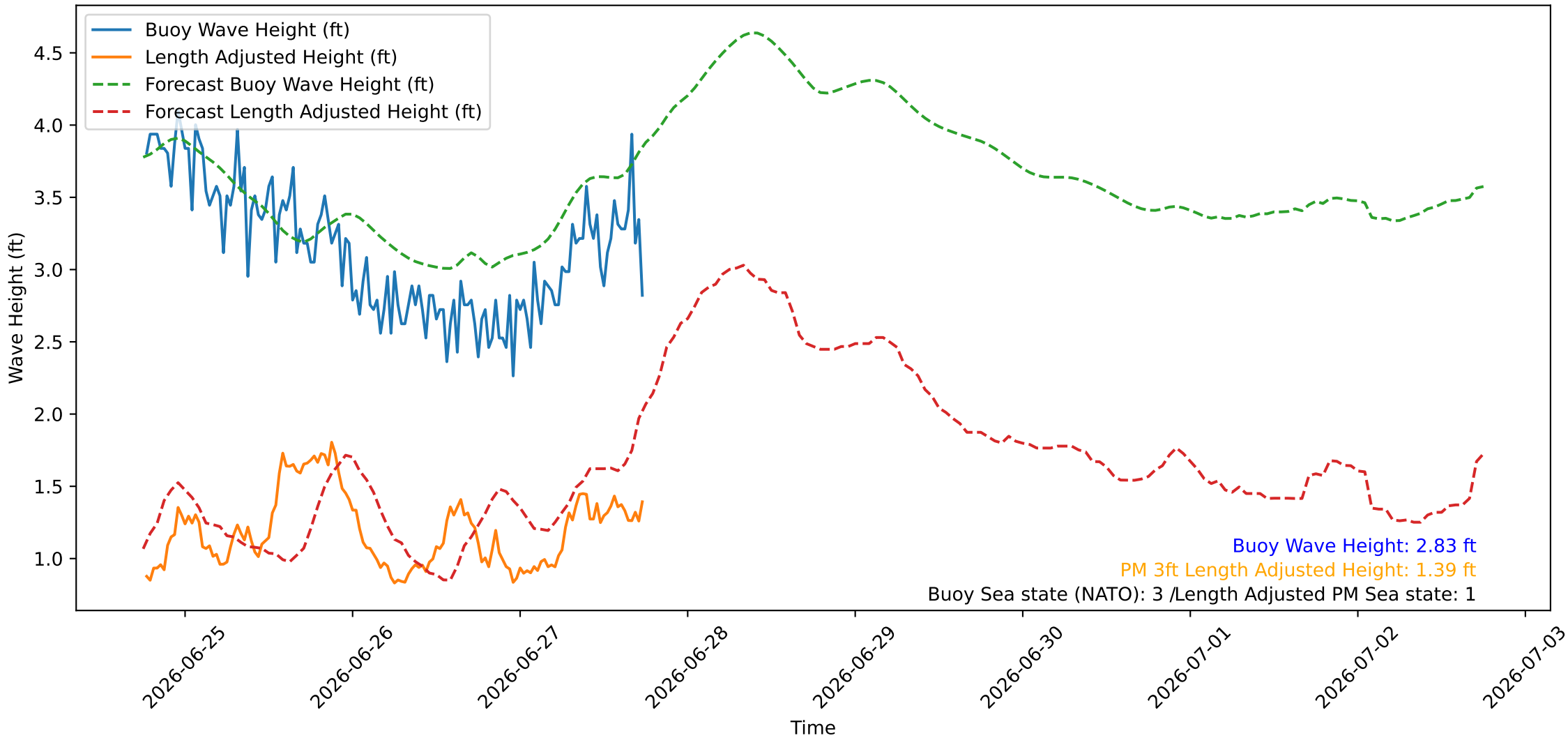
Wave Heights over Time for Green Beach at 2026-06-27 18:21:10
