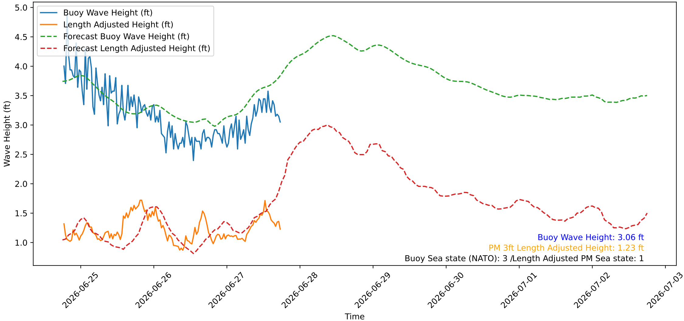
Wave Heights over Time for Oceanside Harbor at 2026-06-27 18:20:27
