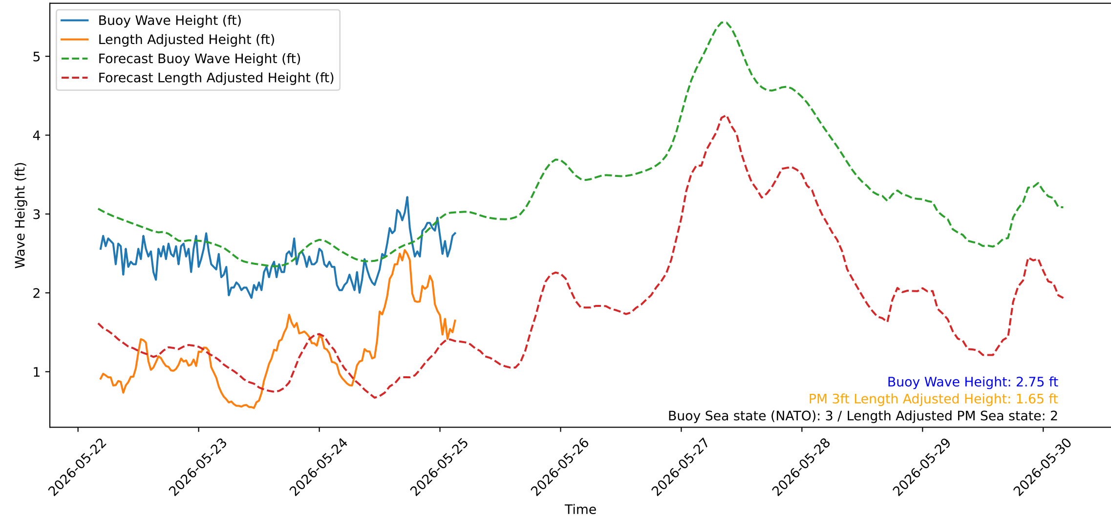
Wave Heights over Time for Red Beach at 2026-05-25 04:00:50
