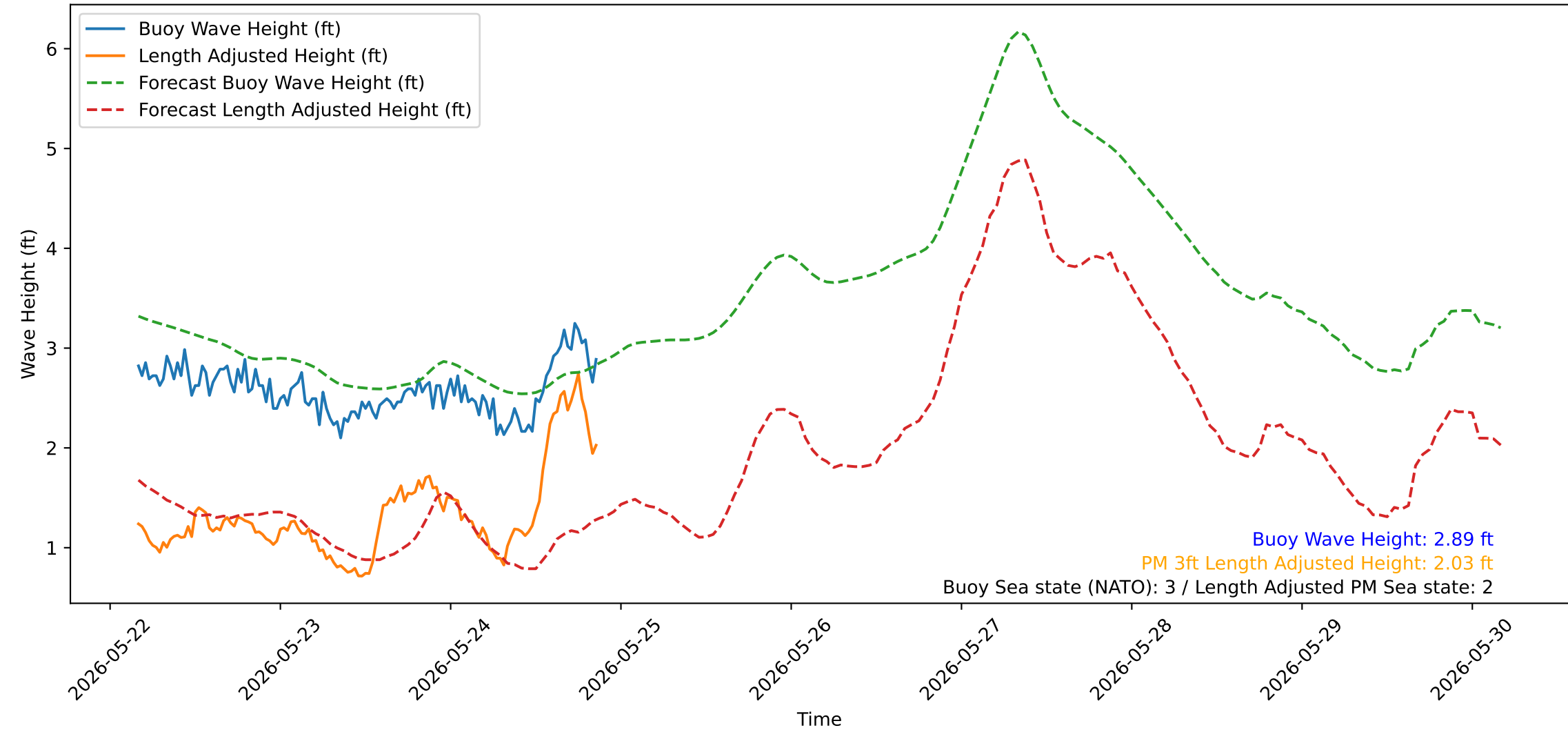
Wave Heights over Time for Oceanside Harbor at 2026-05-25 04:00:31
