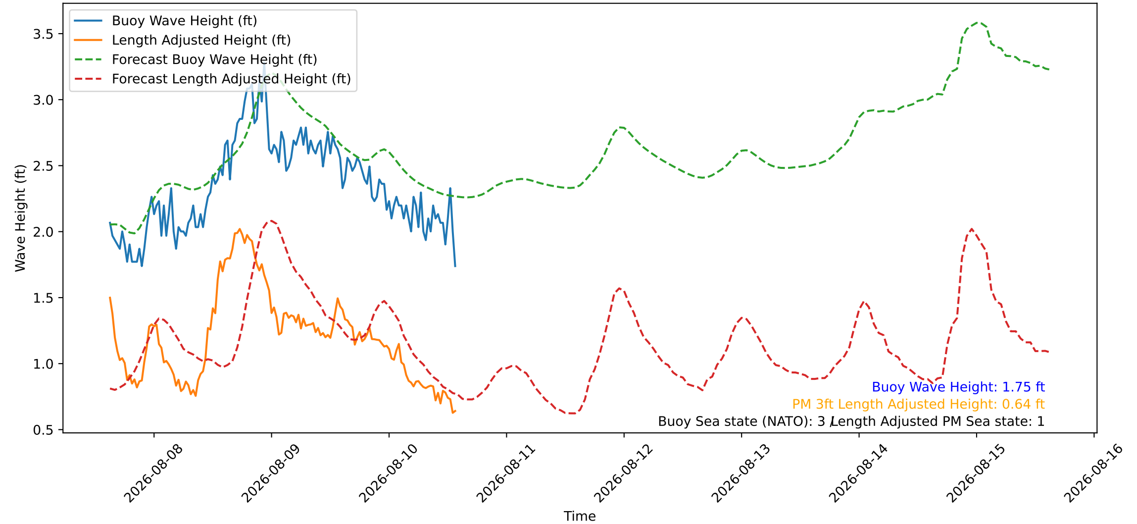
Wave Heights over Time for Red Beach at 2026-08-10 14:40:46
