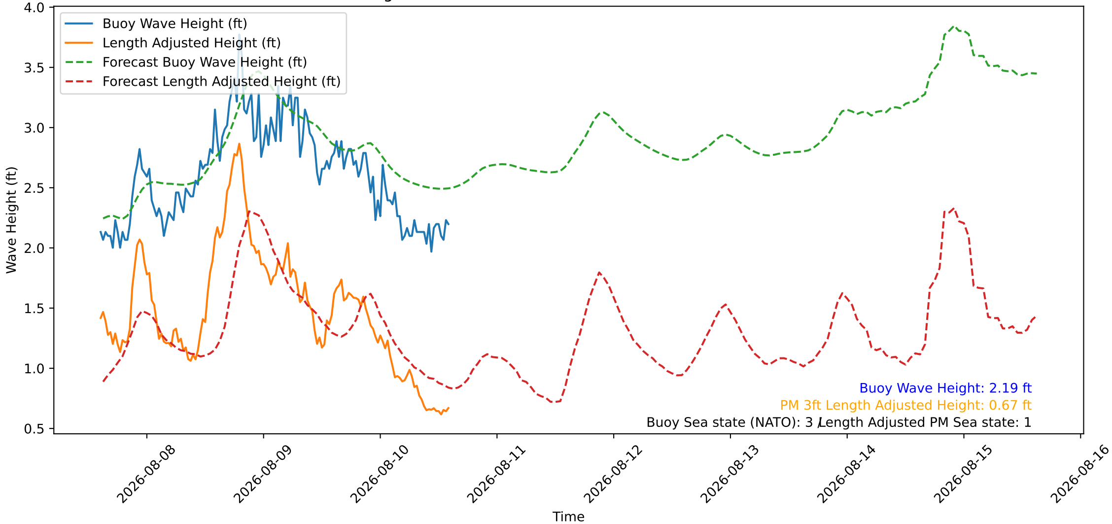
Wave Heights over Time for Green Beach at 2026-08-10 14:41:09
