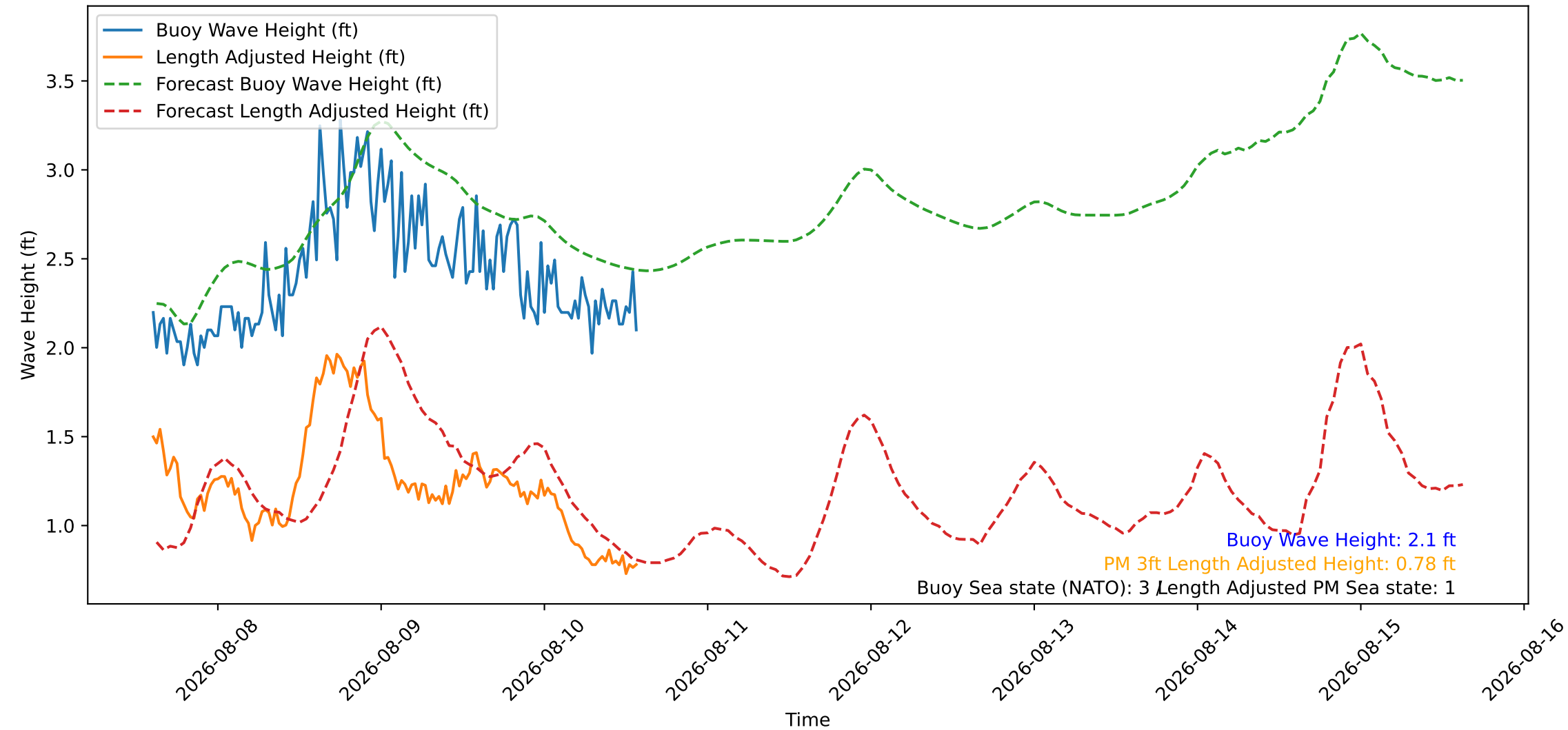
Wave Heights over Time for Oceanside Harbor at 2026-08-10 14:40:26
