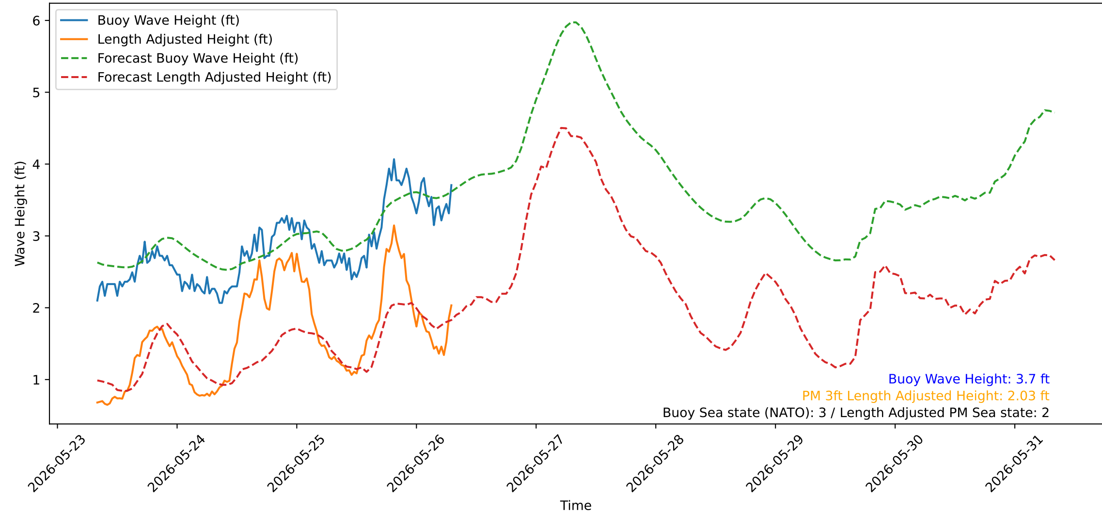
Wave Heights over Time for Green Beach at 2026-05-26 07:51:12
