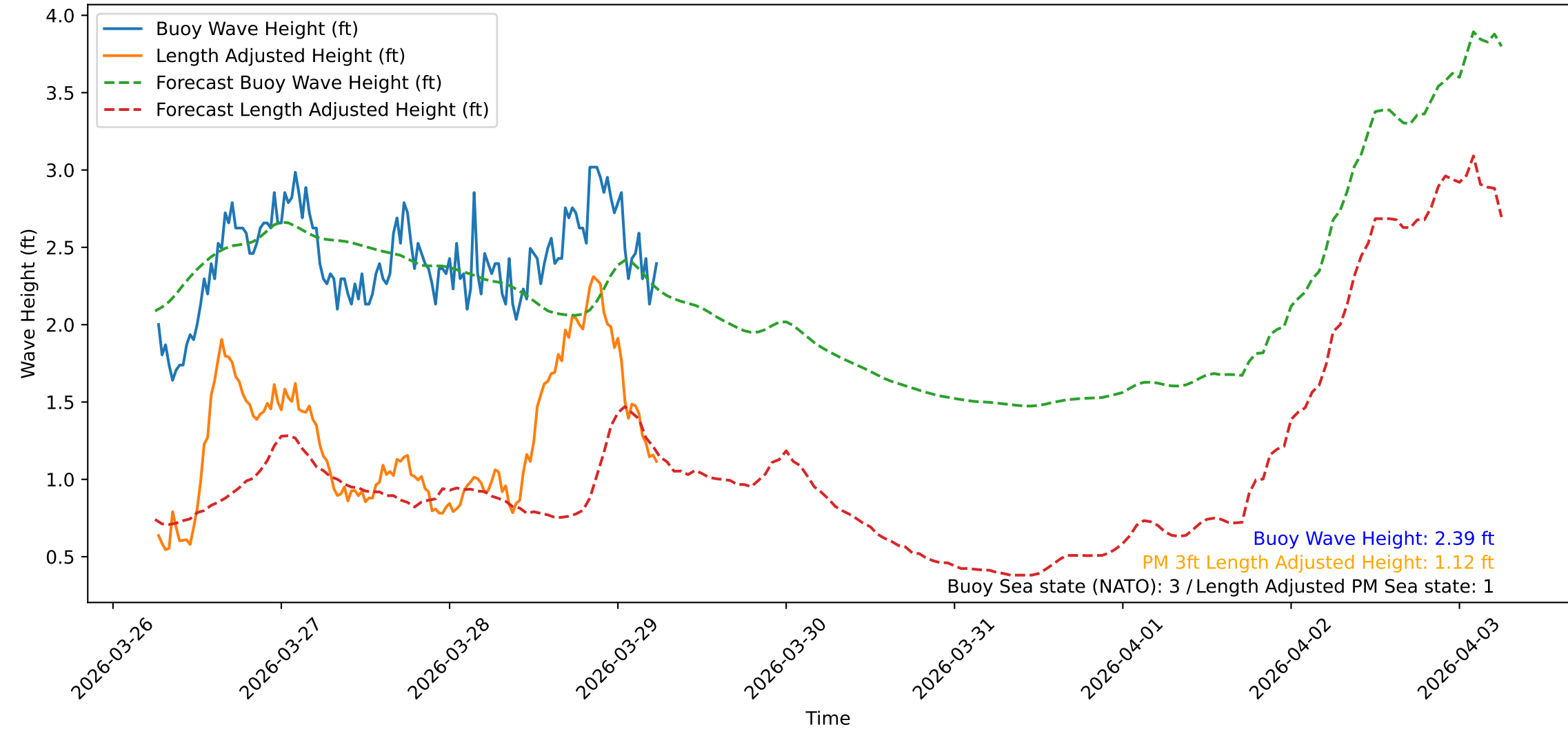
Wave Heights over Time for Red Beach at 2026-03-29 06:20:47
