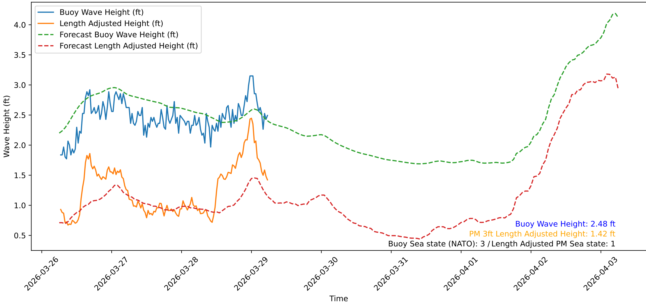
Wave Heights over Time for Oceanside Harbor at 2026-03-29 06:20:31
