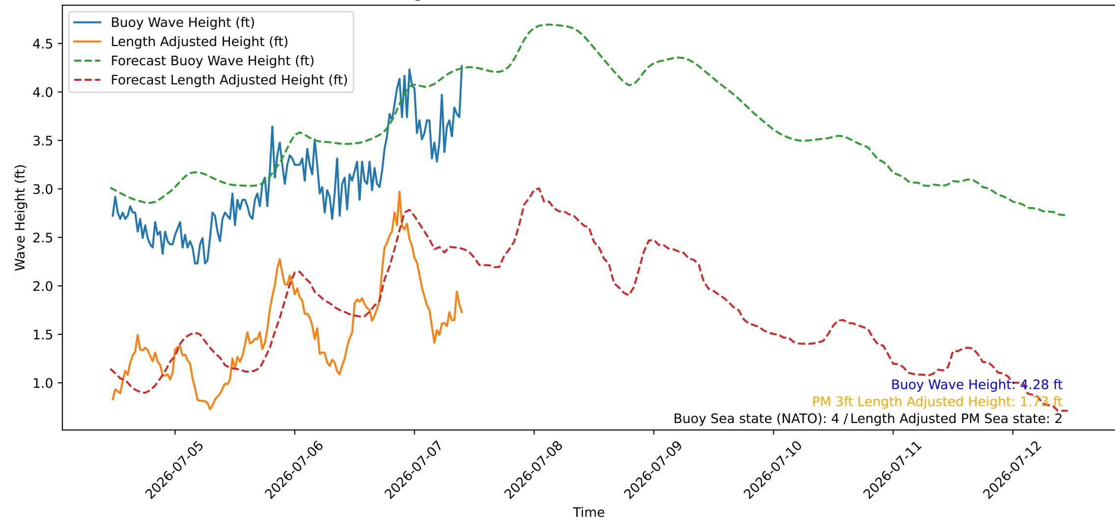
Wave Heights over Time for Red Beach at 2026-07-07 11:00:45
