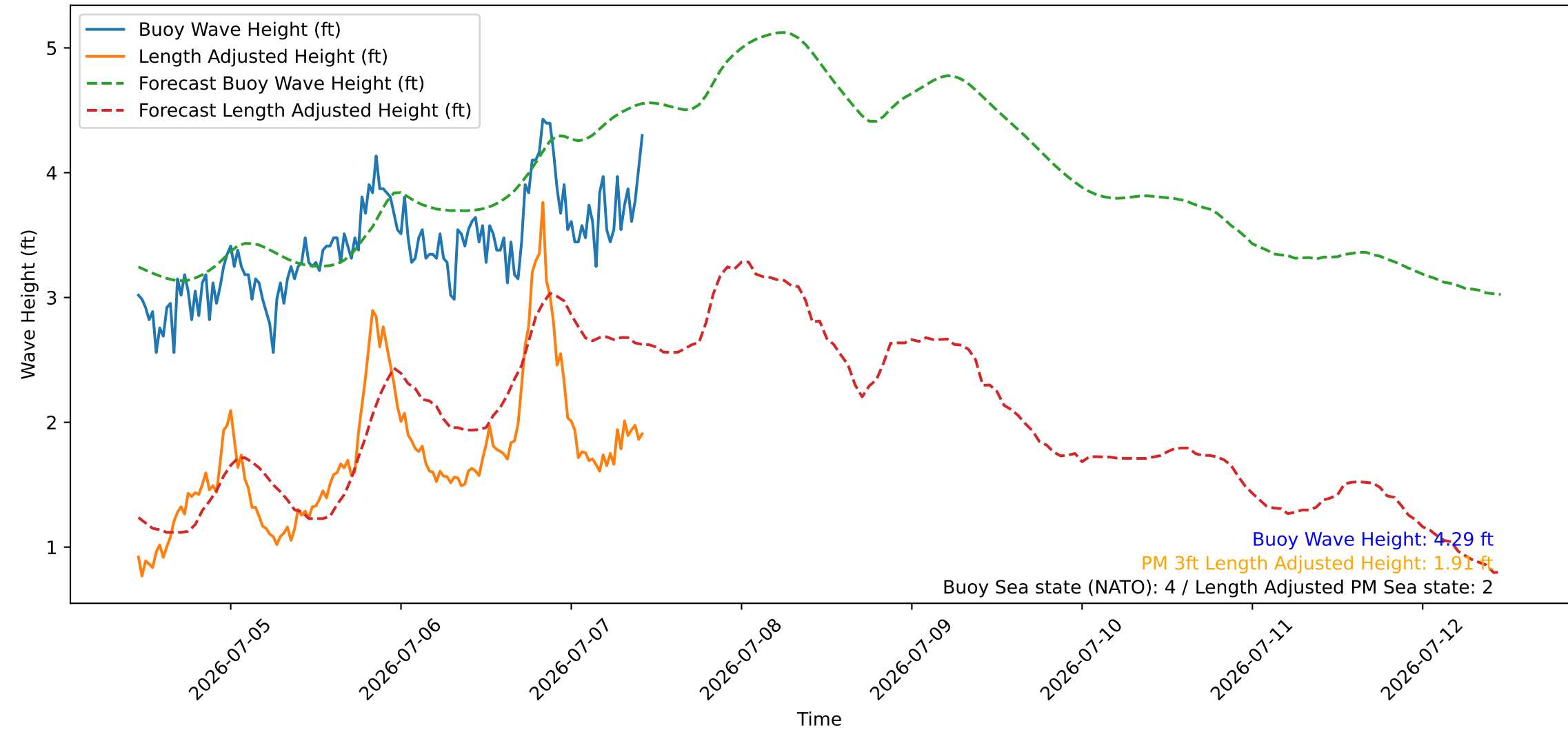
Wave Heights over Time for Green Beach at 2026-07-07 11:01:08
