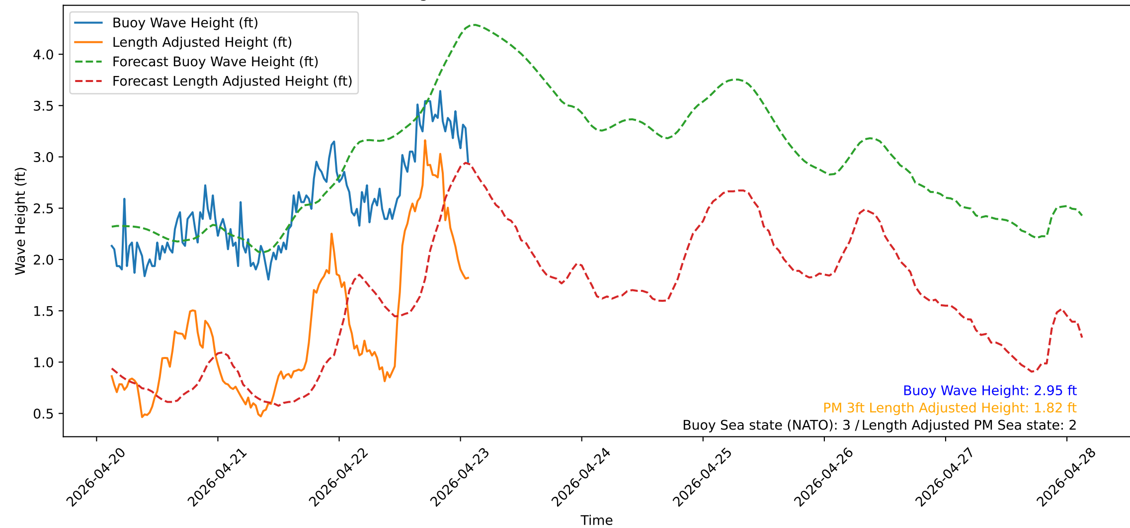
Wave Heights over Time for Red Beach at 2026-04-23 02:40:51
