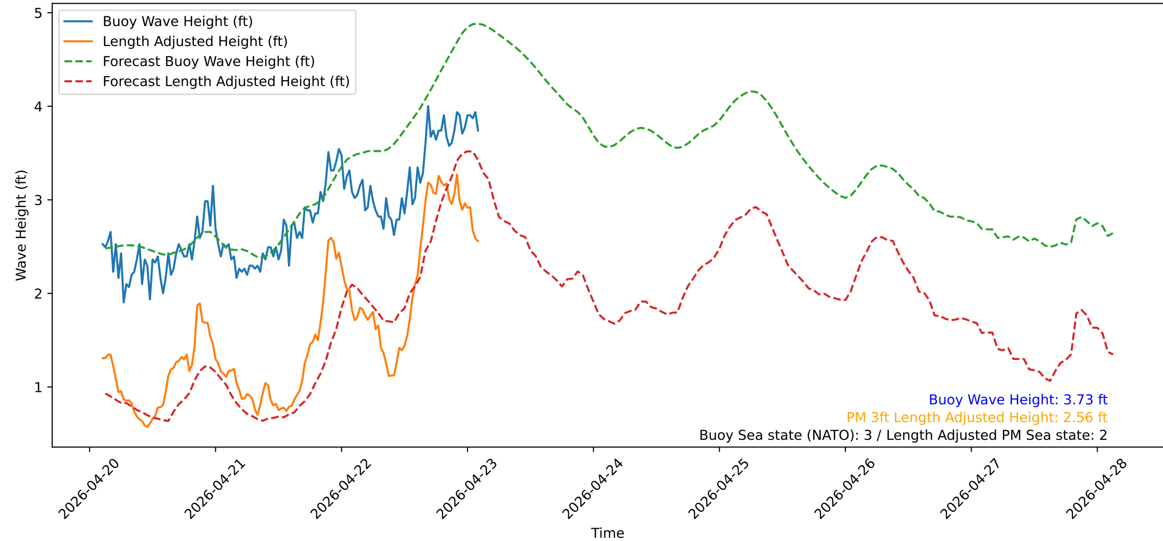
Wave Heights over Time for Green Beach at 2026-04-23 02:41:14
