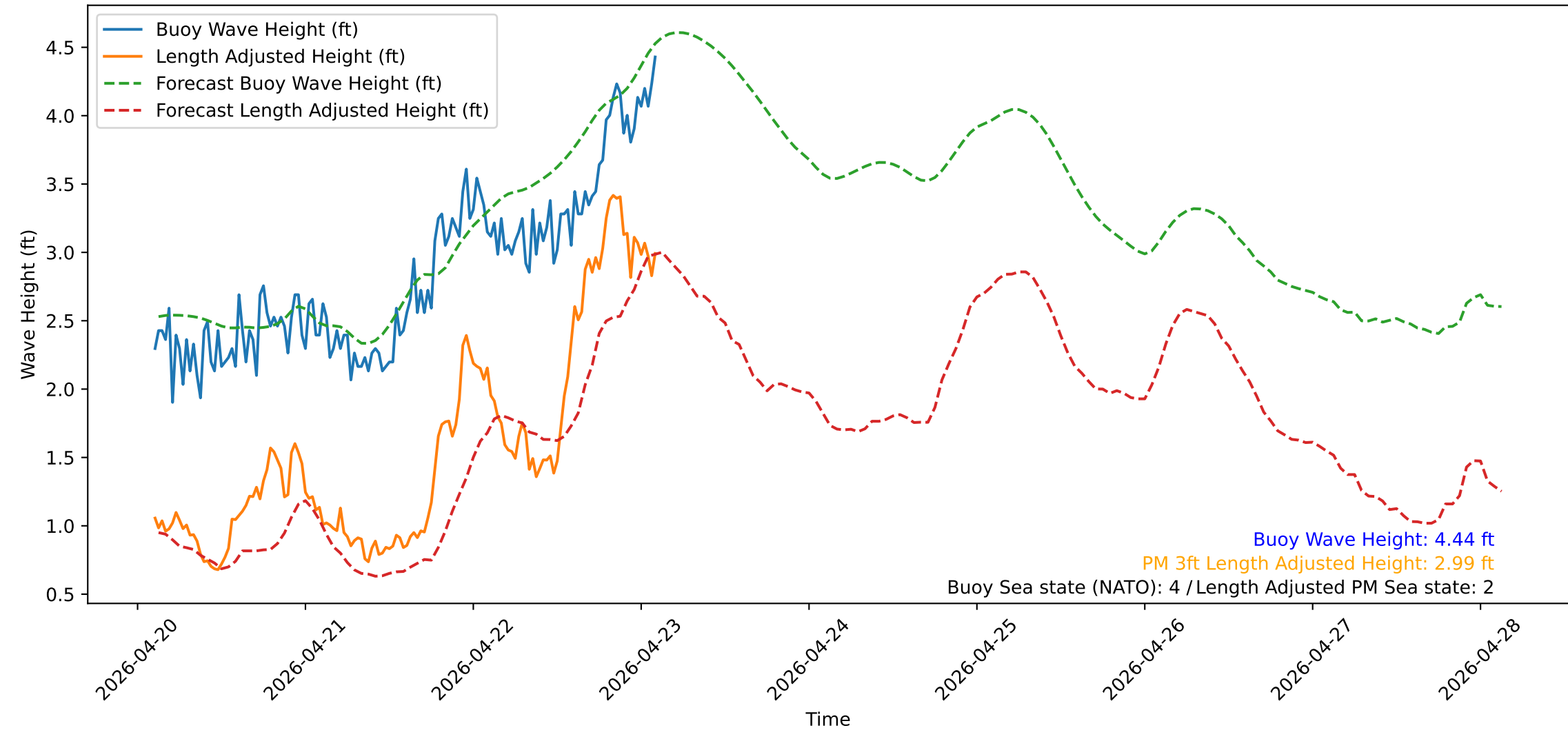
Wave Heights over Time for Oceanside Harbor at 2026-04-23 02:40:31
