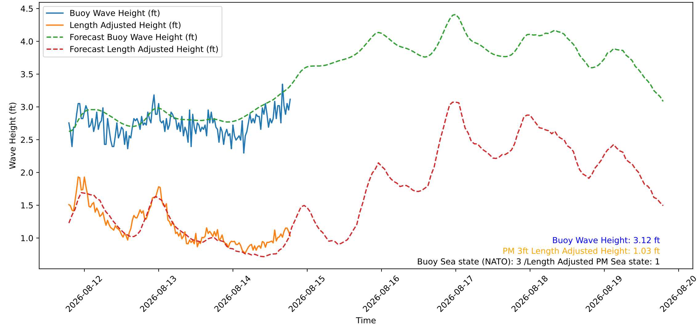
Wave Heights over Time for Oceanside Harbor at 2026-08-14 19:10:26
