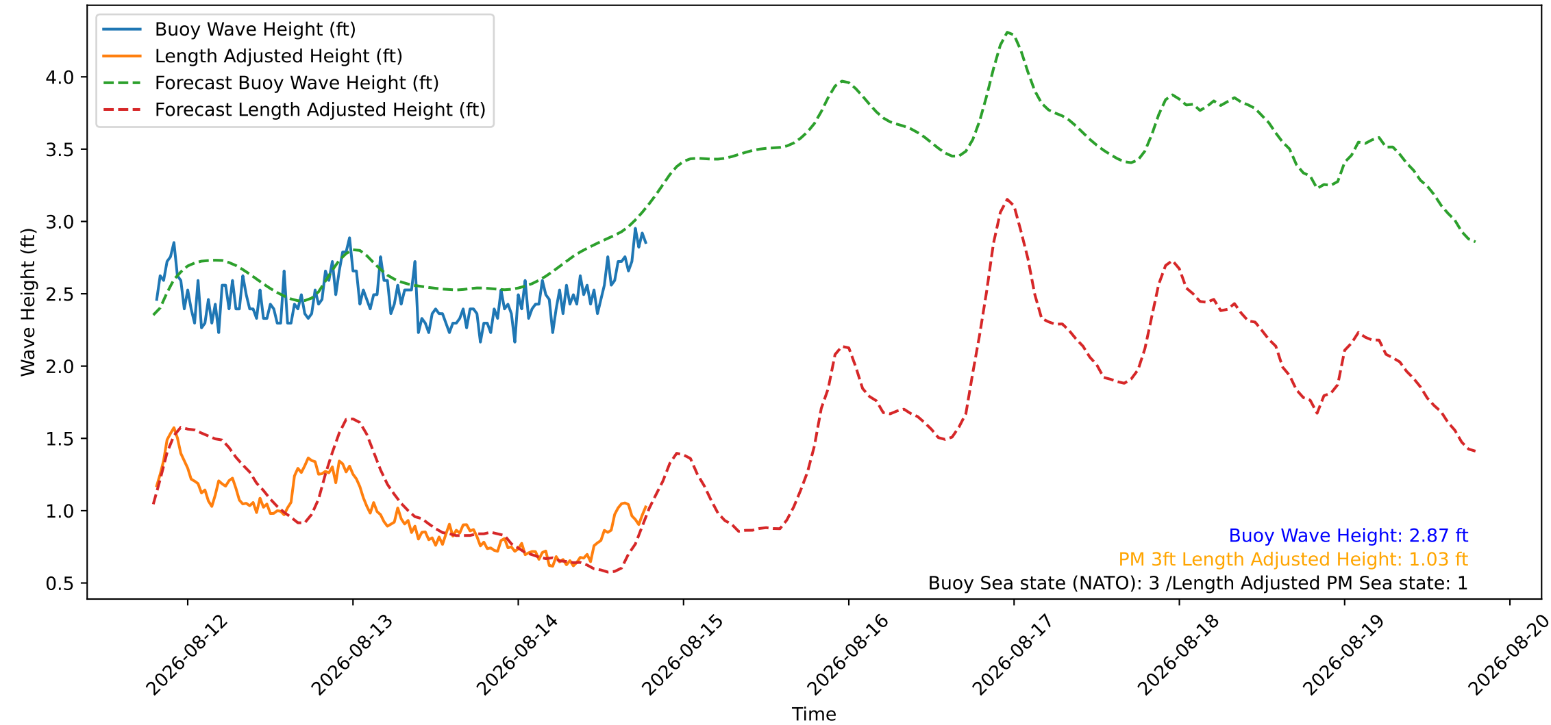
Wave Heights over Time for Red Beach at 2026-08-14 19:10:46
