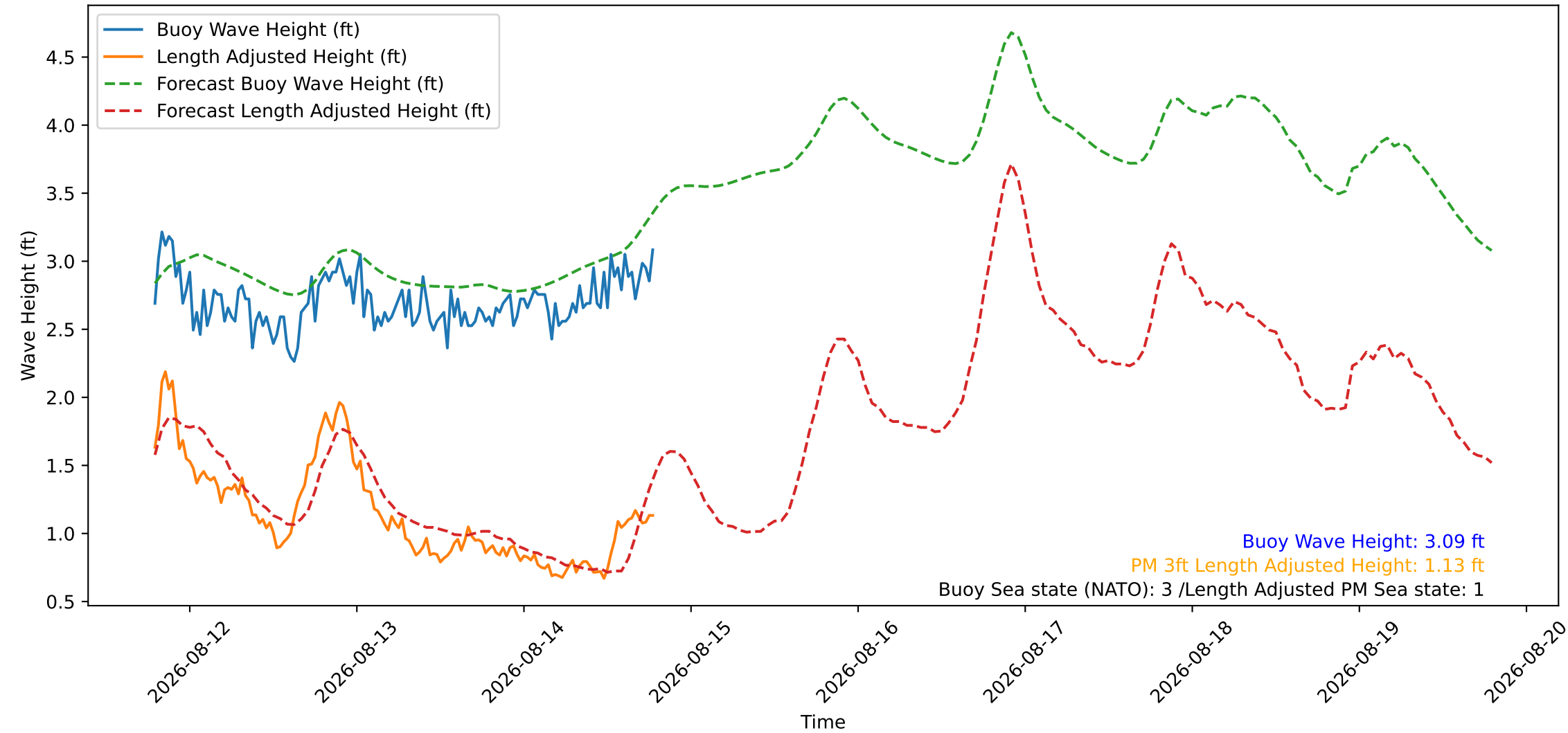
Wave Heights over Time for Green Beach at 2026-08-14 19:11:08
