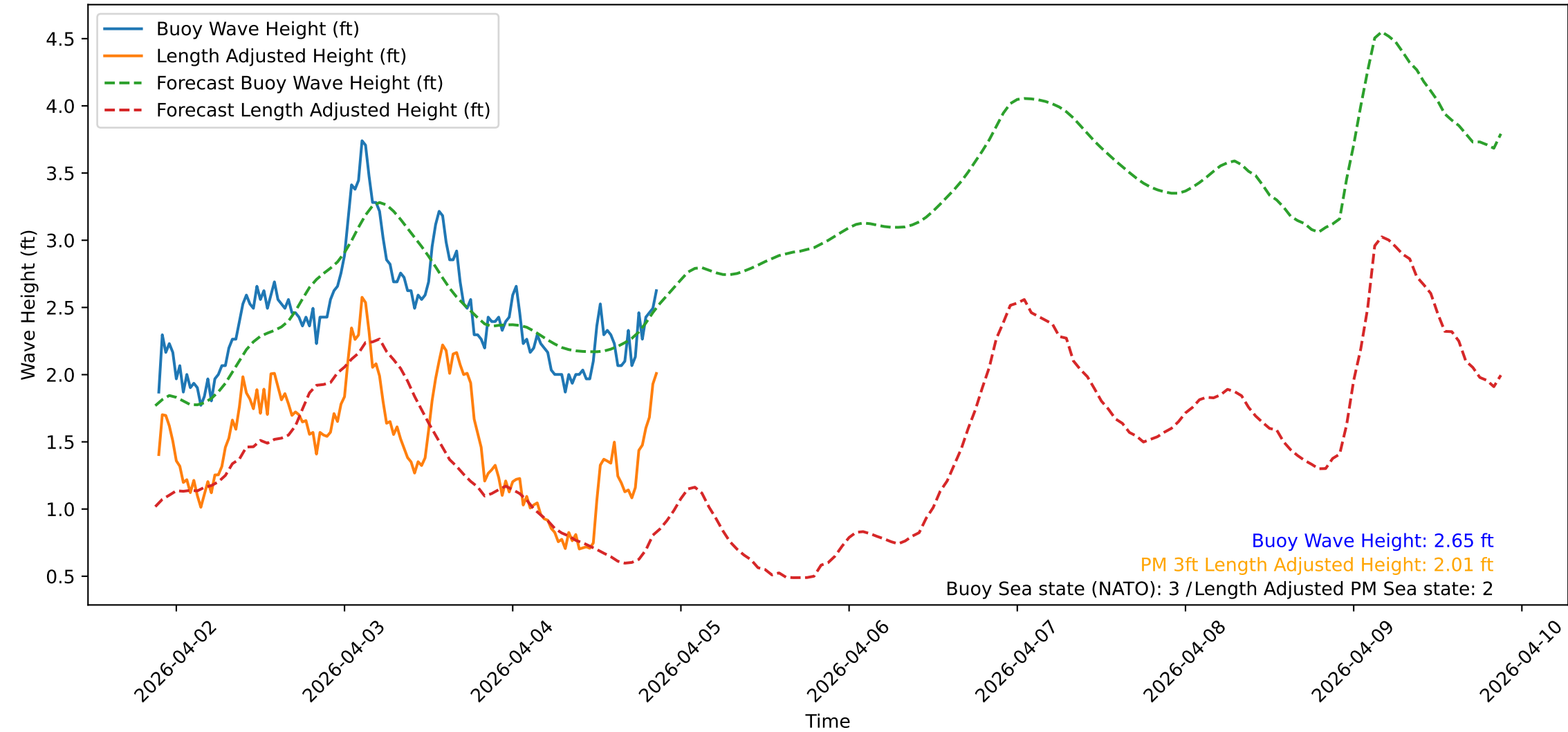
Wave Heights over Time for Red Beach at 2026-04-04 21:11:08
