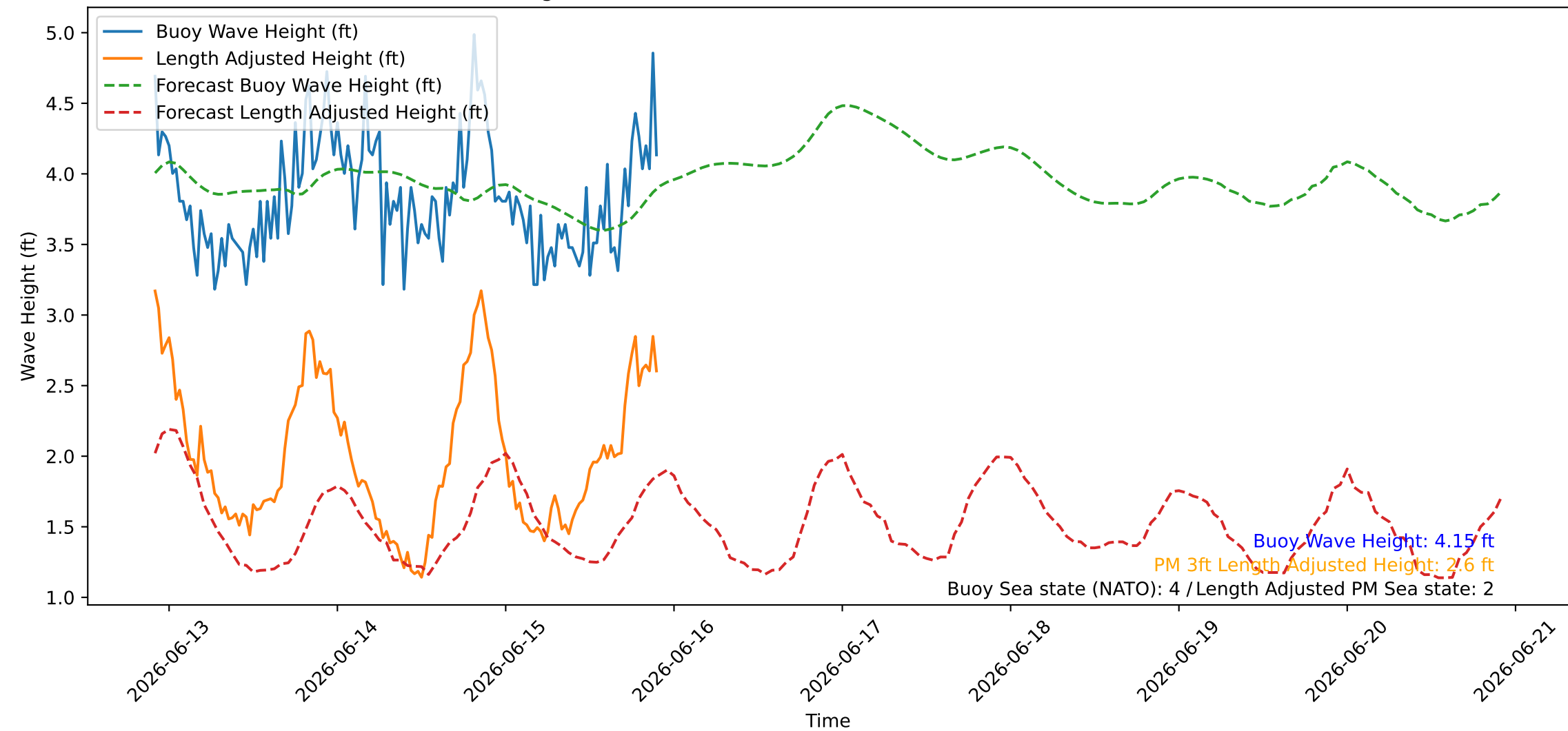
Wave Heights over Time for Oceanside Harbor at 2026-06-15 22:10:26
