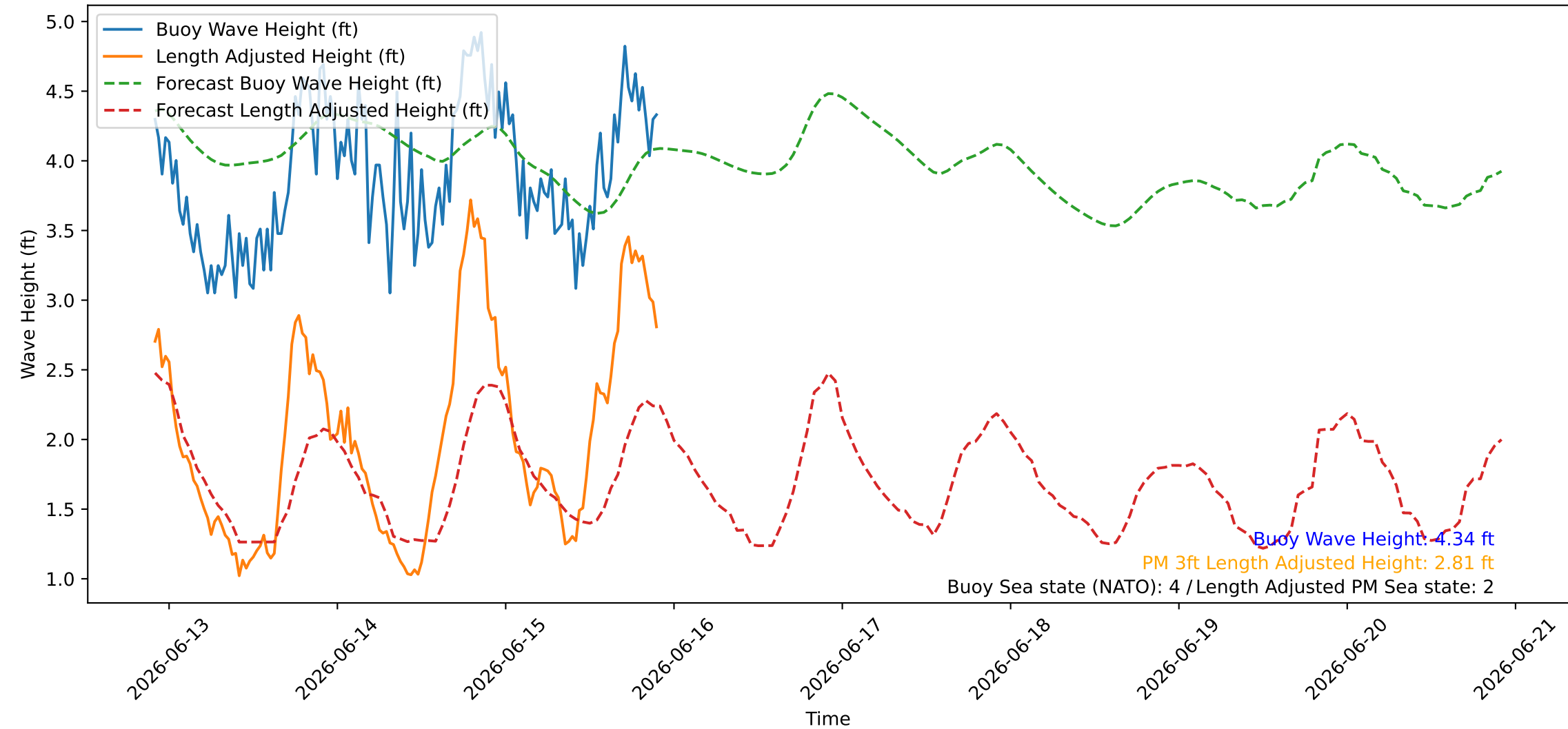
Wave Heights over Time for Green Beach at 2026-06-15 22:11:07
