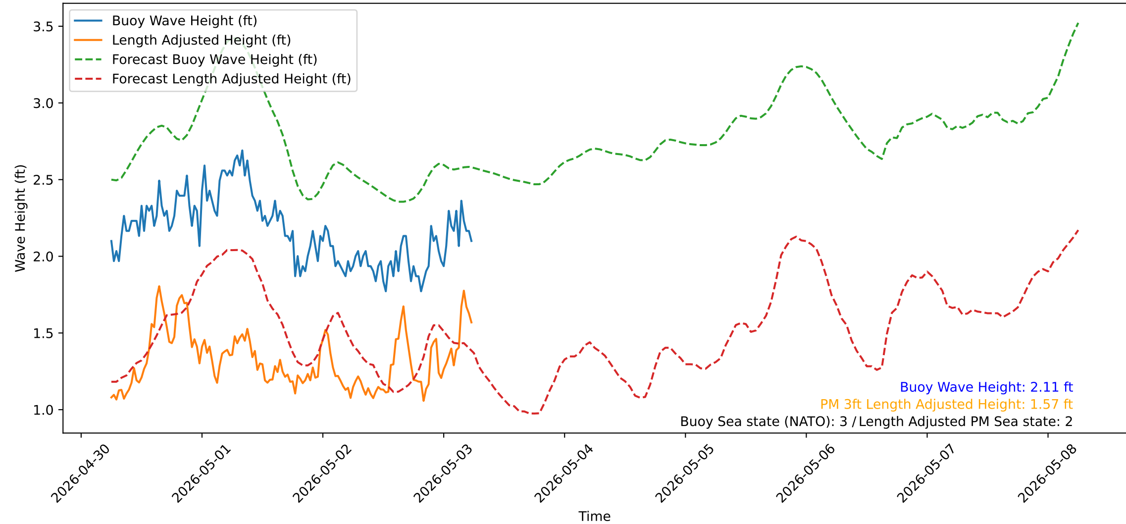
Wave Heights over Time for Oceanside Harbor at 2026-05-03 06:10:31
