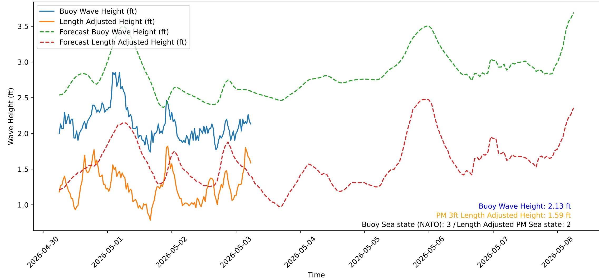
Wave Heights over Time for Green Beach at 2026-05-03 06:11:12
