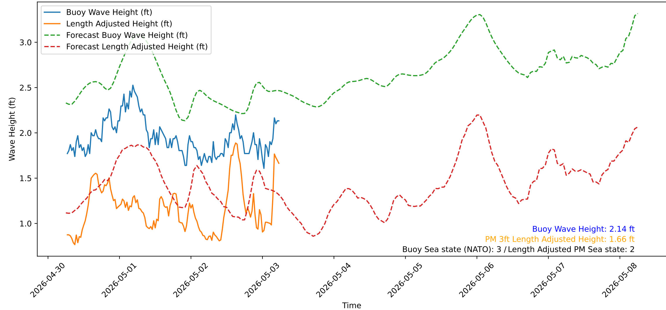
Wave Heights over Time for Red Beach at 2026-05-03 06:10:50
