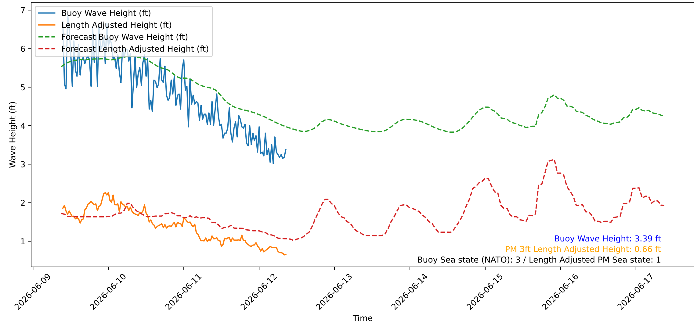
Wave Heights over Time for Green Beach at 2026-06-12 09:21:11
