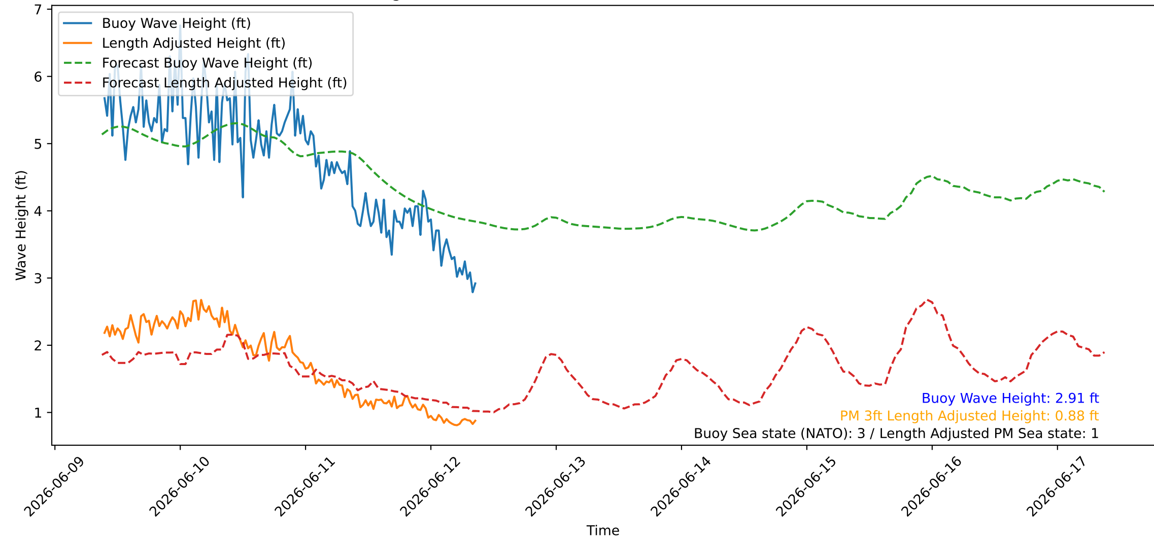
Wave Heights over Time for Oceanside Harbor at 2026-06-12 09:20:26
