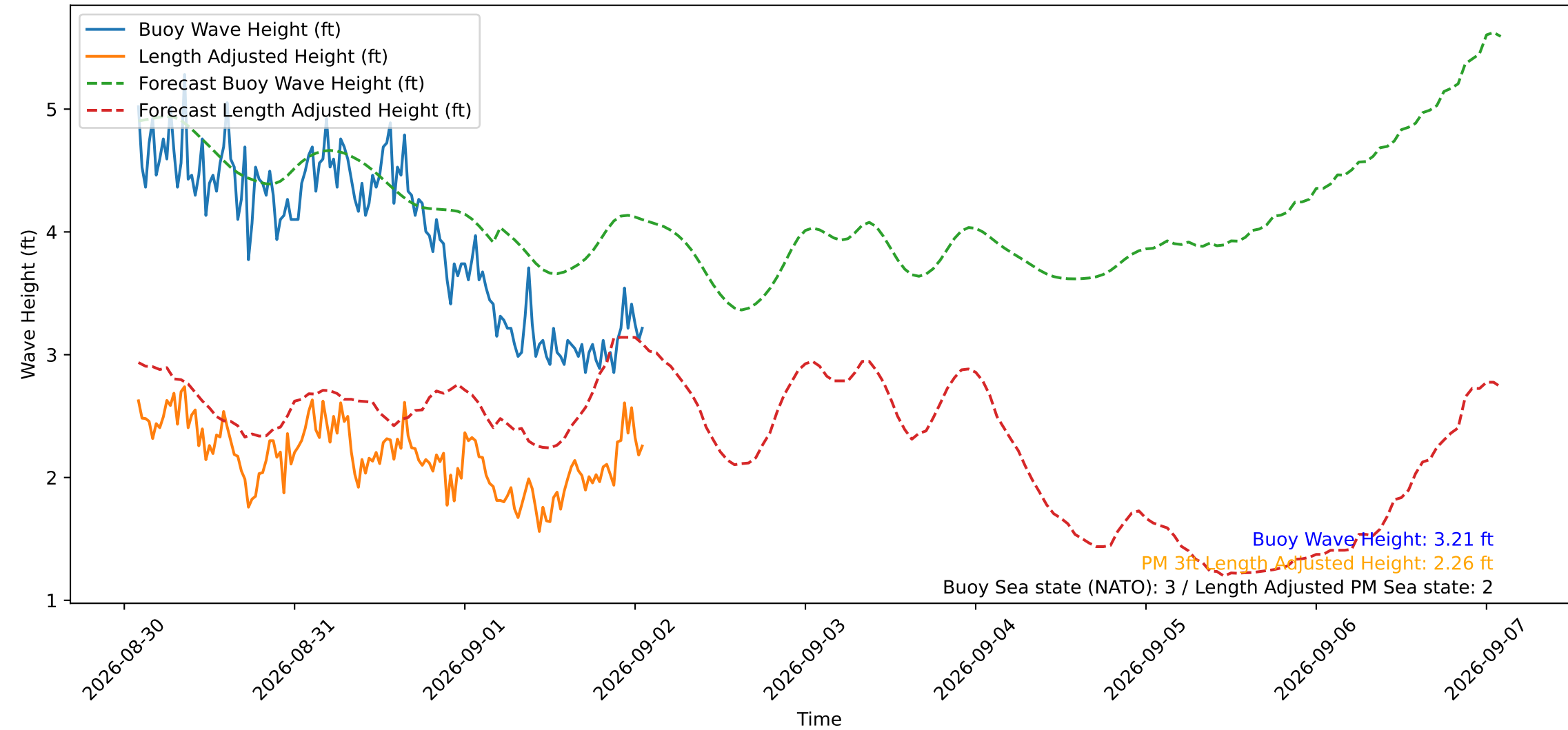
Wave Heights over Time for Oceanside Harbor at 2026-09-02 02:10:29
