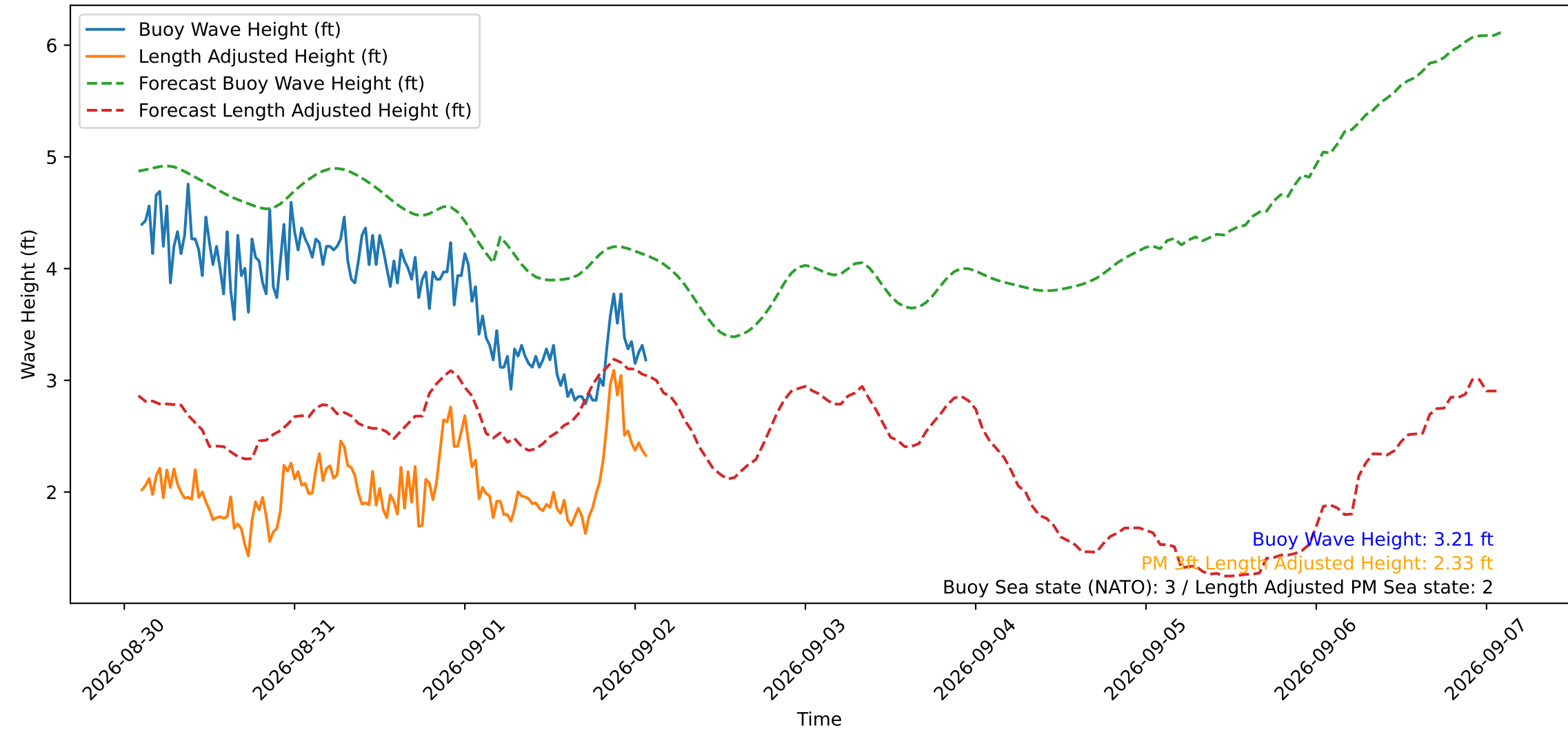
Wave Heights over Time for Green Beach at 2026-09-02 02:11:12
