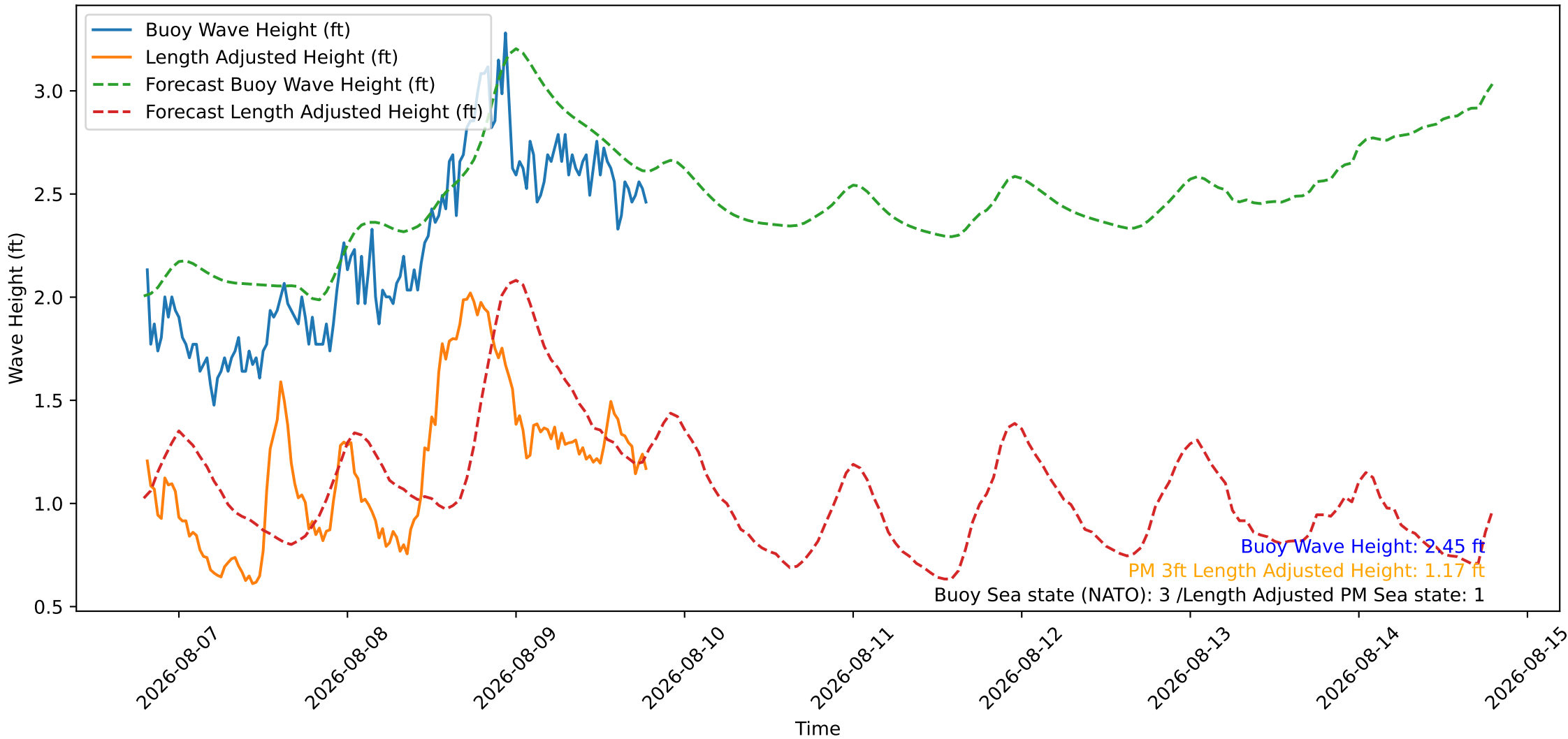
Wave Heights over Time for Red Beach at 2026-08-09 19:20:47
