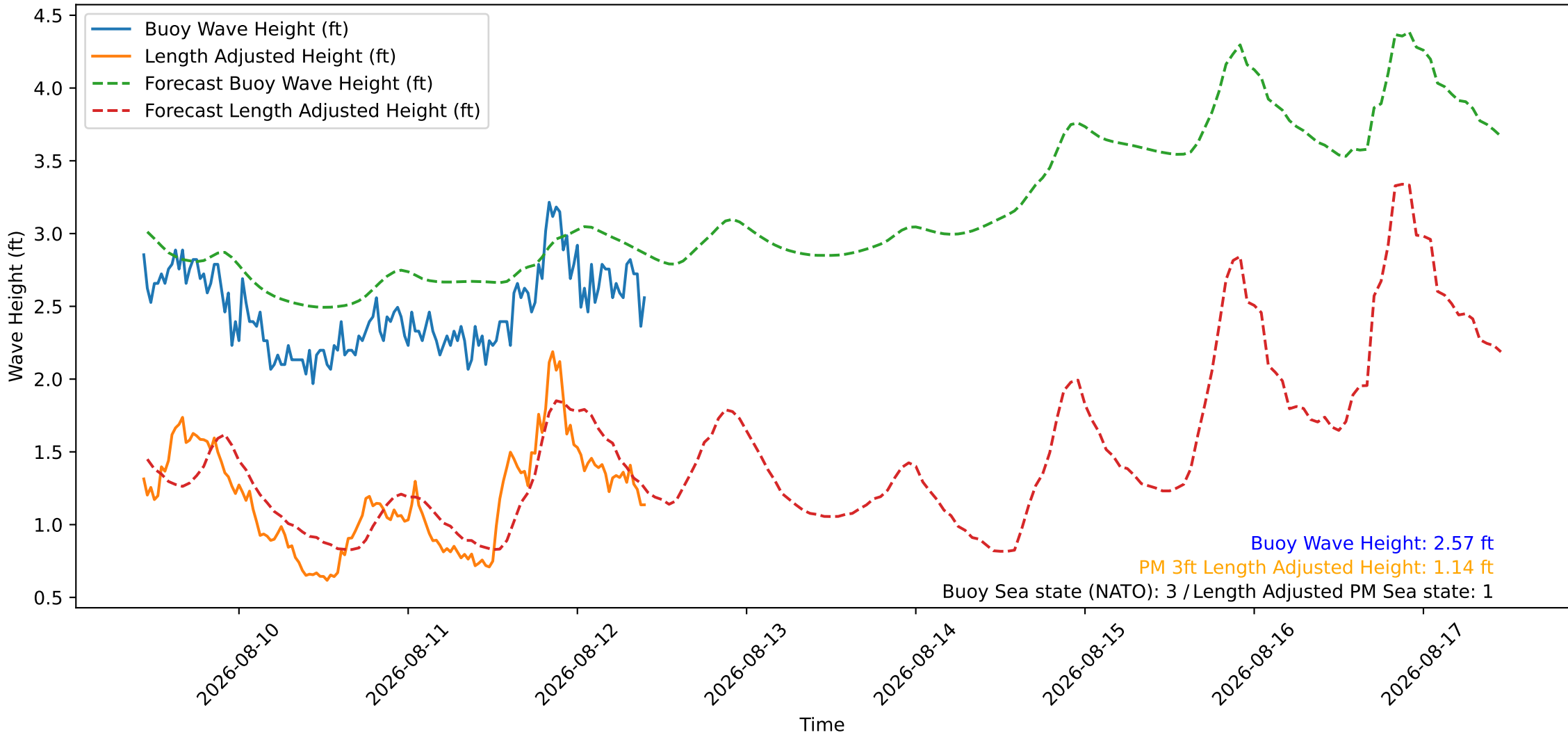
Wave Heights over Time for Green Beach at 2026-08-12 10:31:09
