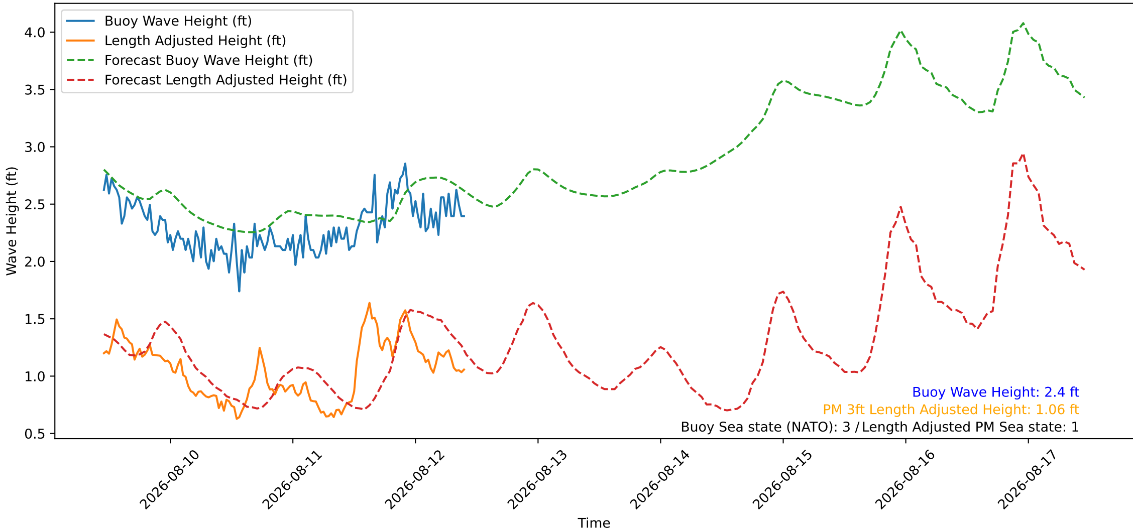
Wave Heights over Time for Red Beach at 2026-08-12 10:30:46
