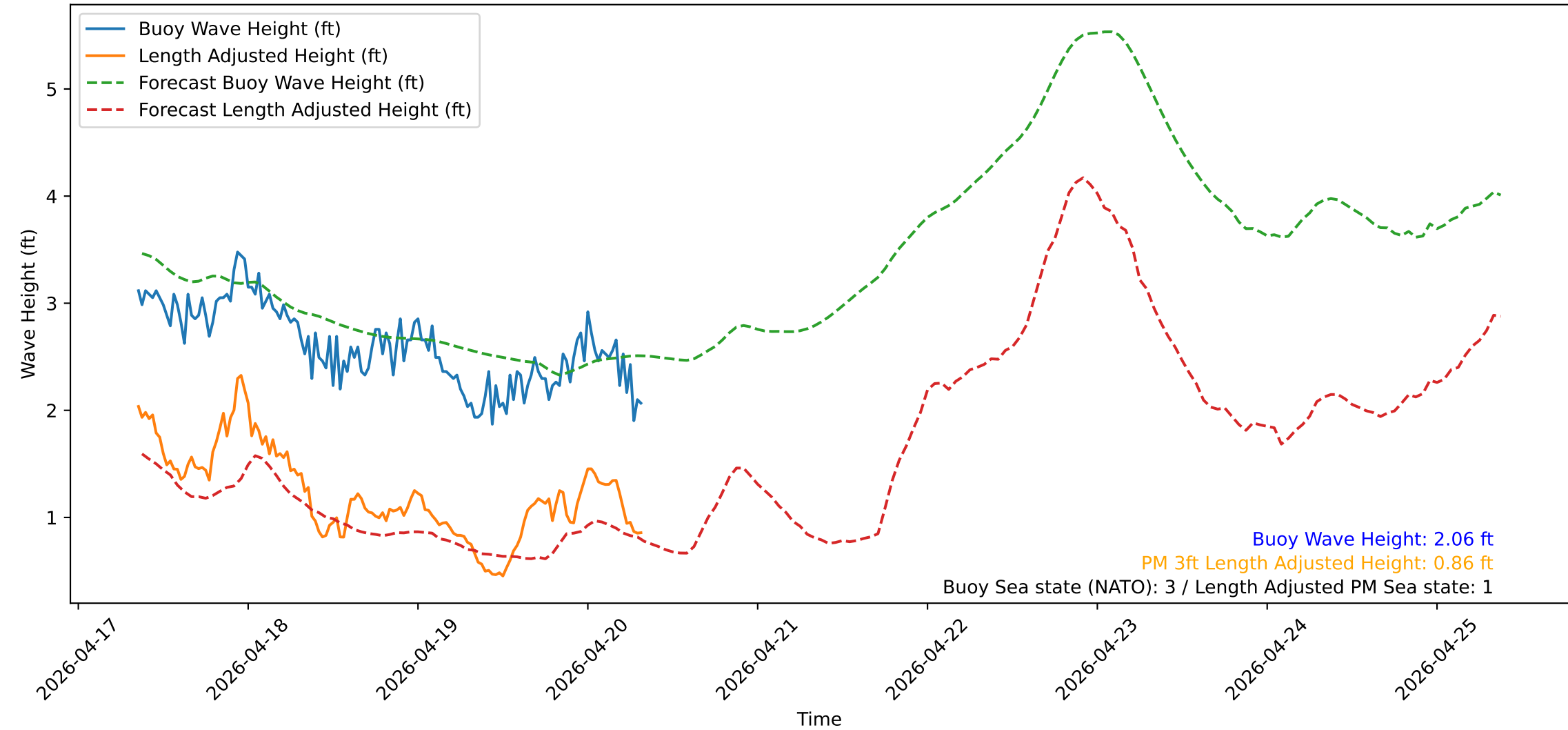
Wave Heights over Time for Green Beach at 2026-04-20 08:31:14
