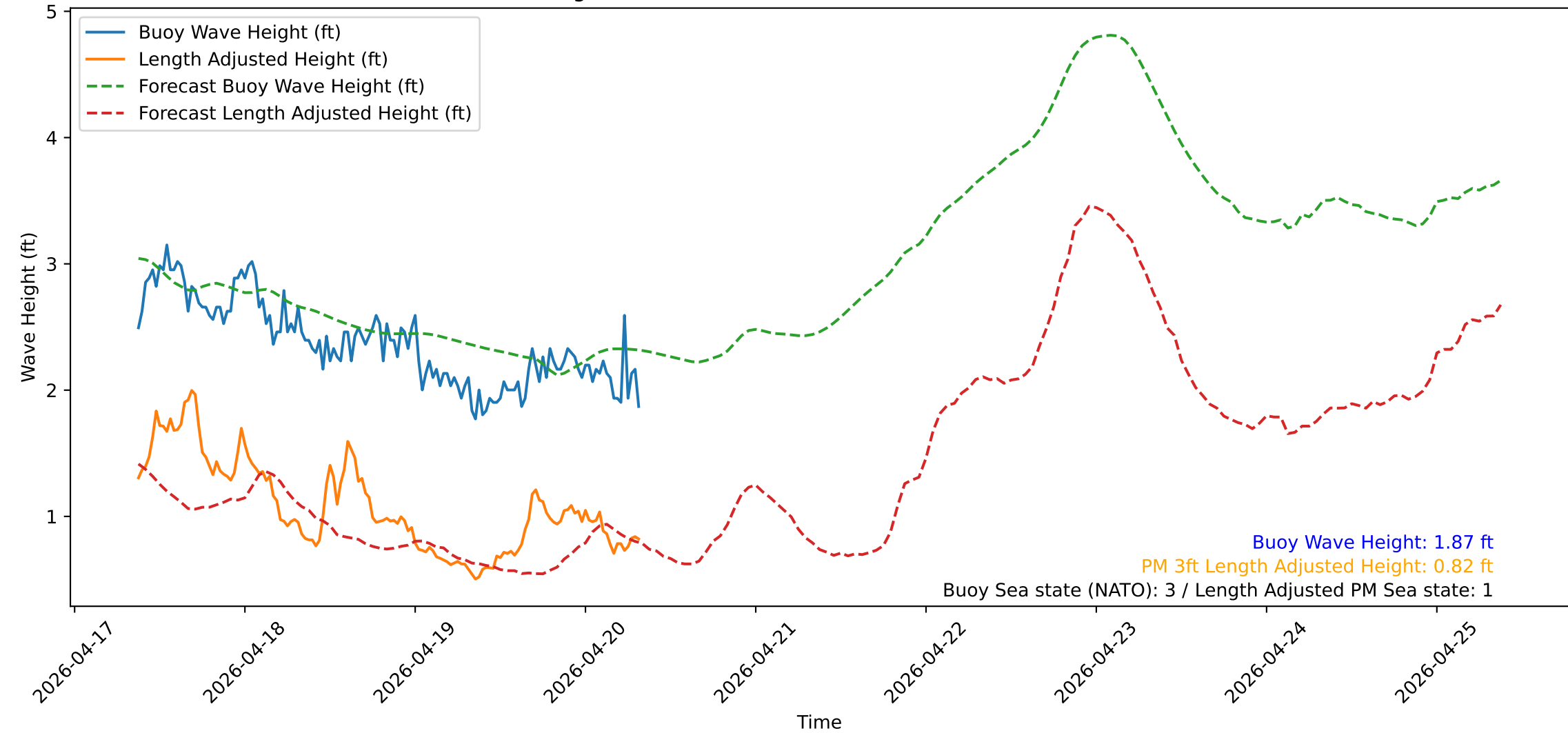
Wave Heights over Time for Red Beach at 2026-04-20 08:30:51
