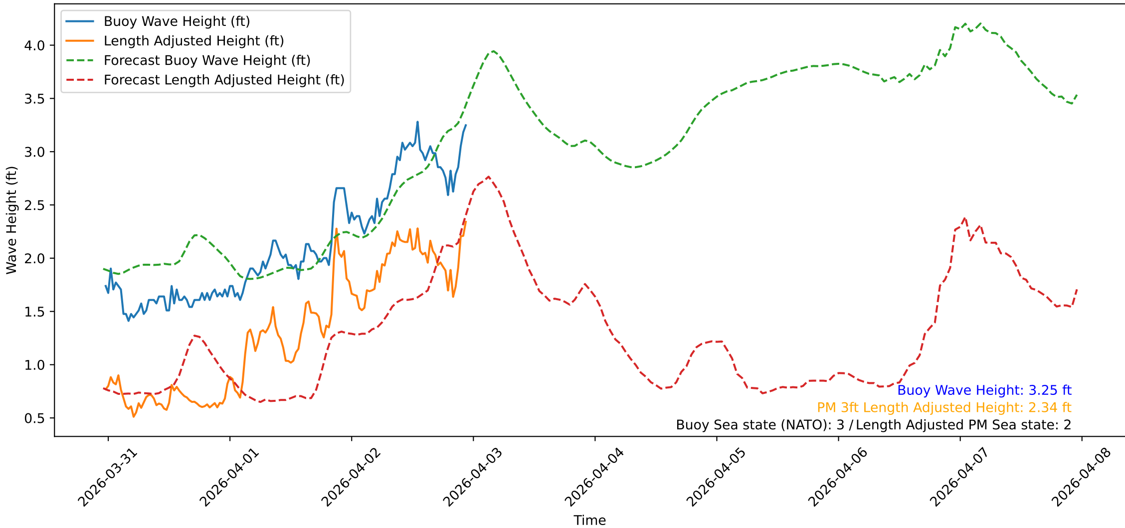
Wave Heights over Time for Green Beach at 2026-04-02 23:21:09
