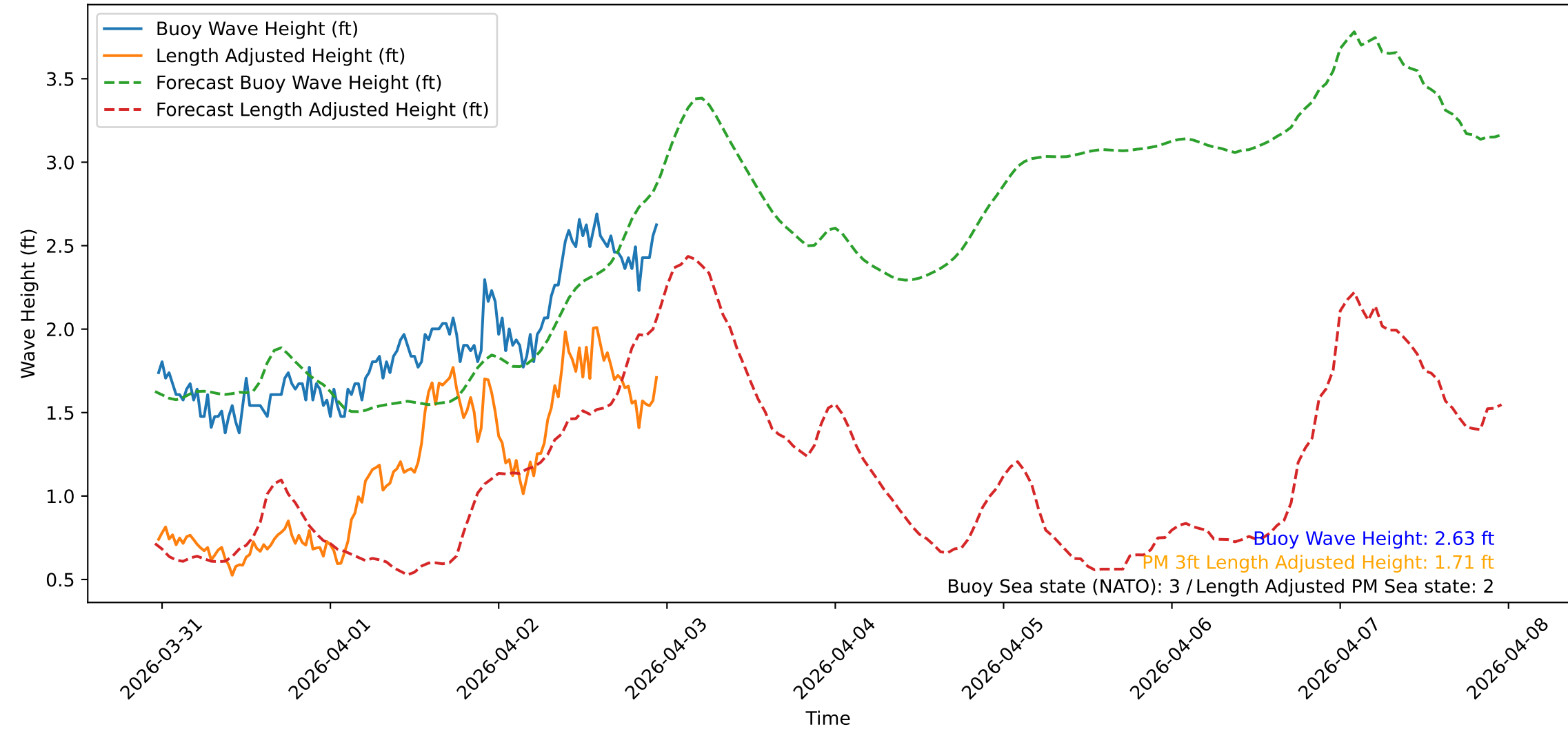
Wave Heights over Time for Red Beach at 2026-04-02 23:20:47
