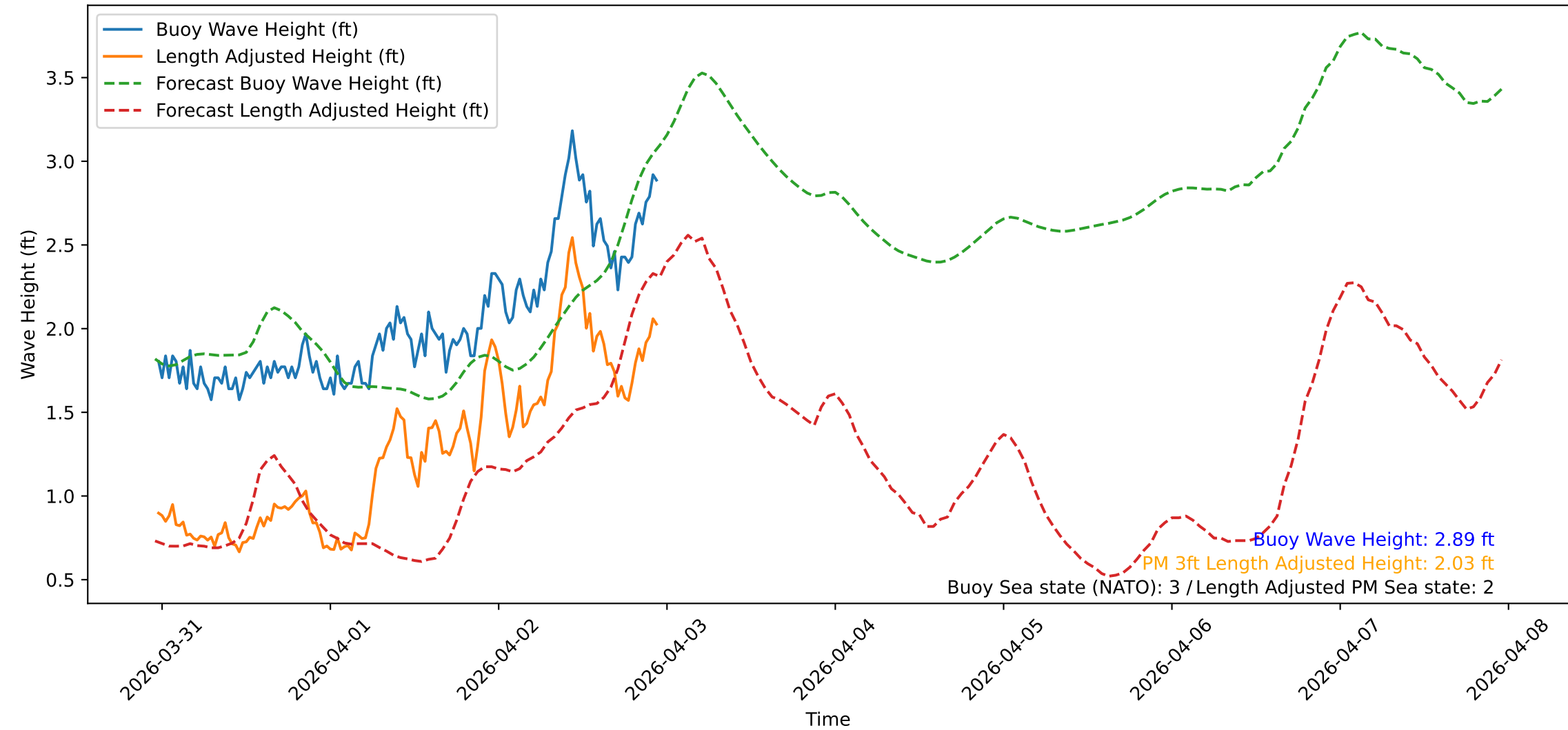
Wave Heights over Time for Oceanside Harbor at 2026-04-02 23:20:31
