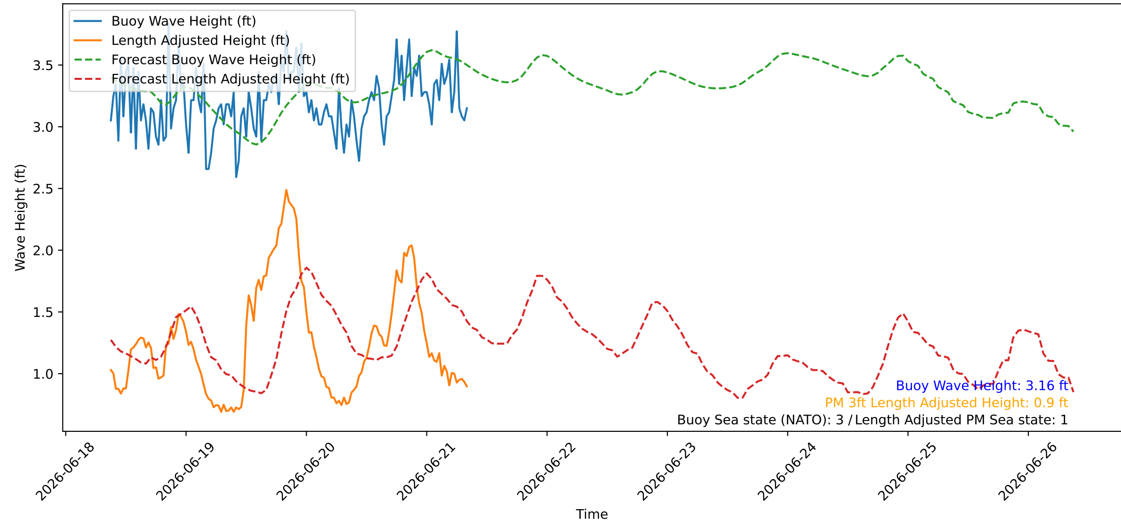
Wave Heights over Time for Red Beach at 2026-06-21 08:50:47
