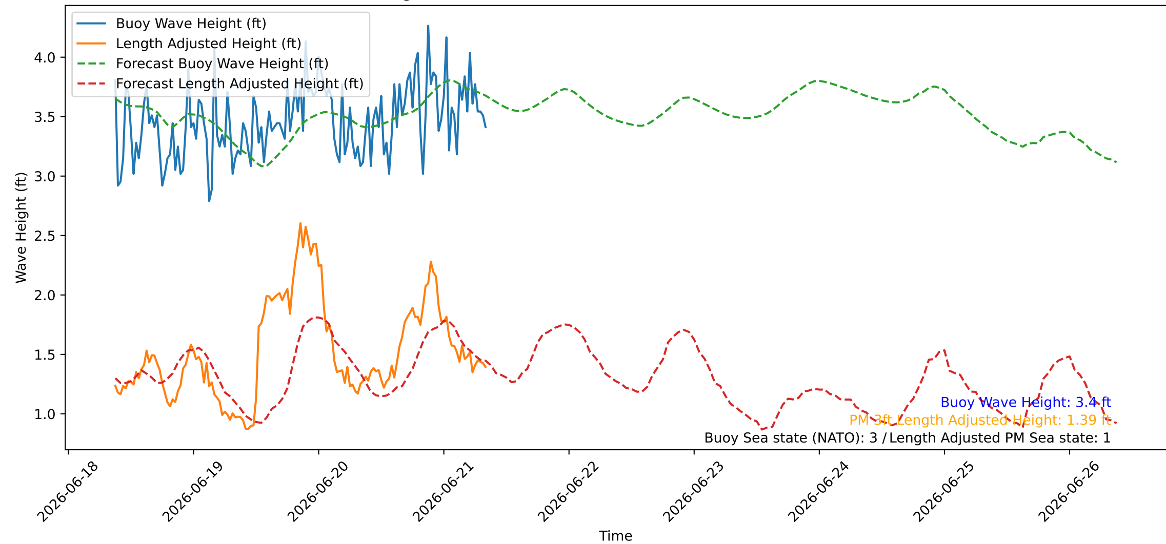
Wave Heights over Time for Oceanside Harbor at 2026-06-21 08:50:26
