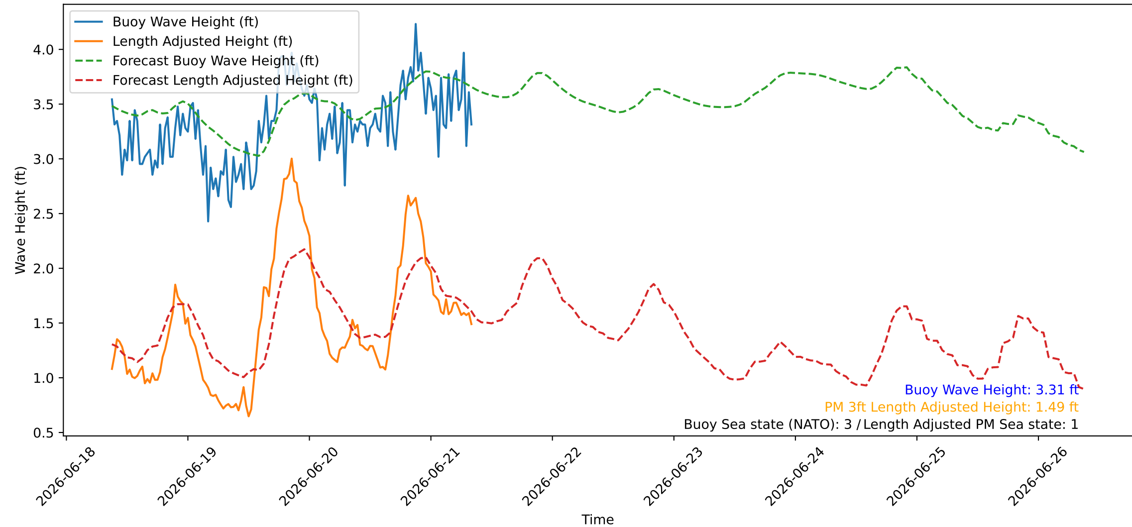
Wave Heights over Time for Green Beach at 2026-06-21 08:51:09
