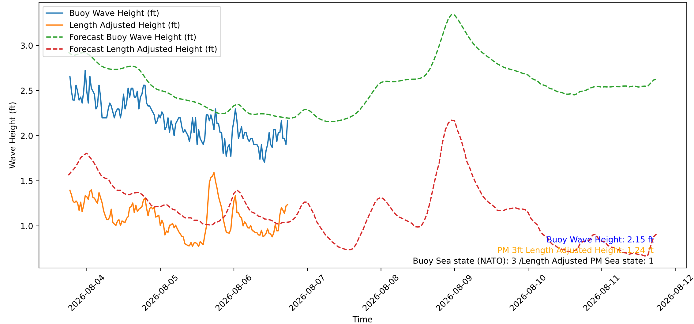
Wave Heights over Time for Oceanside Harbor at 2026-08-06 18:20:26
