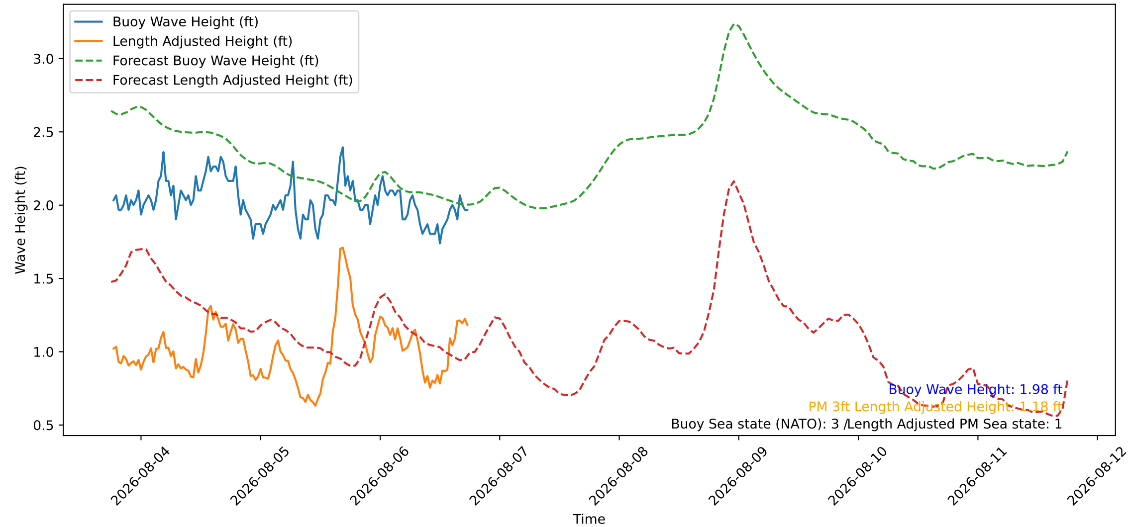
Wave Heights over Time for Red Beach at 2026-08-06 18:20:47
