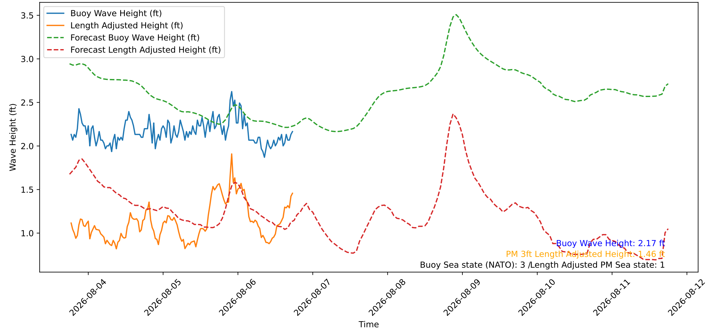
Wave Heights over Time for Green Beach at 2026-08-06 18:21:09
