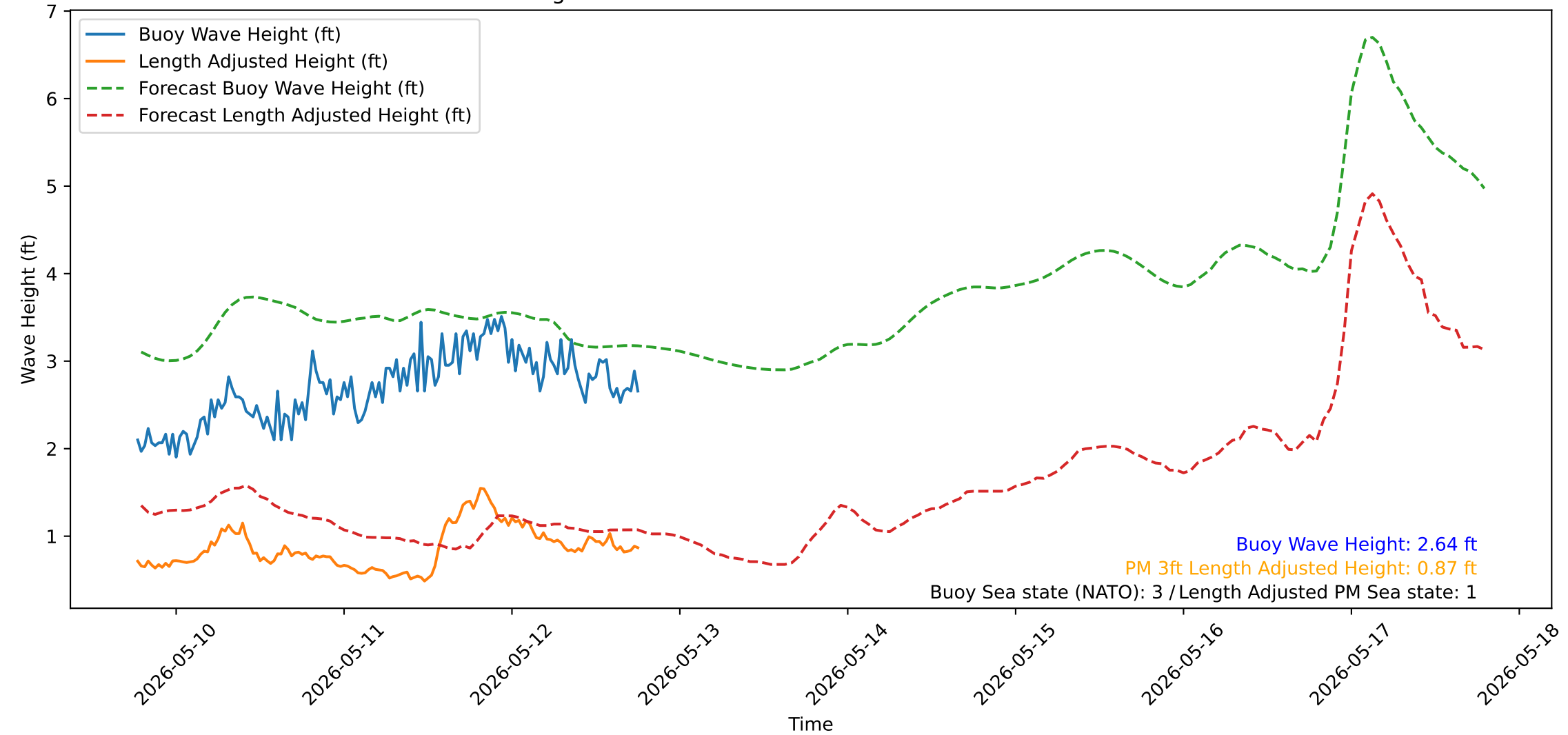
Wave Heights over Time for Green Beach at 2026-05-12 18:41:14
