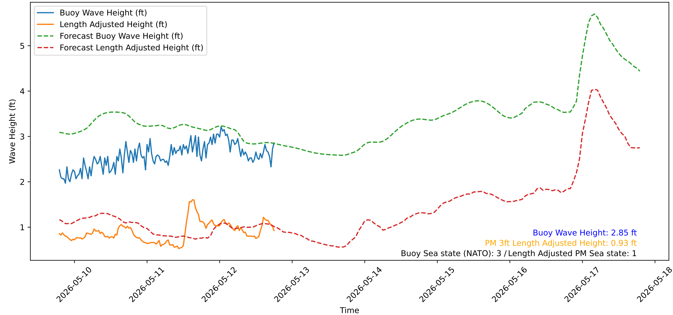
Wave Heights over Time for Red Beach at 2026-05-12 18:40:51
