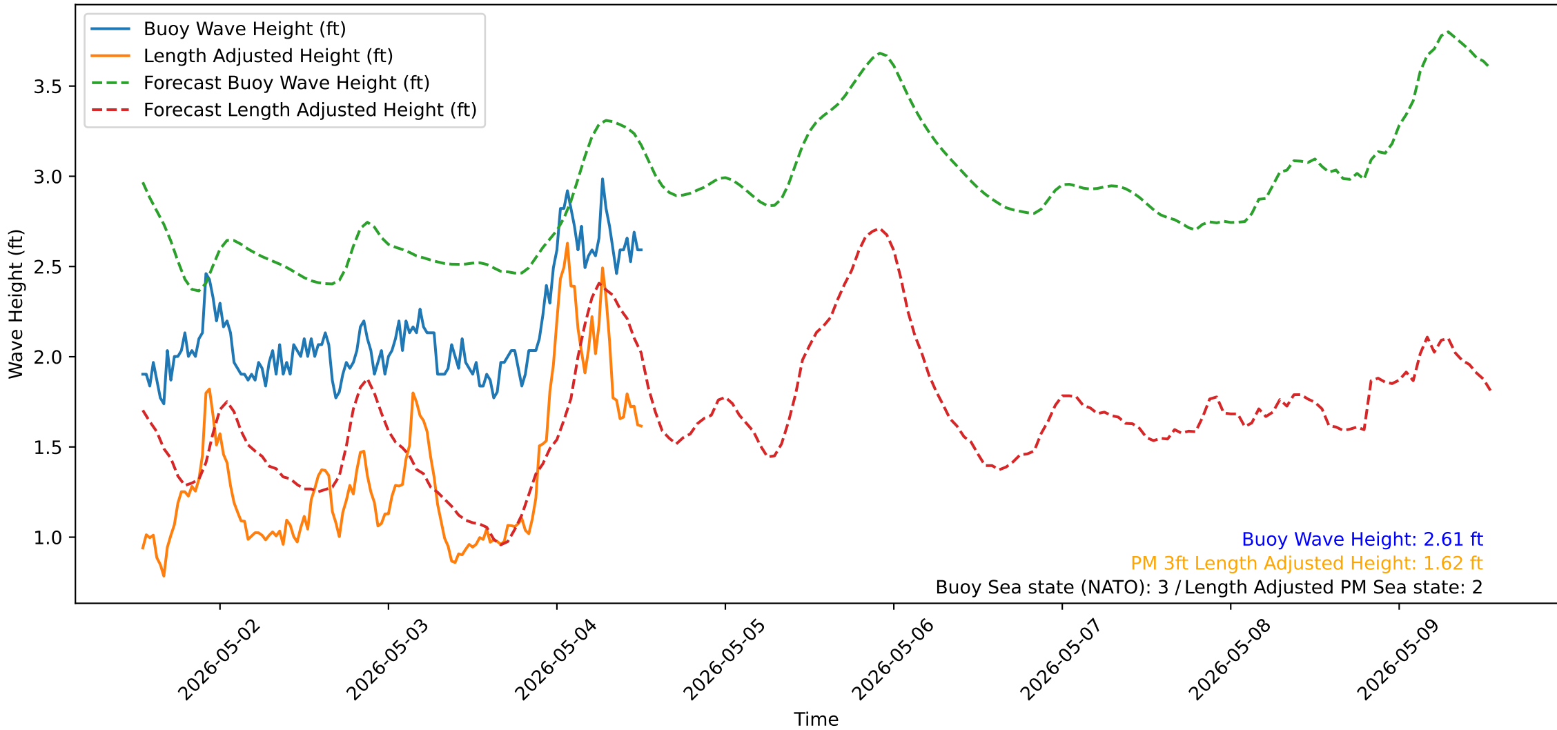
Wave Heights over Time for Green Beach at 2026-05-04 12:51:13
