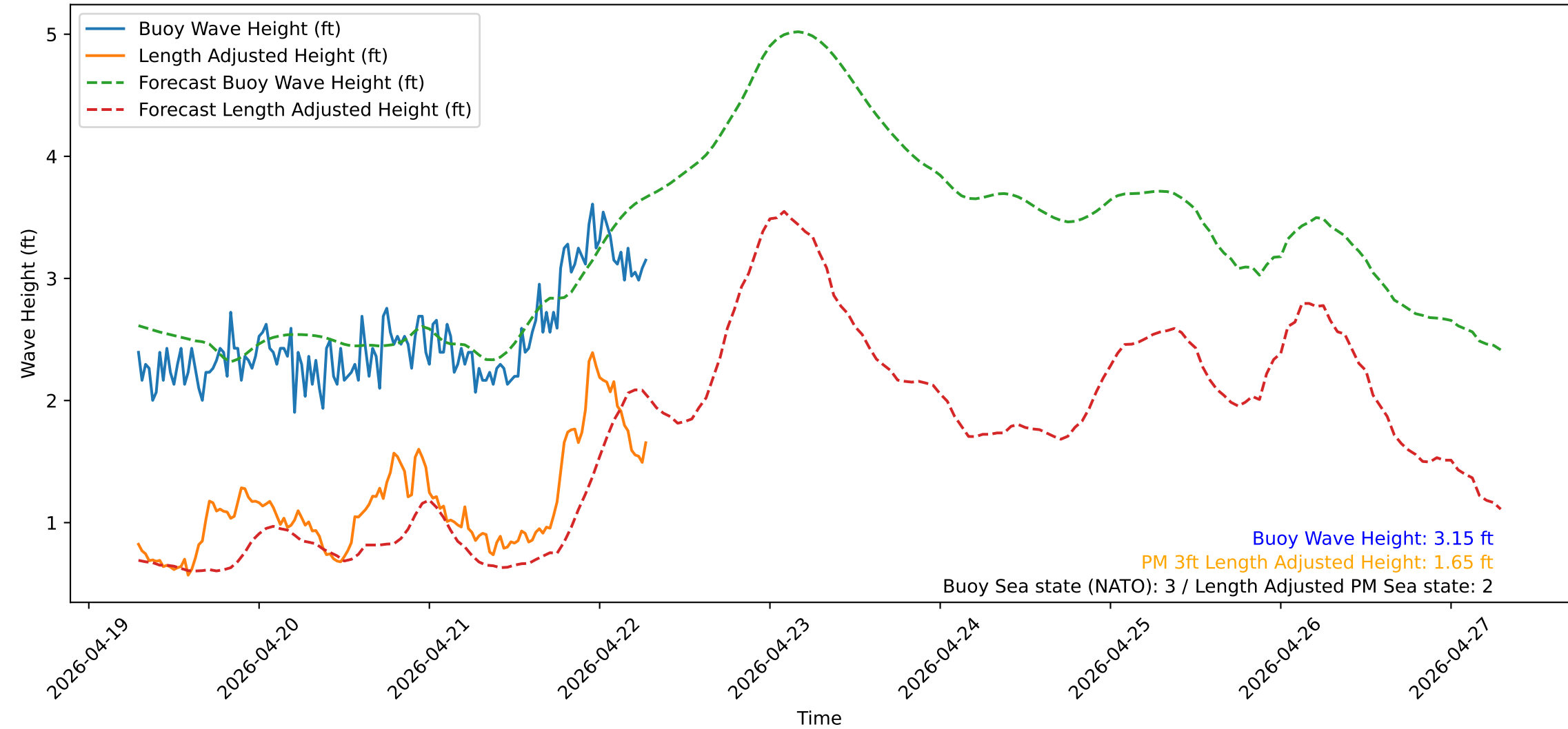
Wave Heights over Time for Oceanside Harbor at 2026-04-22 07:00:32
