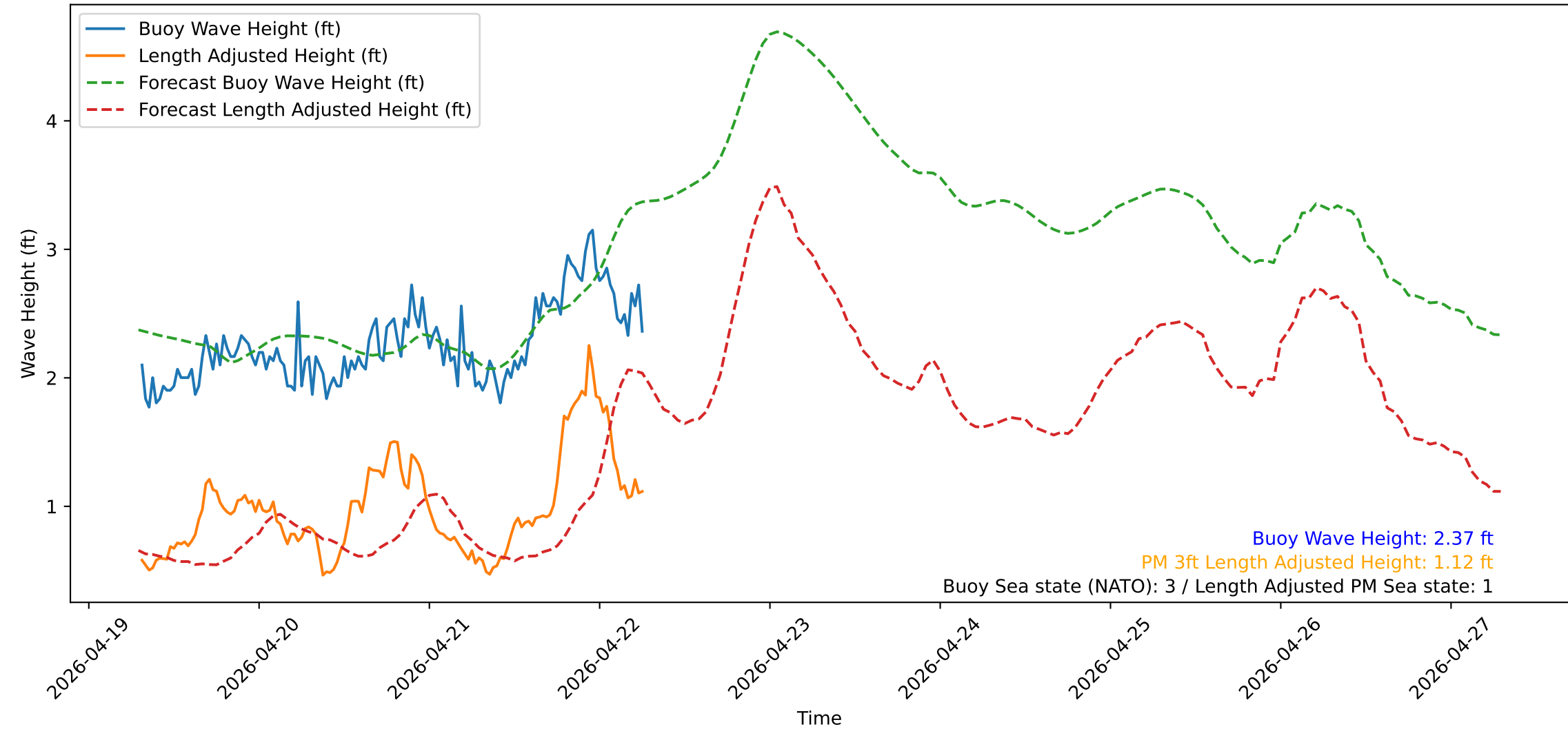
Wave Heights over Time for Red Beach at 2026-04-22 07:00:51
