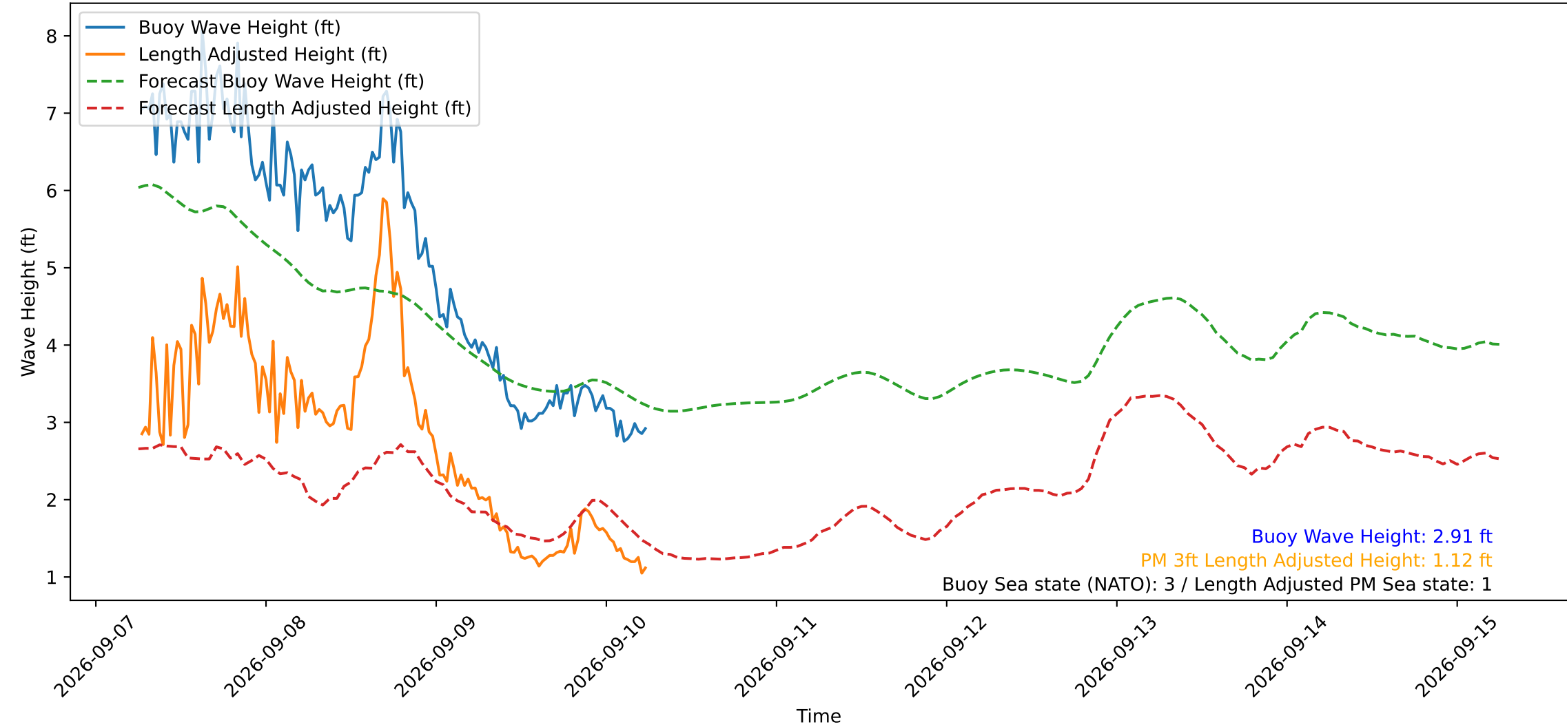
Wave Heights over Time for Green Beach at 2026-09-10 06:11:12
