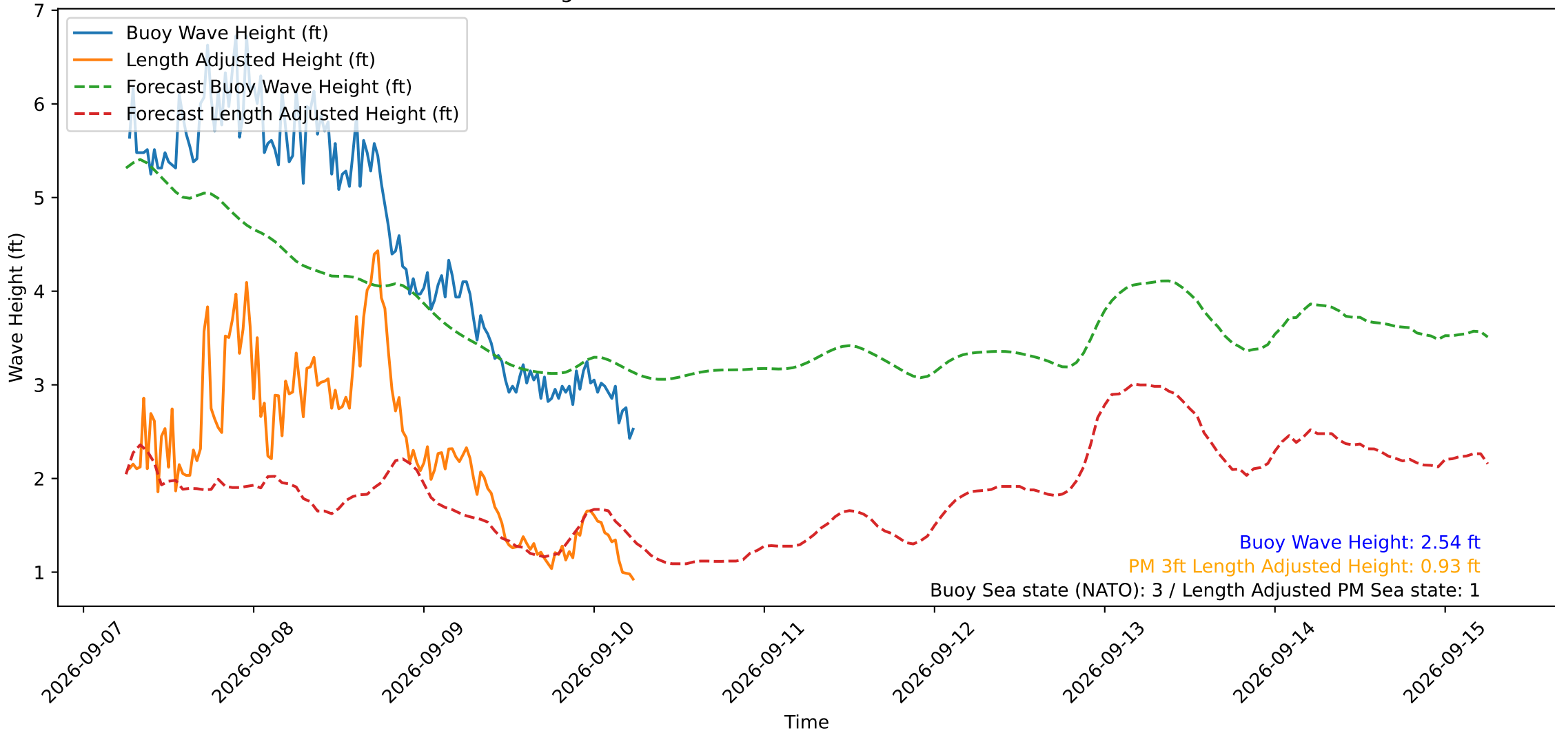
Wave Heights over Time for Red Beach at 2026-09-10 06:10:50
