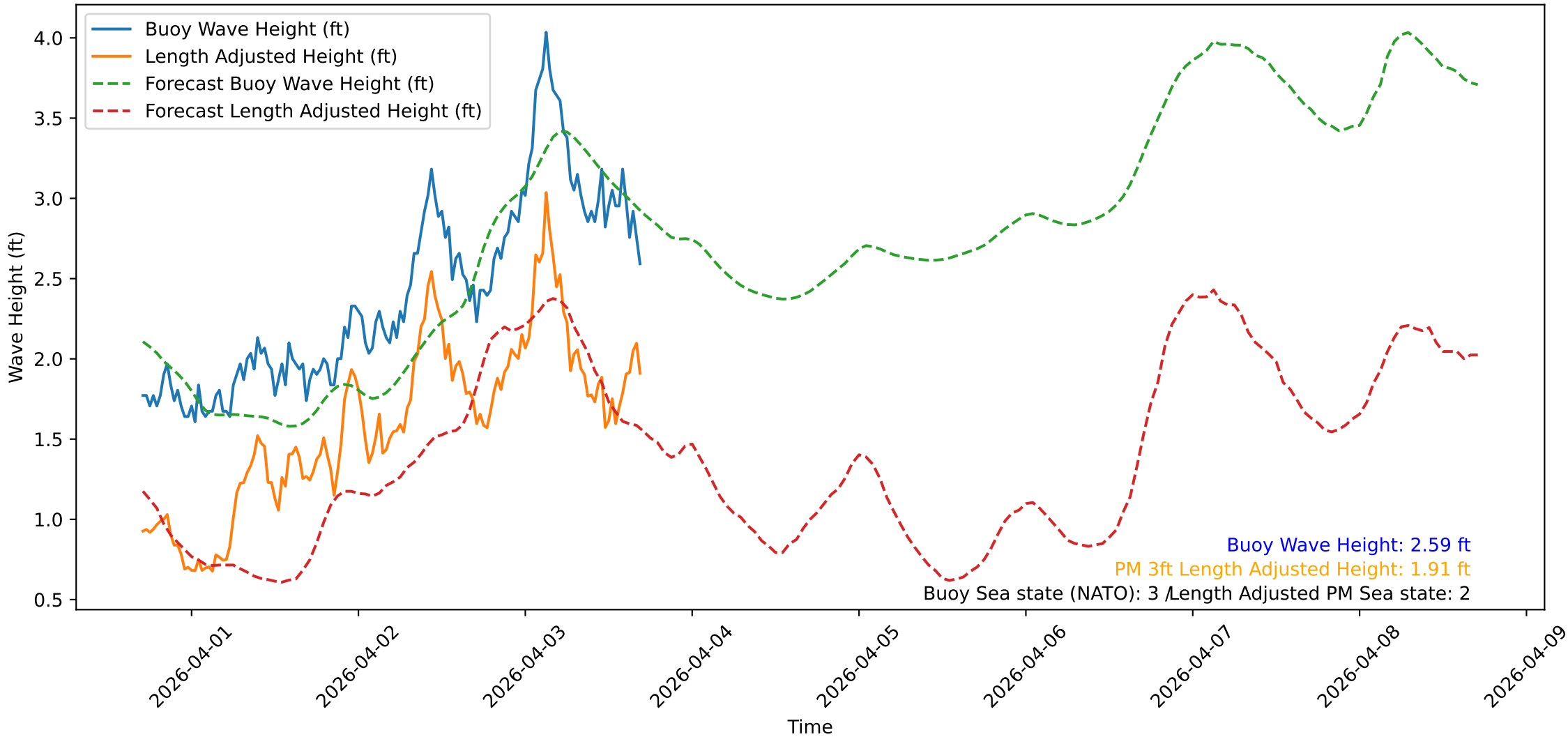
Wave Heights over Time for Oceanside Harbor at 2026-04-03 17:10:32
