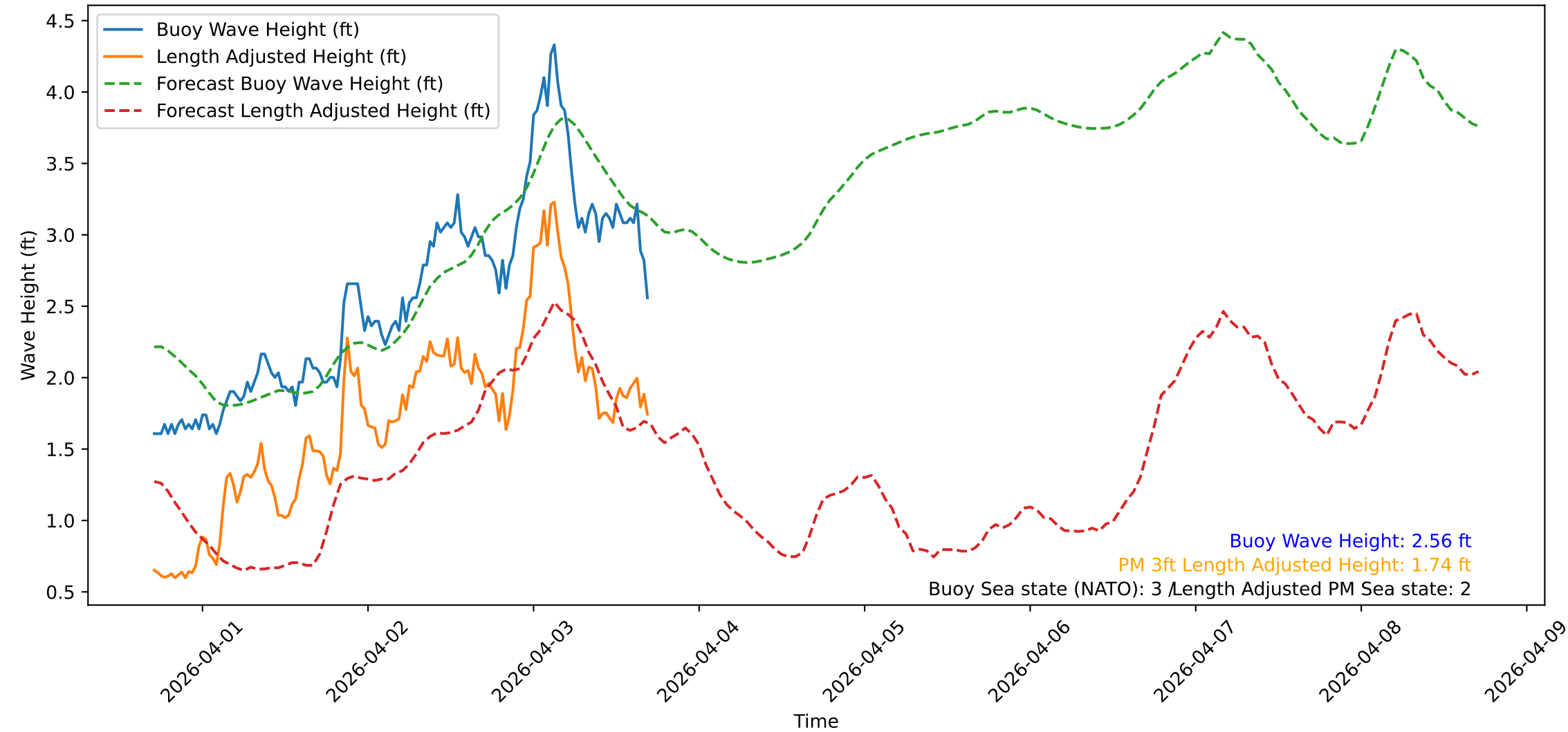
Wave Heights over Time for Green Beach at 2026-04-03 17:11:12
