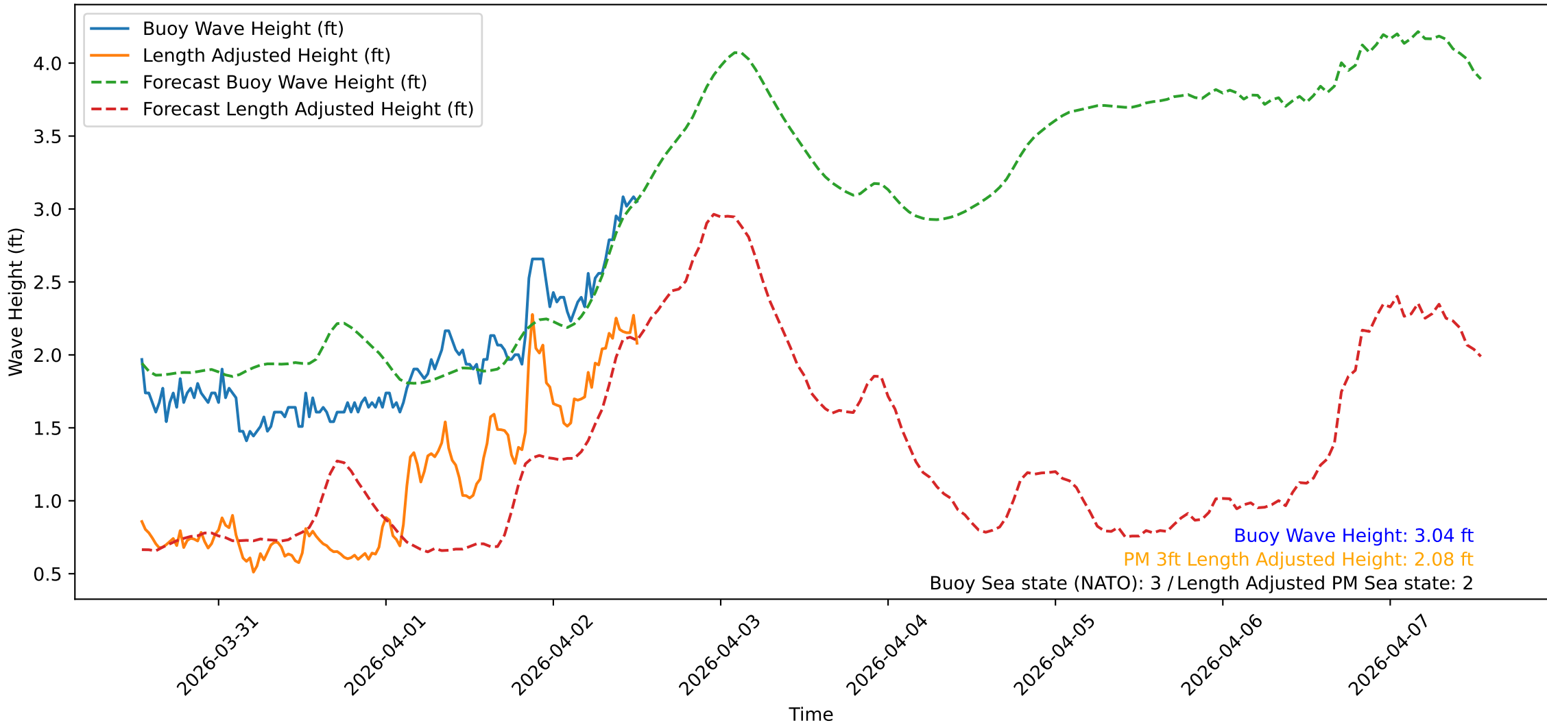
Wave Heights over Time for Green Beach at 2026-04-02 13:01:09
