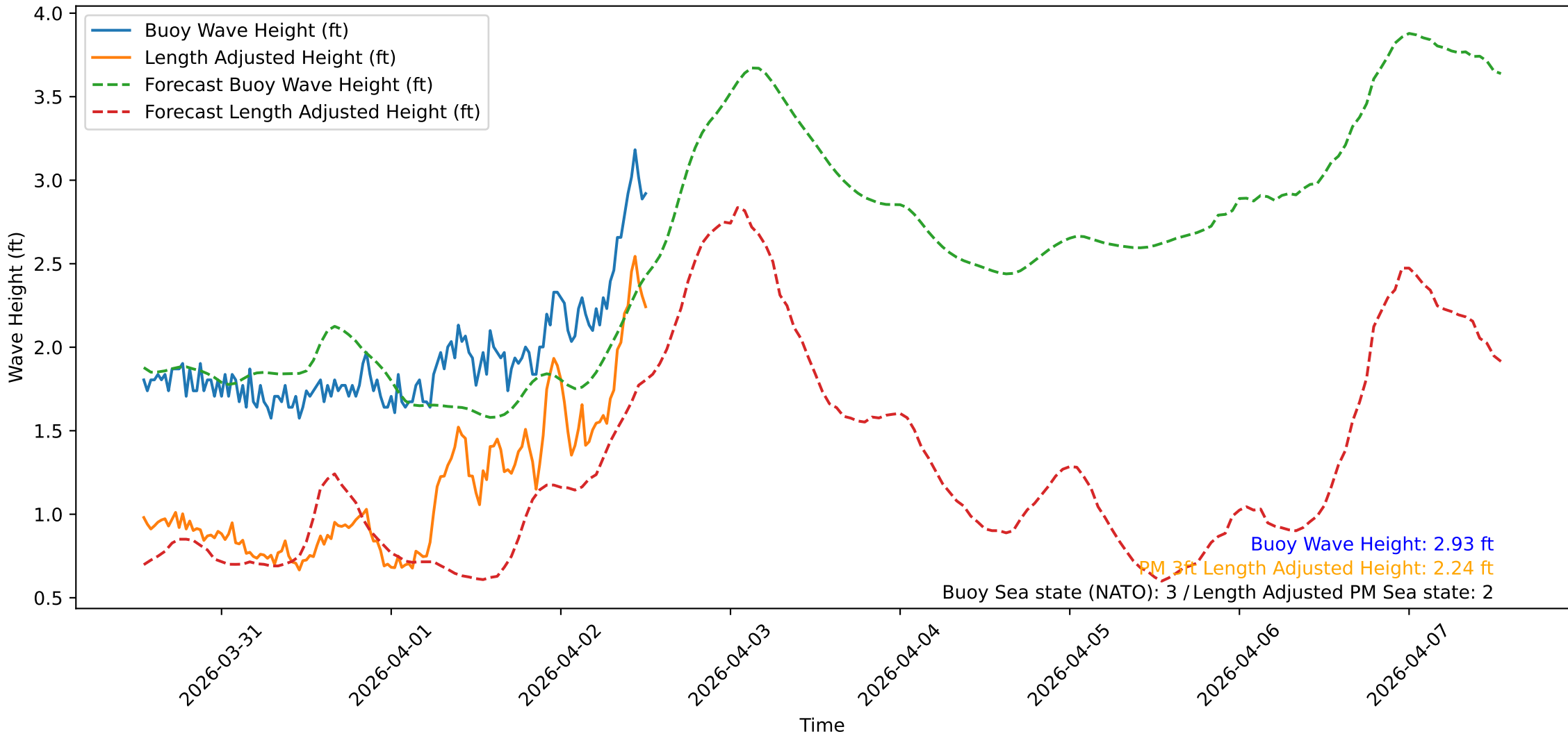
Wave Heights over Time for Oceanside Harbor at 2026-04-02 13:00:31
