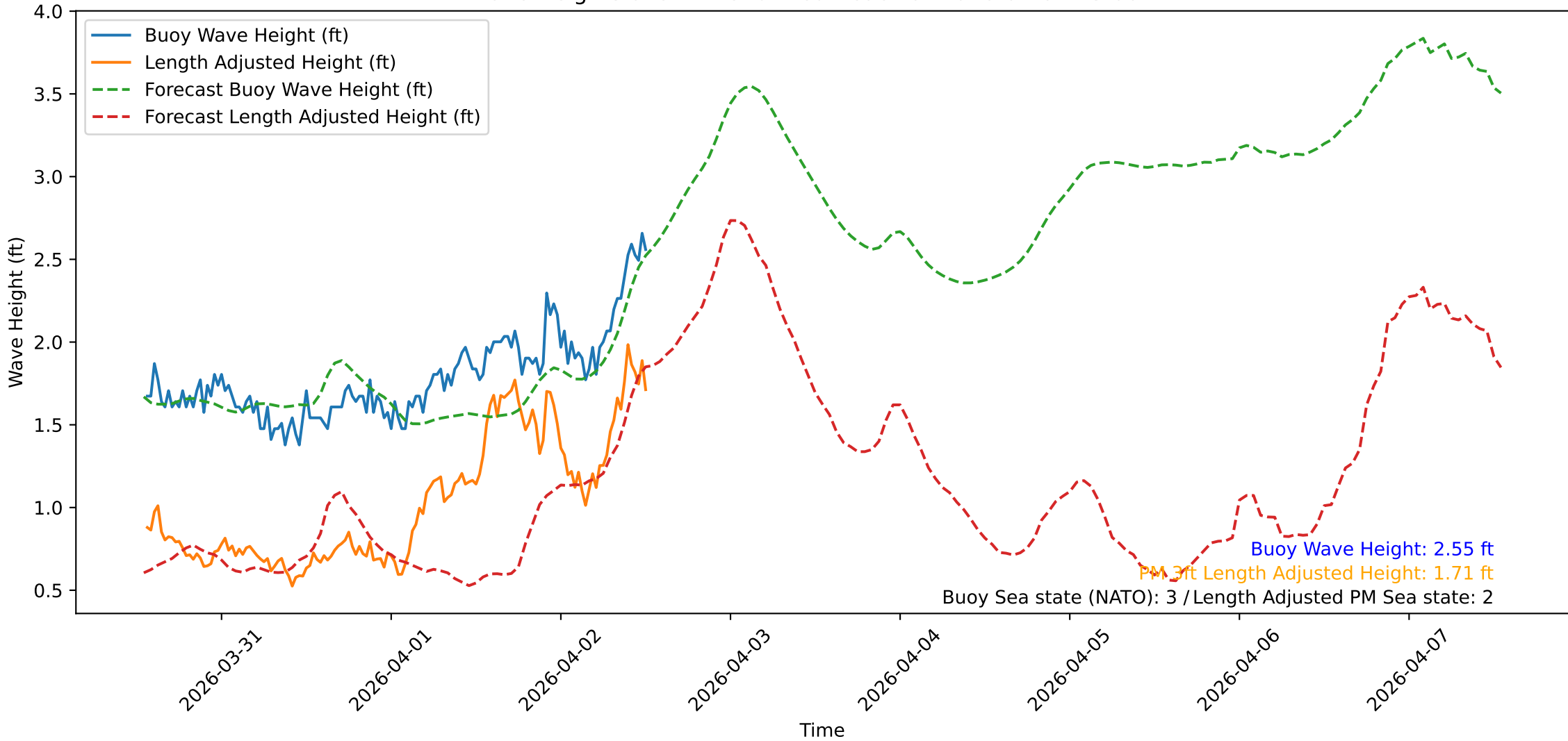
Wave Heights over Time for Red Beach at 2026-04-02 13:00:47
