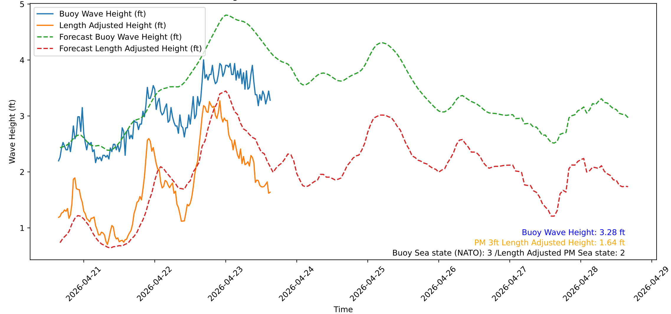
Wave Heights over Time for Green Beach at 2026-04-23 15:41:13
