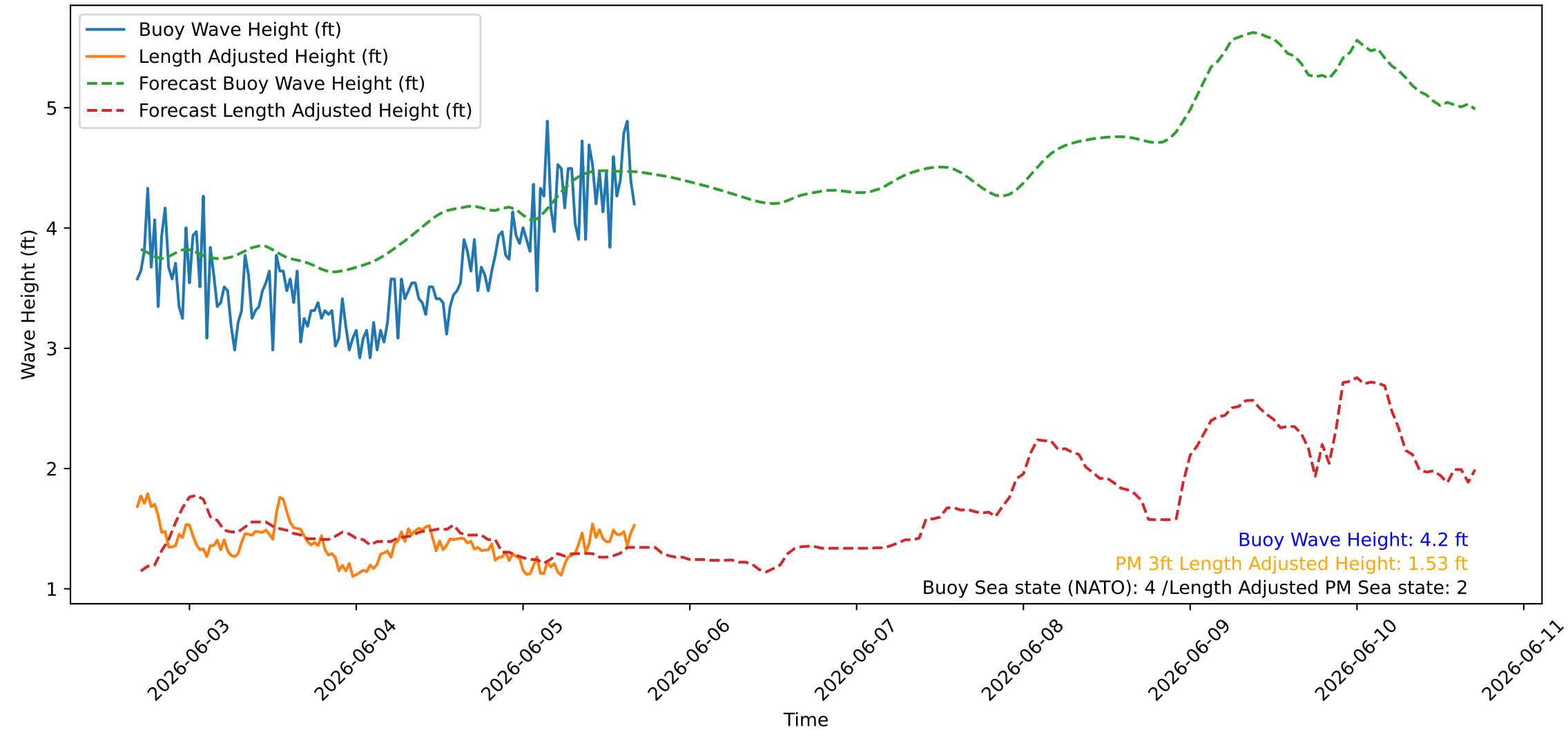
Wave Heights over Time for Oceanside Harbor at 2026-06-05 16:30:26
