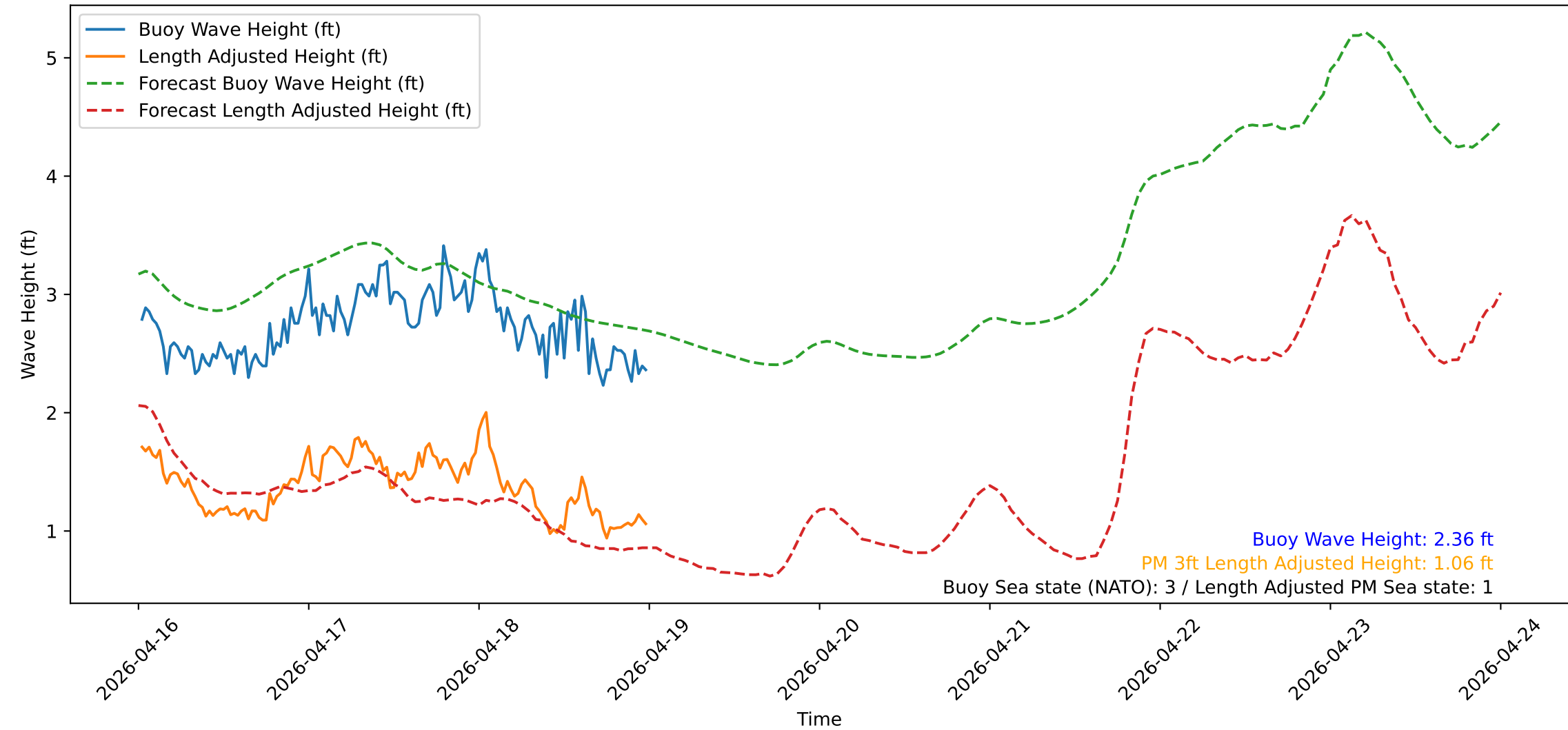
Wave Heights over Time for Oceanside Harbor at 2026-04-19 00:20:31
