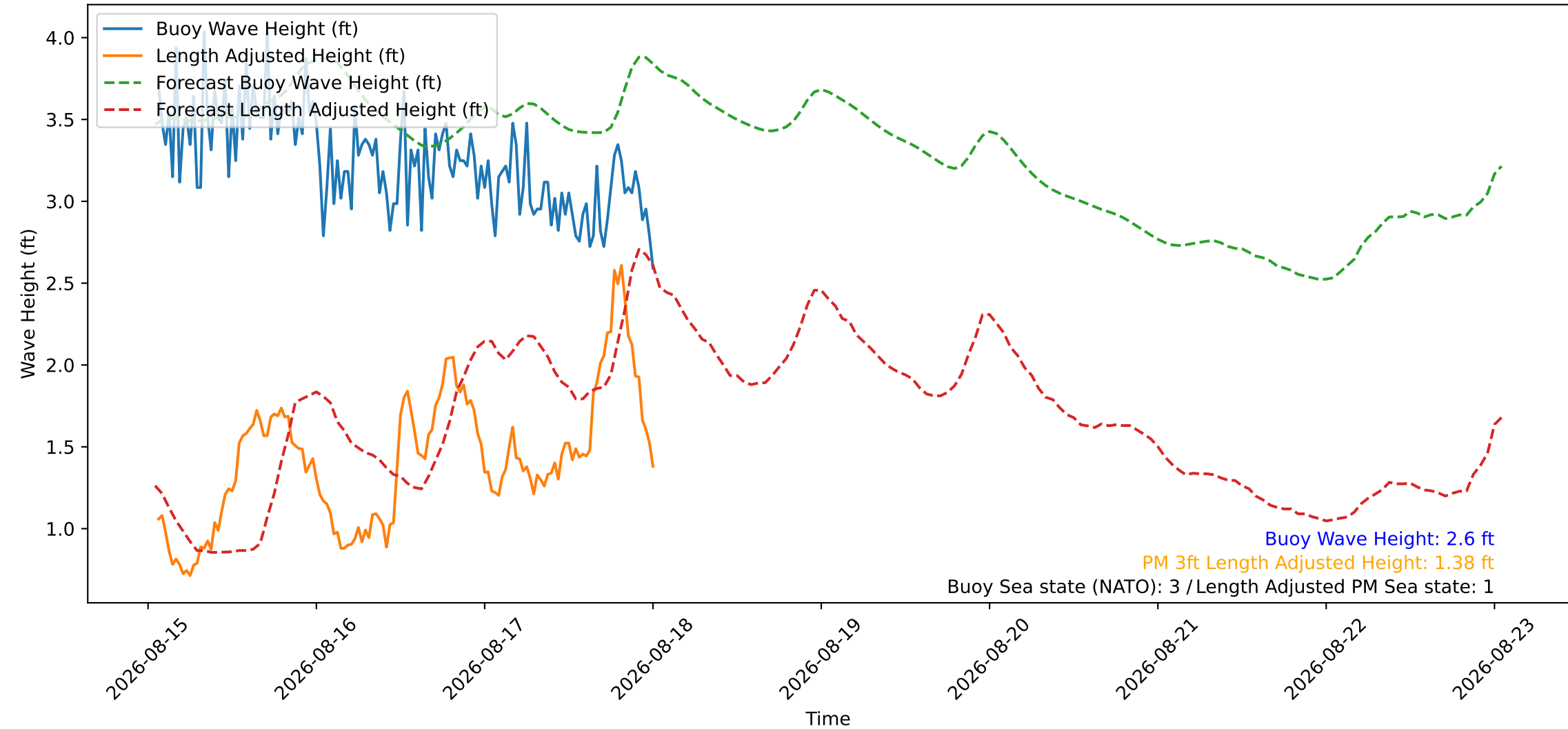
Wave Heights over Time for Red Beach at 2026-08-18 01:00:46
