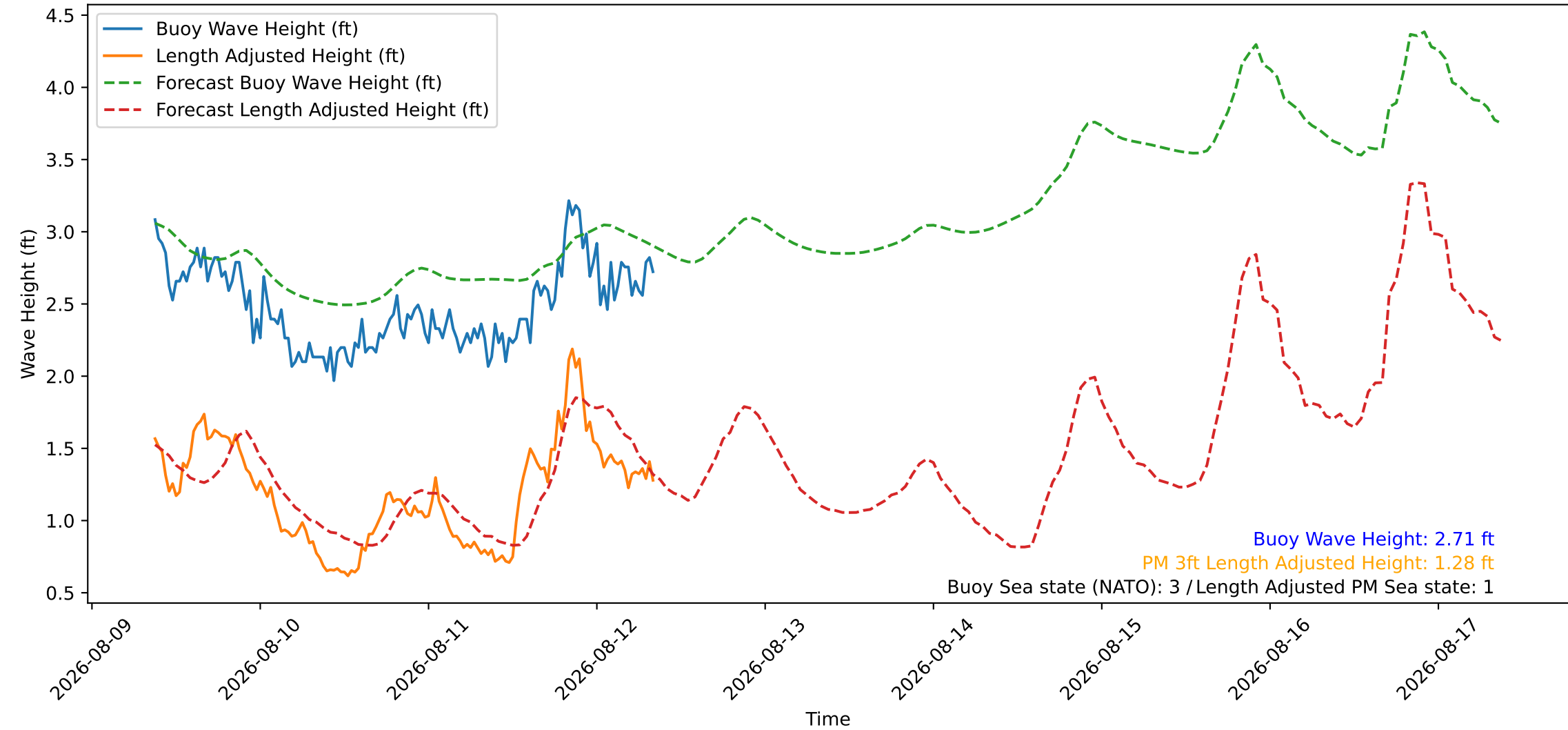
Wave Heights over Time for Green Beach at 2026-08-12 09:01:10
