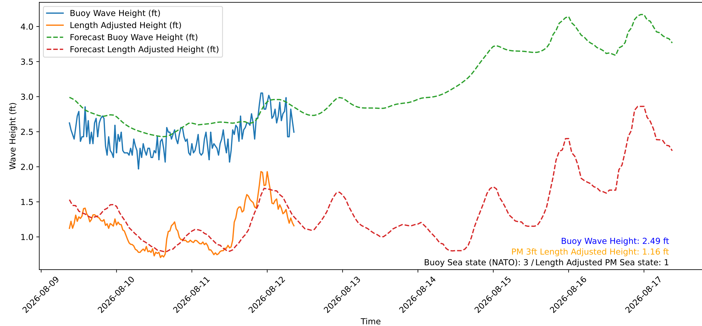
Wave Heights over Time for Oceanside Harbor at 2026-08-12 09:00:27
