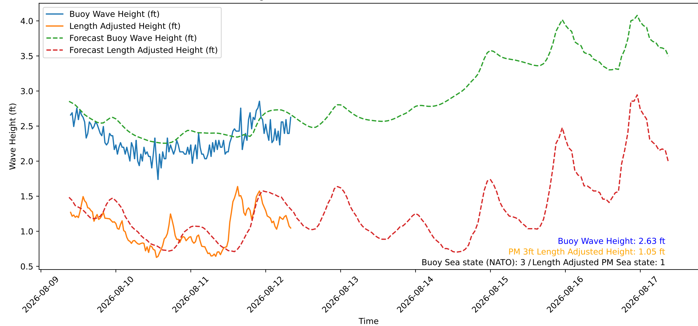
Wave Heights over Time for Red Beach at 2026-08-12 09:00:46
