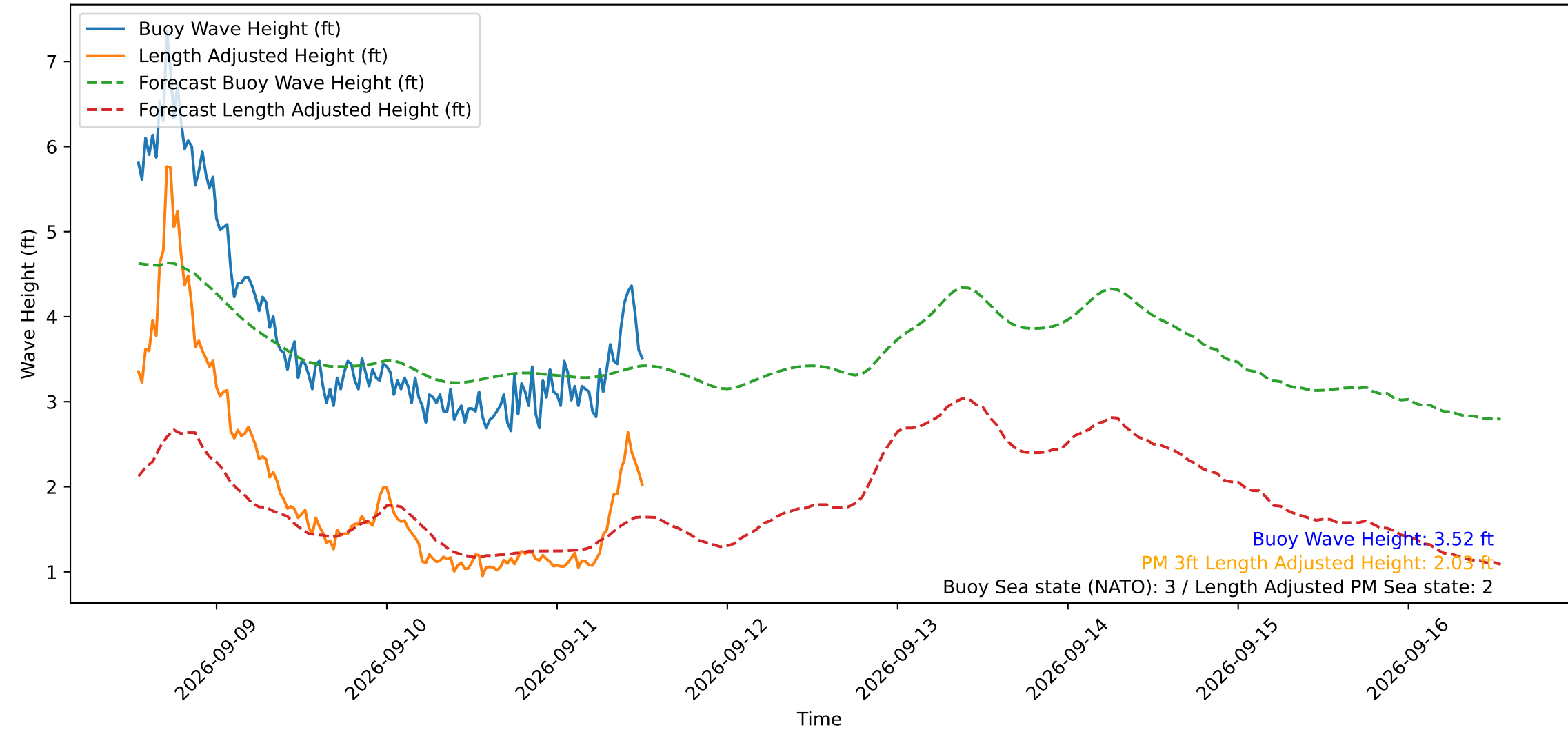
Wave Heights over Time for Oceanside Harbor at 2026-09-11 12:50:30
