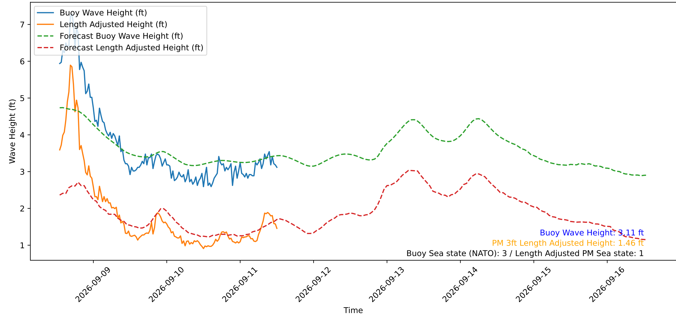
Wave Heights over Time for Green Beach at 2026-09-11 12:51:16
