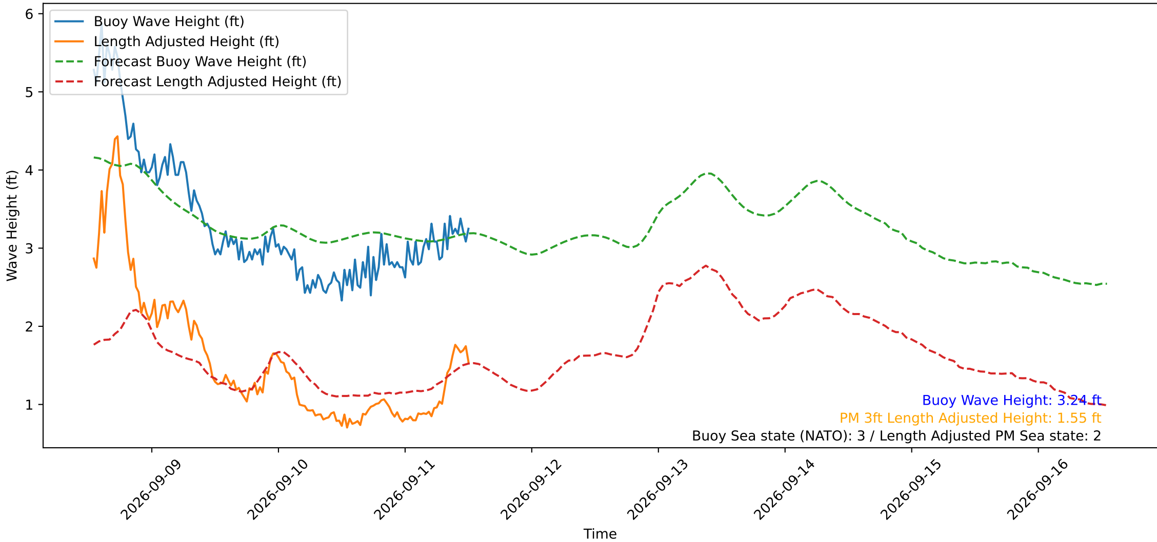
Wave Heights over Time for Red Beach at 2026-09-11 12:50:51
