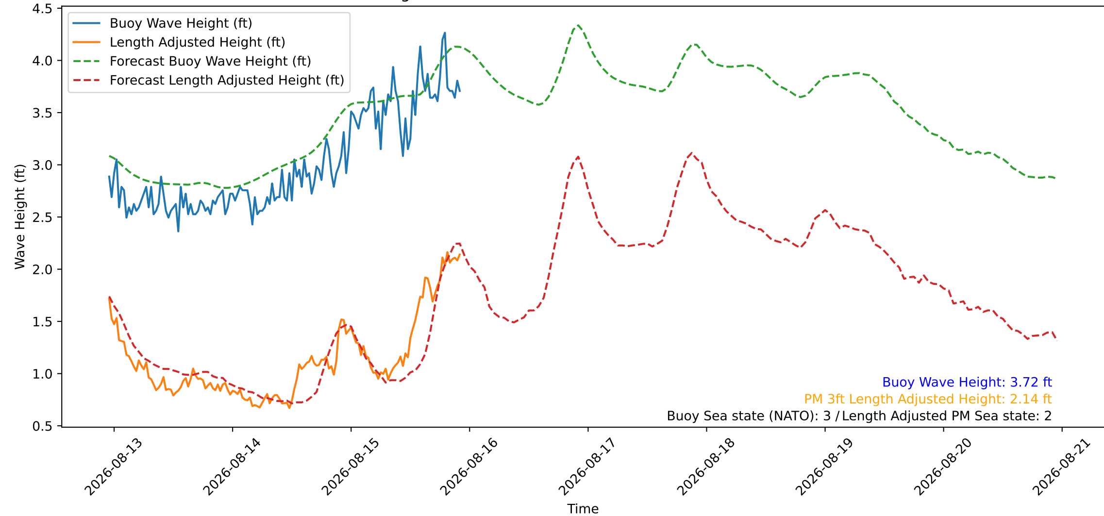
Wave Heights over Time for Green Beach at 2026-08-15 22:41:09
