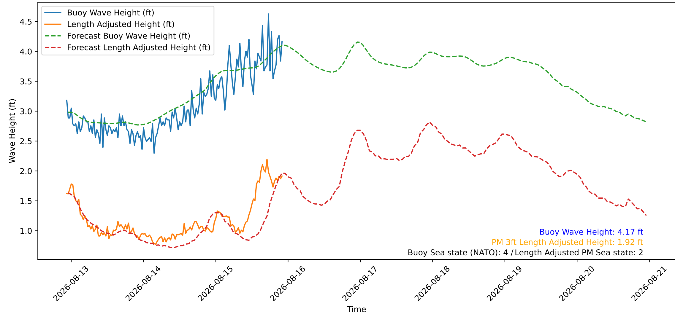
Wave Heights over Time for Oceanside Harbor at 2026-08-15 22:40:27
