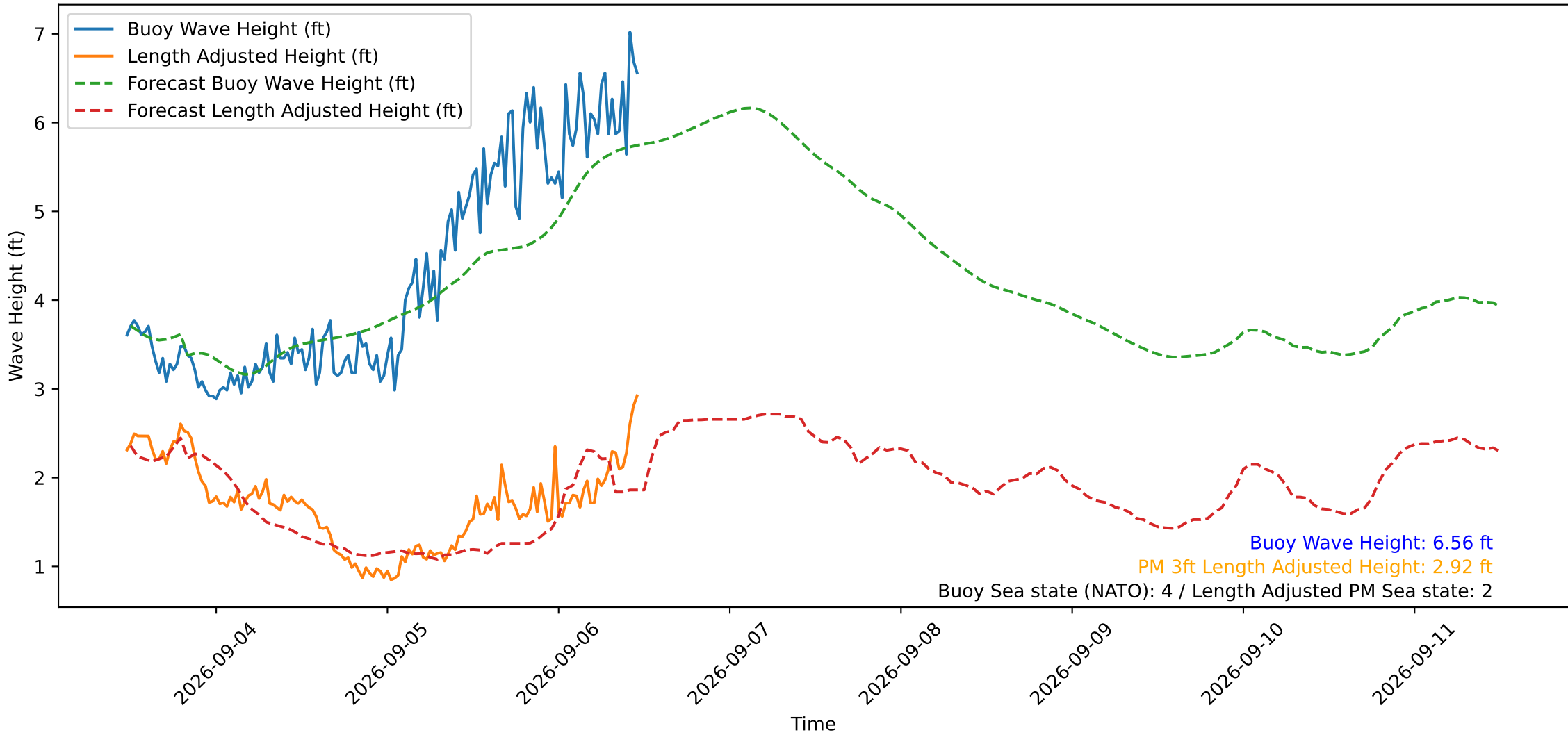
Wave Heights over Time for Oceanside Harbor at 2026-09-06 11:40:30
