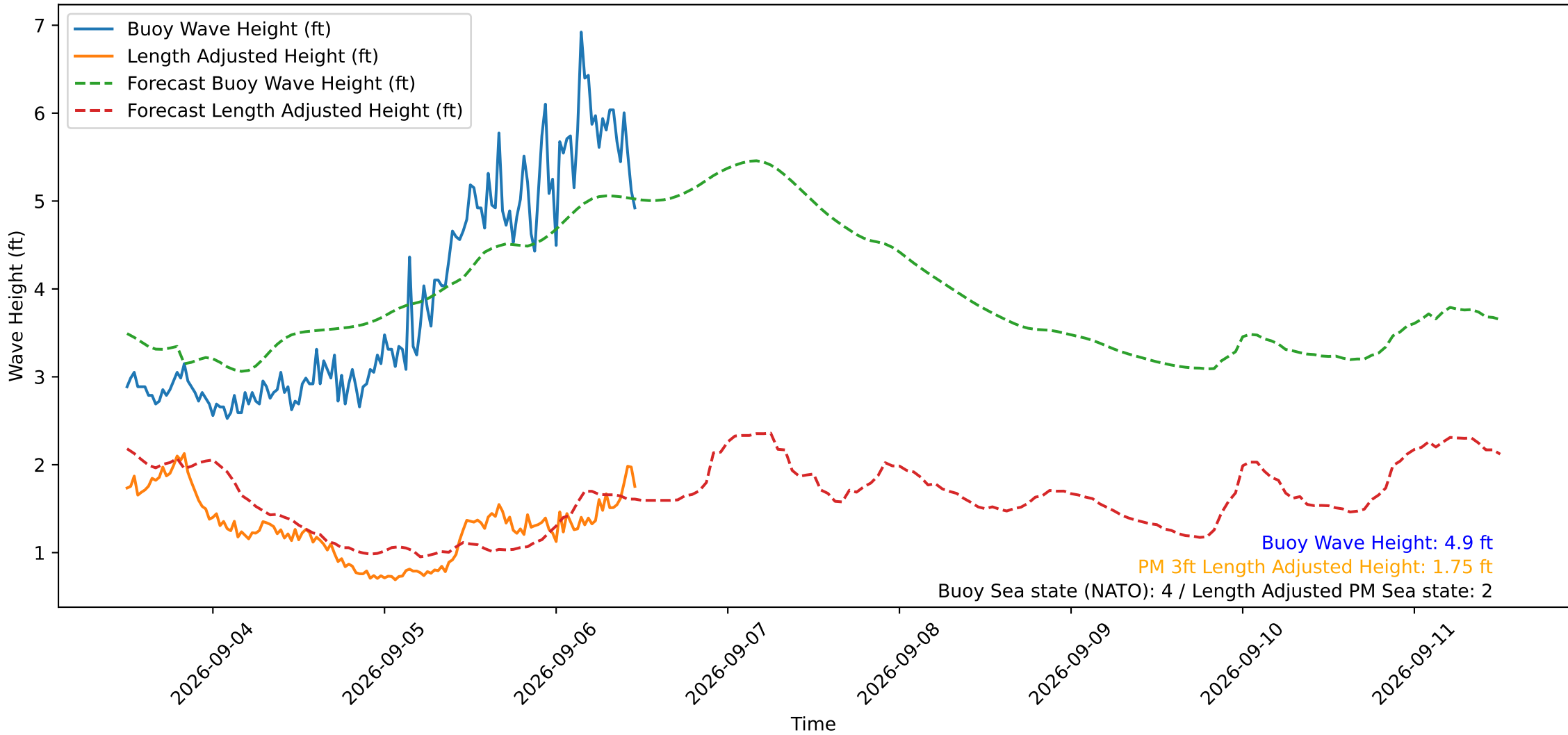
Wave Heights over Time for Red Beach at 2026-09-06 11:40:49
