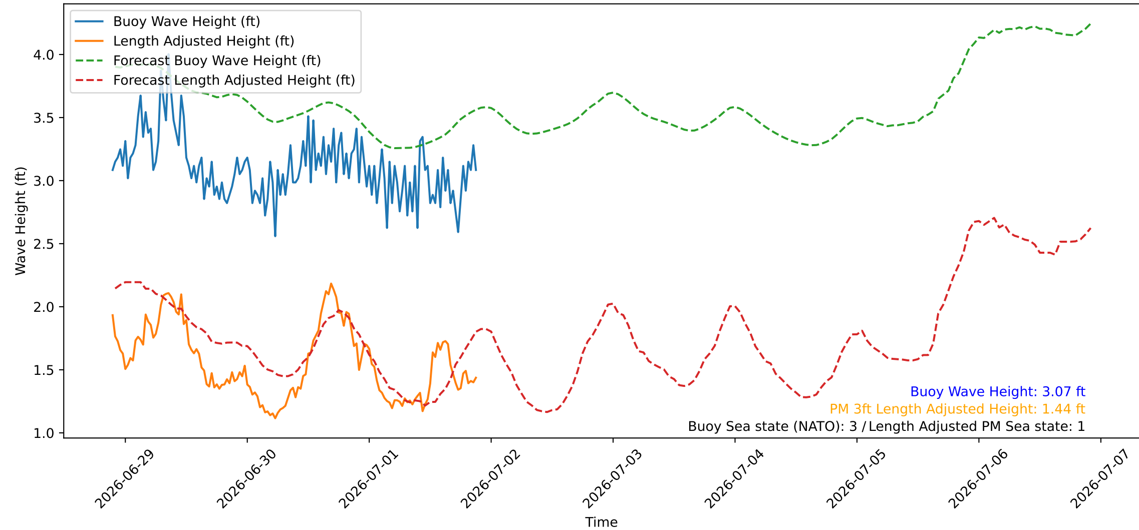
Wave Heights over Time for Oceanside Harbor at 2026-07-01 21:40:26
