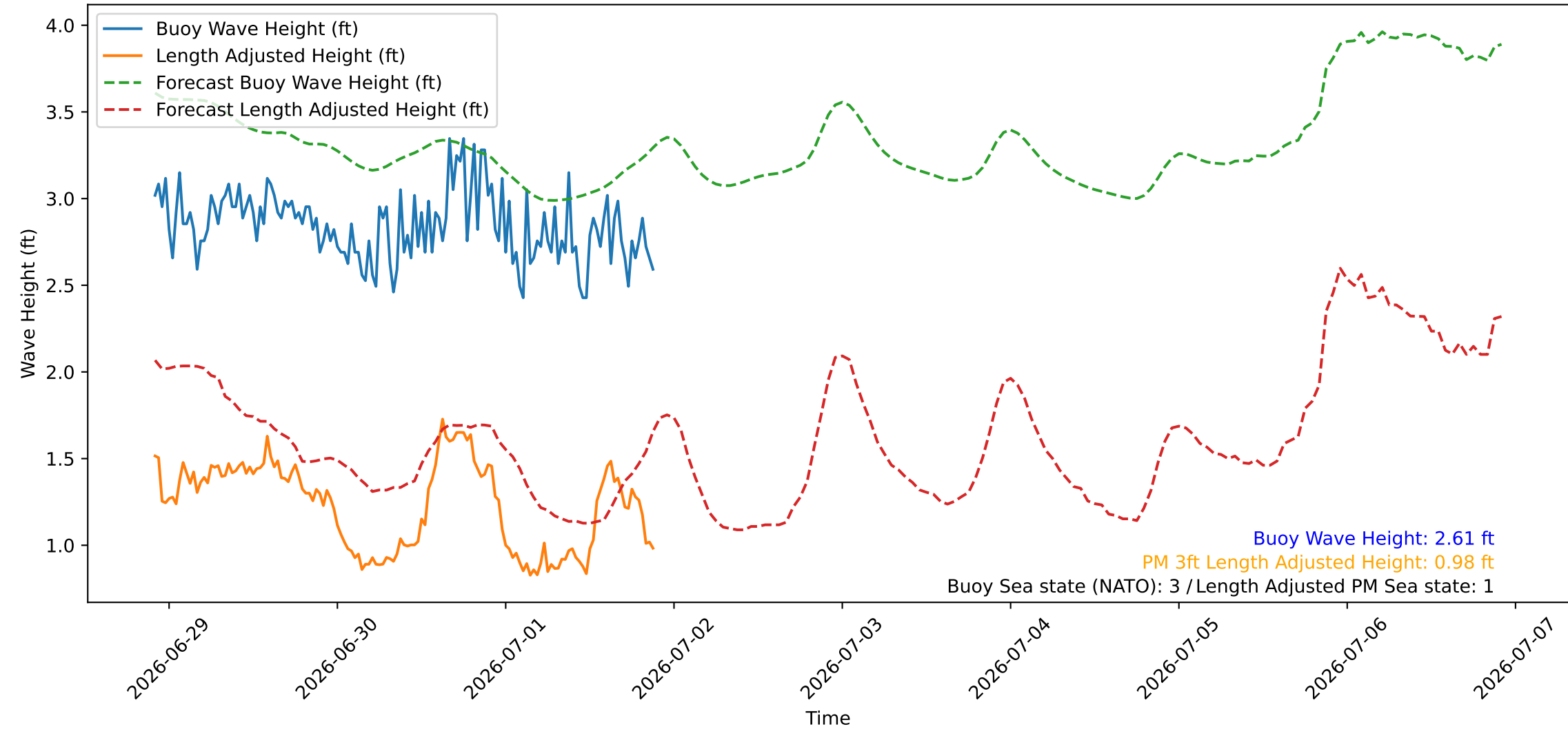
Wave Heights over Time for Red Beach at 2026-07-01 21:40:46
