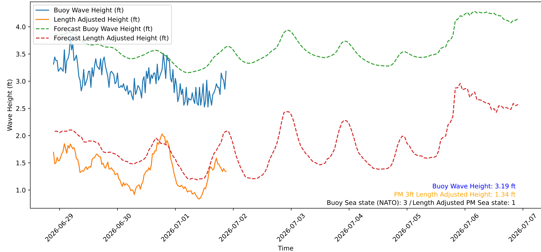
Wave Heights over Time for Green Beach at 2026-07-01 21:41:08
