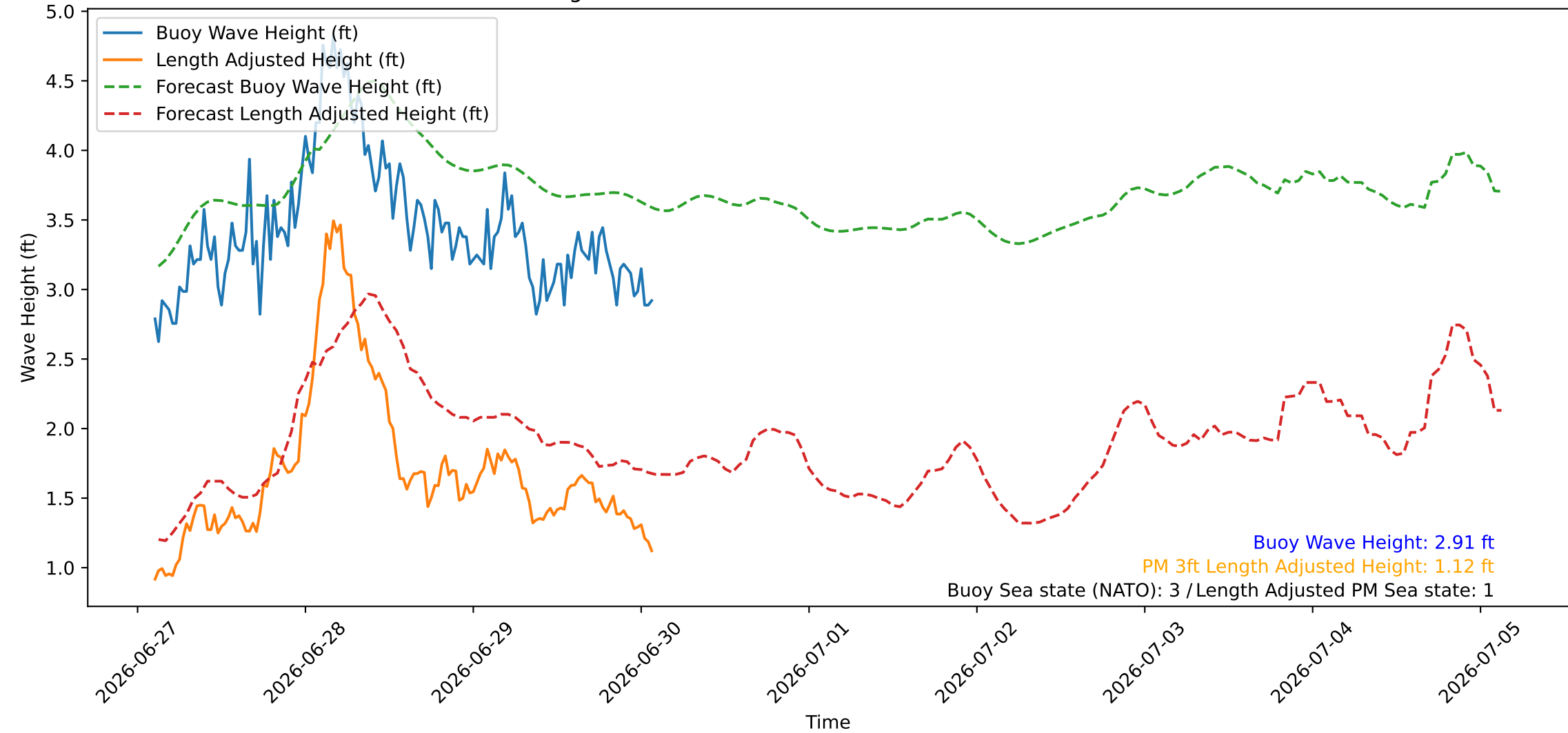
Wave Heights over Time for Green Beach at 2026-06-30 02:31:07
