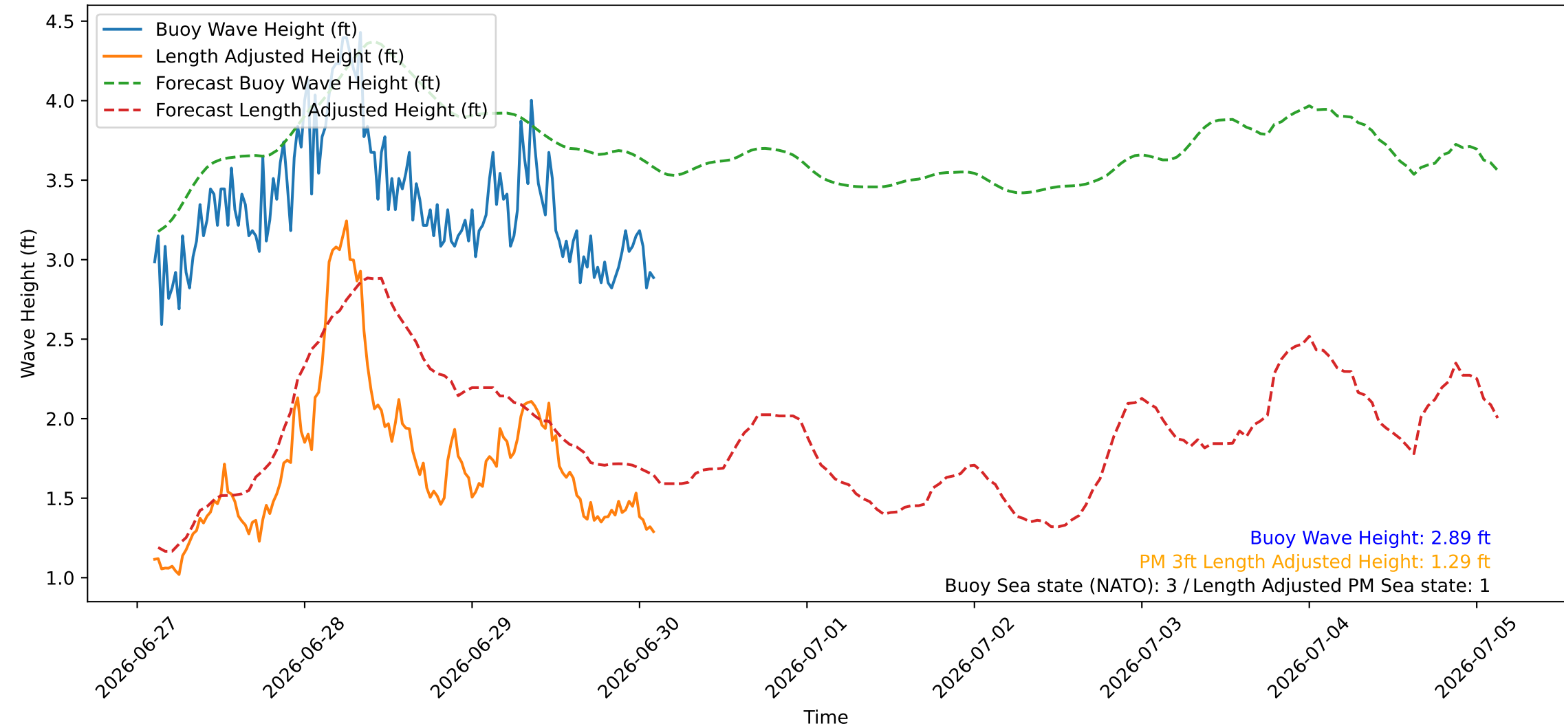
Wave Heights over Time for Oceanside Harbor at 2026-06-30 02:30:26
