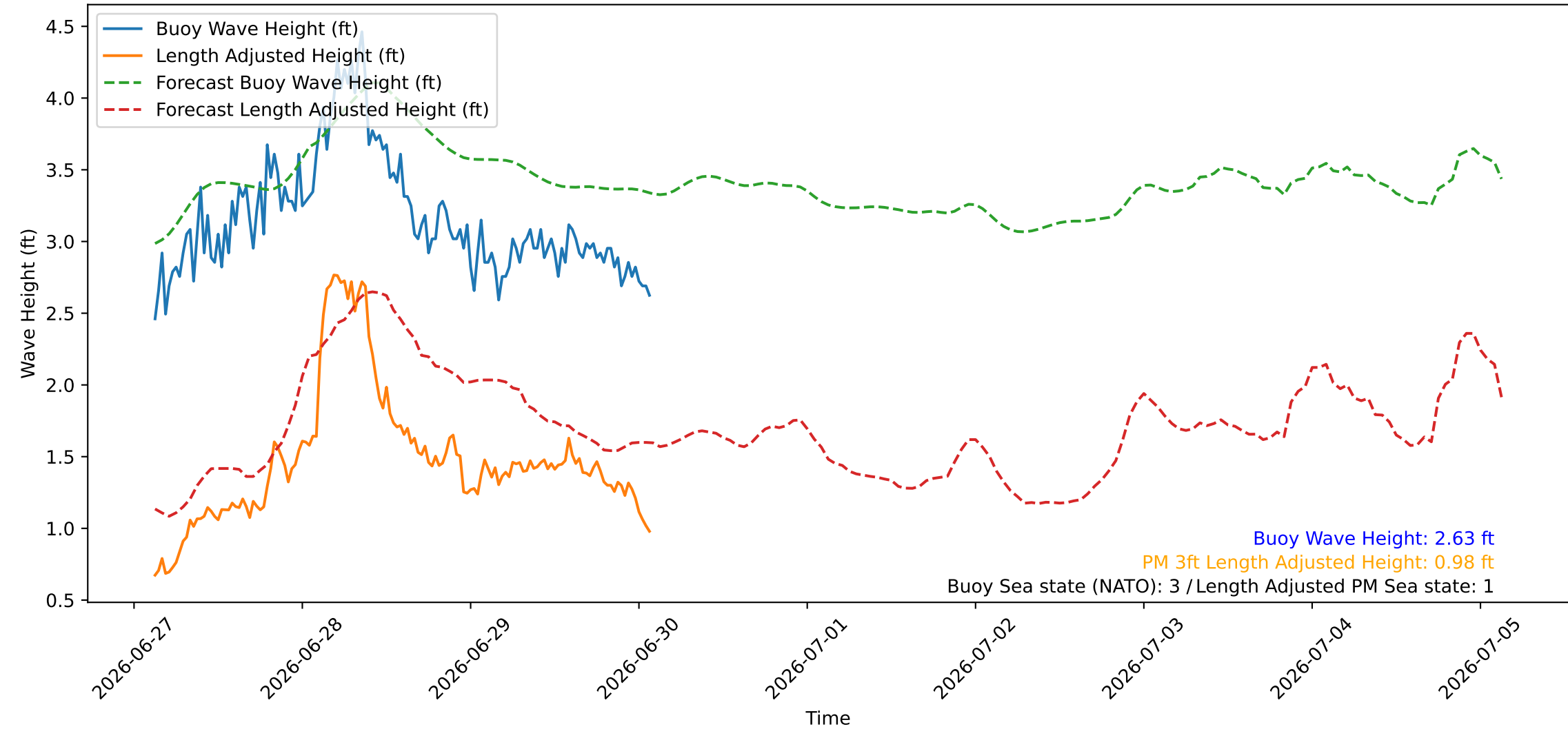
Wave Heights over Time for Red Beach at 2026-06-30 02:30:45
