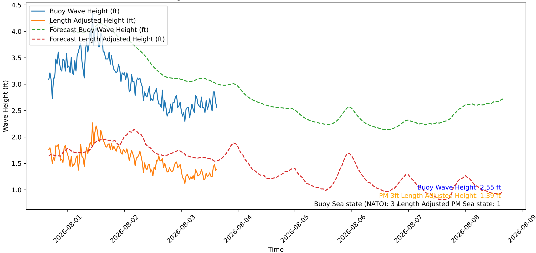
Wave Heights over Time for Oceanside Harbor at 2026-08-03 15:50:26
